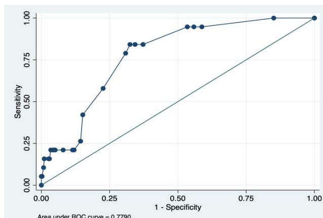
Figure 3 Post logistic regression ROC Curve
