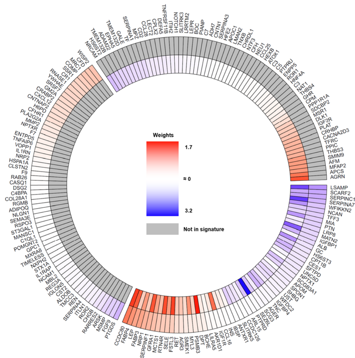
Figure 3. Proteins in the BMI-protein signature (outer circle) and WC-protein signature (inner circle). The colours represent the direction (red = increase, blue = decrease, grey = not in signature) while the intensity of the colours represents the magnitudes of the beta coefficients from elastic net regression. The bottom right segment represents the shared proteins between the BMI-protein and WC-protein signature. Moving anticlockwise, the top right segment represents proteins that are only in the WC-protein signature. Finally, the last segment on the top left represents proteins that are only in the BMI-protein signature. Text annotations are Entrez Gene symbols and the full protein names are provided in Supplementary Table 5. Abbreviations: BMI, body mass index; WC, waist circumference.
