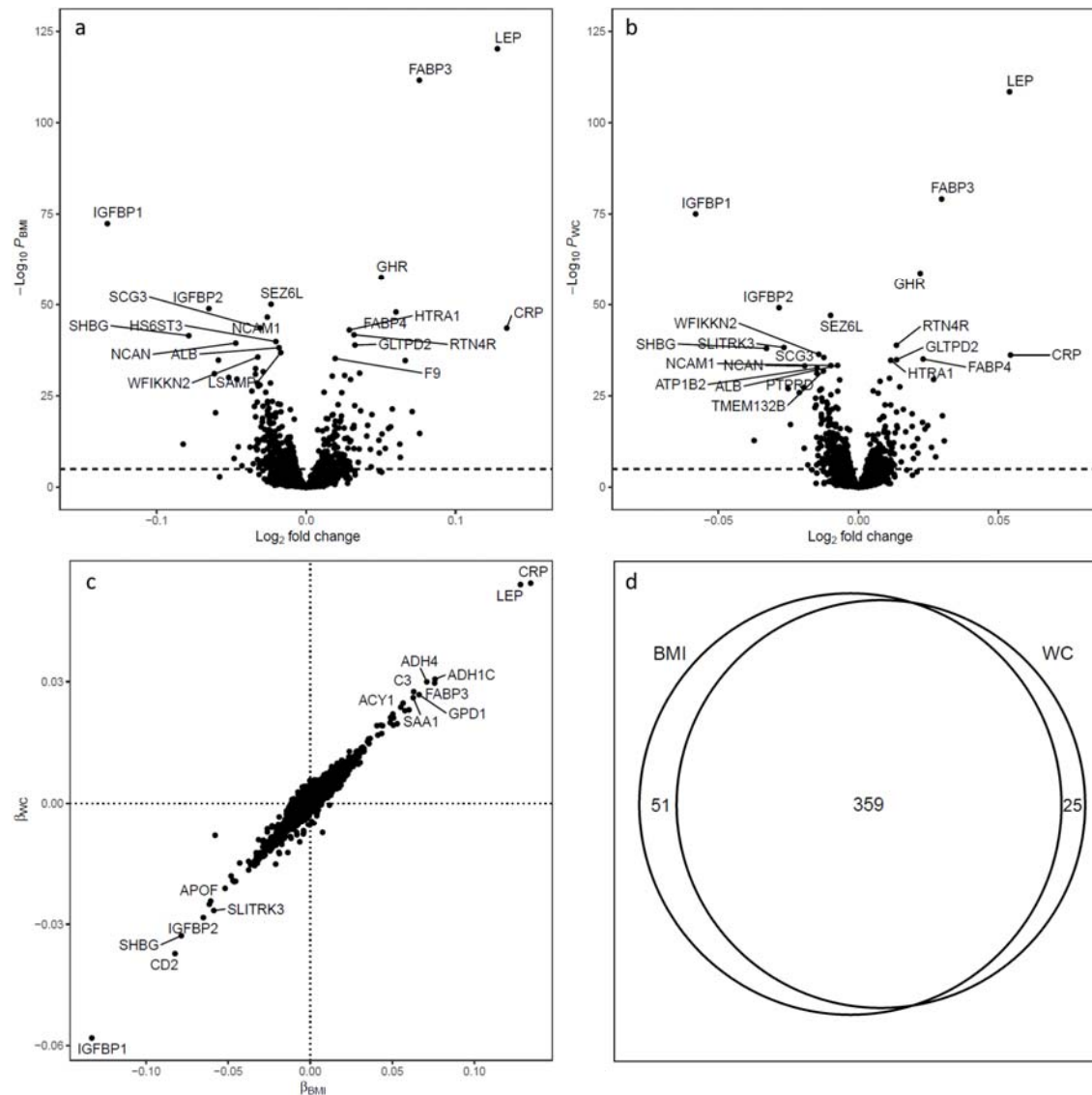
Figure 2. (a) Volcano-plot of -\log_{10}(P_{\text{BMI}}) against \log_2(\text{fold change}) per \text{kg}/\text{m}^2 increment of BMI. (b) Volcano-plot of -\log_{10}(P_{\text{WC}}) against \log_2(\text{fold change}) per cm increment of WC. Dashed lines represent the threshold for statistical significance after Bonferroni correction. (c) Scatterplot of the beta coefficients for WC against the beta coefficients for BMI. Text annotations are Entrez Gene symbols and the full protein names are provided in Supplementary Table 4. (d) Venn diagram of the number of proteins that were significantly associated with BMI and WC at the Bonferroni threshold. Abbreviations: BMI, body mass index; WC, waist circumference.
