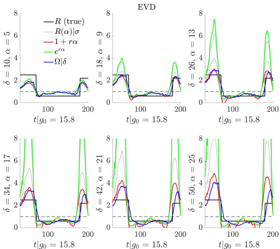
Figure S2: Relationships among transmissibility metrics for EVD. We explore threshold statistics computed using Eq. (S1) under structural assumptions from [2] and compare against the angular reproduction number \Omega (blue) at various window sizes of \alpha and \delta=2\alpha respectively. These EVD simulations are from Figure 3 of the main text with the true reproduction number (black) undergoing step dynamics. The threshold R(\alpha) statistics combine mean growth rate estimates from Figure S1 with \alpha , which serves as a proxy for the mean generation time under
