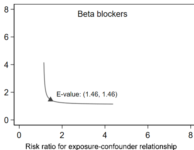
Figure 2. Sensitivity analysis examining the relationship between potential unaccounted confounders.
