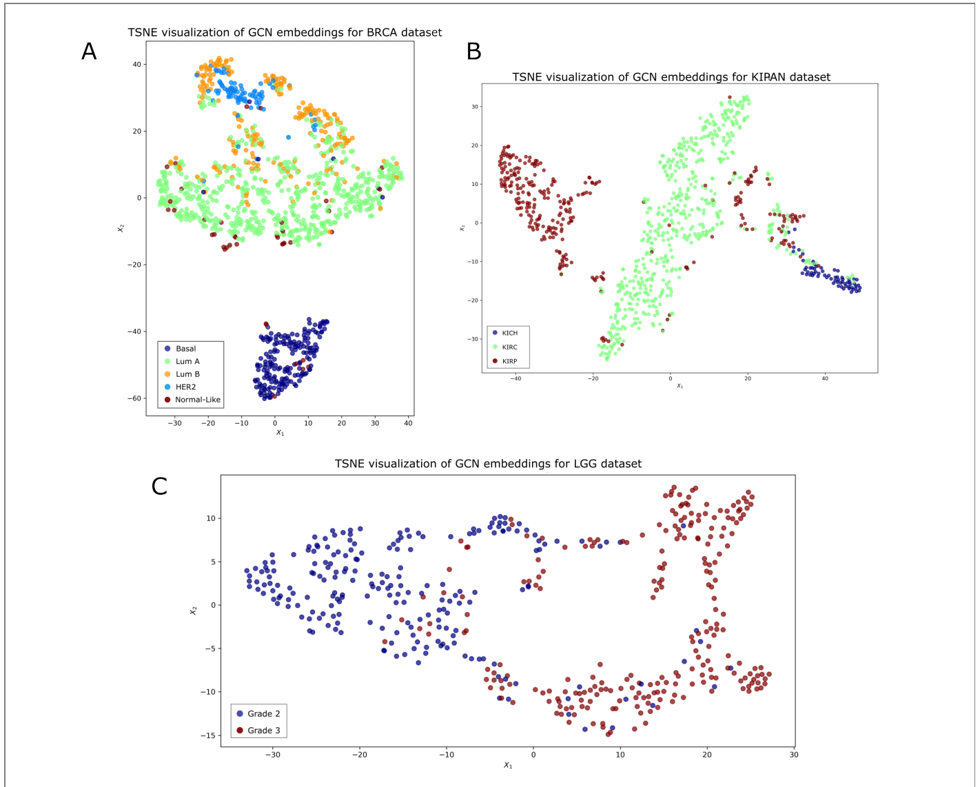
Figure S1. GCN TSNE Plots | The node embeddings learnt by the GCN model were visualised using TSNE plots. A shows the embeddings for the BRCA dataset, B for the KIPAN and C for the LGG datasets. These visualisations show the predictive power of the GCN and its ability to distinguish between classes.
