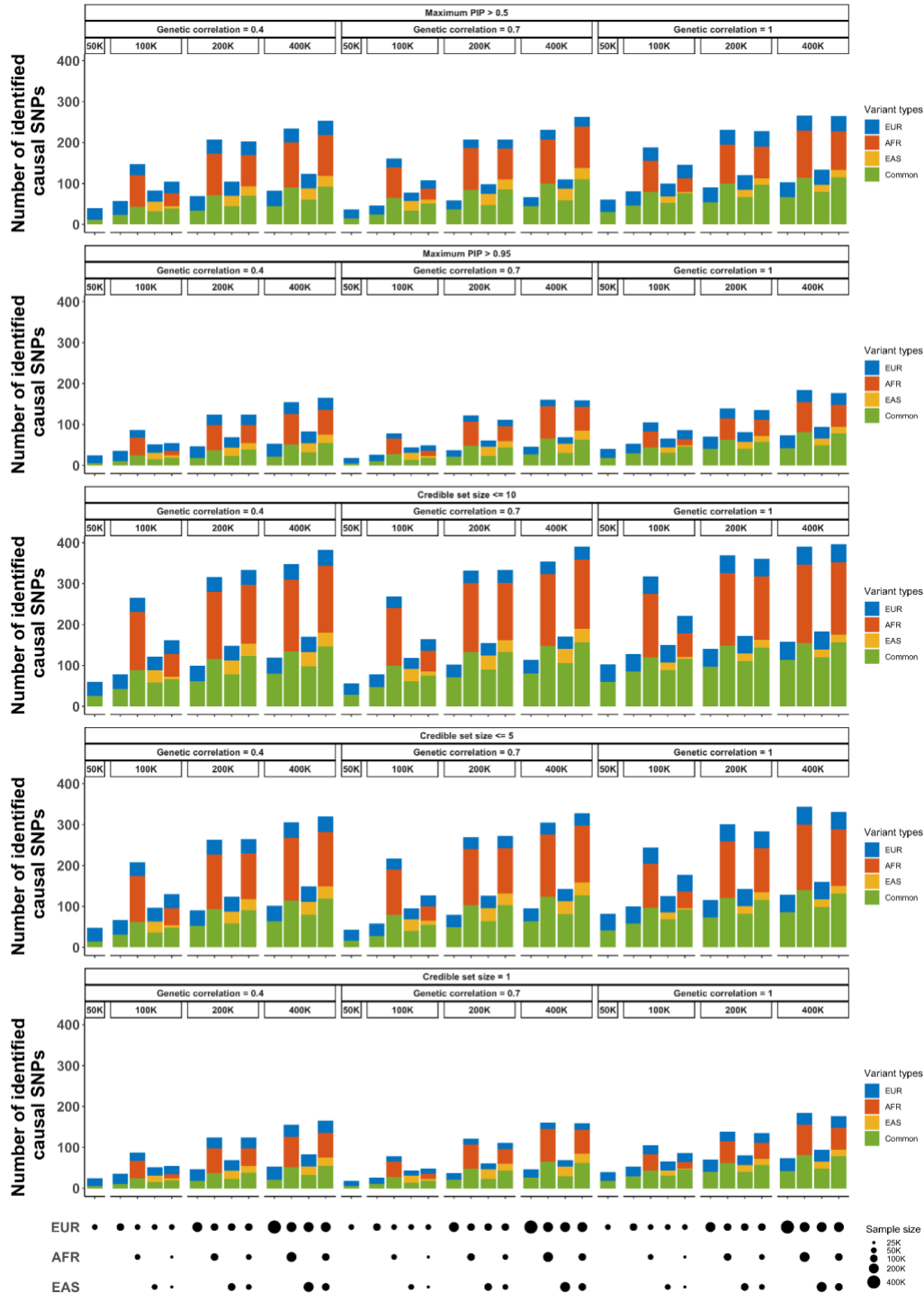
Supplementary Figure 14: The number of confidently identified causal SNPs under varying genetic correlations ( r_g ). The top label of each subpanel indicates the total sample size and the confidence level for the credible sets. The bottom panels indicate the sample size from each population. Numerical results are available in Supplementary Table 11.
