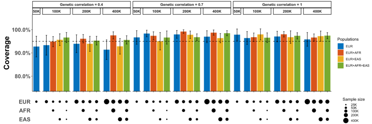
Supplementary Figure 11: The coverage of SuSiEx under varying genetic correlations ( r_g ). The dashed line represents the 95% coverage. The error bar represents the 95% confidence interval. The top label of each subpanel indicates the total sample size and the genetic correlation. The bottom panels indicate the sample size from each population. Numerical results are available in Supplementary Table 11.
