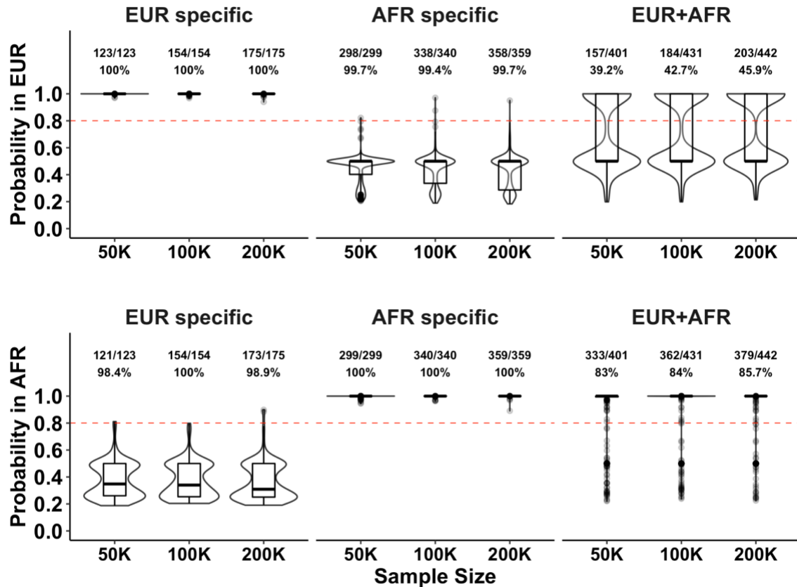
Supplementary Figure 29: The population-specific causal probability under the standard simulation setting. Analyses were conducted with a balanced EUR and AFR sample size. The x-axis shows the discovery sample size. The y-axis shows the population-specific causal probability of the identified credible set. The red dashed lines represent the probability of 0.8, which is used as a threshold to infer whether an identified credible set is causal in a population. The label at the top of each panel denotes the ground-truth causal configuration: “EUR specific” indicates that the variant is causal in the EUR population but not in the AFR population; “AFR specific” indicates that the variant is causal in the AFR population but not in the EUR population; “EUR+AFR” indicates that the variant is causal in both EUR and AFR populations. The fractional number on each panel represents “the number of credible sets with correct inference” among “the total number of credible sets identified by SuSiEx”. The percentage represents the accuracy of the inference. Numerical results are available in Supplementary Table 16.
