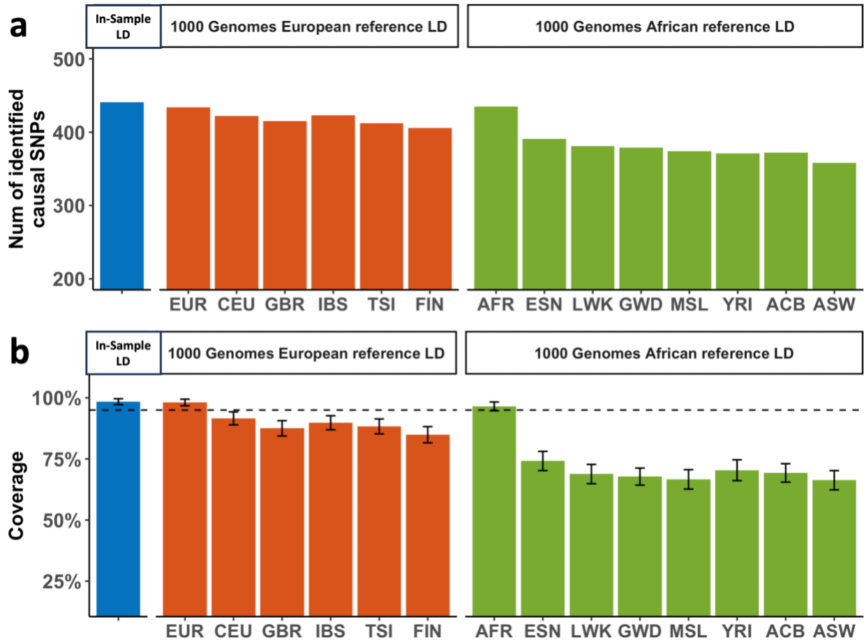
Supplementary Figure 39: Comparison of fine-mapping analyses between in-sample LD and external reference LD. Simulation was performed using the standard simulation setting with 200K EUR and 200K AFR samples. a , The number of identified true causal variants (true causal variants covered by a credible set). b , The coverage of credible sets. The dashed line indicates 95% coverage. The error bar indicates the 95% confidence interval. The top label of each subpanel indicates the reference panel used in the analysis. In-sample LD indicates that in-sample LD was used for both EUR and AFR samples. 1000 Genomes European reference LD indicates that reference LD from 1000 Genomes EUR subpopulations (CEU, GBR, IBS, TSI, FIN) was used for EUR samples but in-sample LD was used for AFR samples. 1000 Genomes African reference LD indicates that reference LD from 1000 Genomes AFR subpopulations (ESN, LWK, GWD, MSL, YRI, ACB, ASW) was used for AFR samples but in-sample LD was used for EUR samples. Numerical results are available in Supplementary Table 18.
