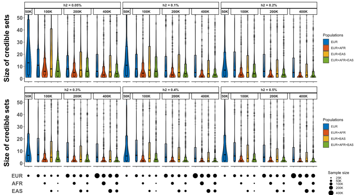
Supplementary Figure 17: The size of credible sets identified by SuSiEx under varying local heritability ( h^2 ). The upper and lower bounds of the box indicate the 75th and 25th percentiles, respectively. The middle line in the box indicates the median. The top label of each subpanel indicates the total sample size and the local heritability. The bottom panels indicate the sample size from each population. Numerical results are available in Supplementary Table 12.
