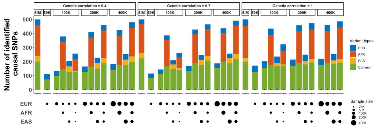
Supplementary Figure 10: The number of causal SNPs identified by SuSiEx under varying genetic correlations ( r_g ). The top label of each subpanel indicates the total sample size and the genetic correlation. The bottom panels indicate the sample size from each population. Numerical results are available in Supplementary Table 11.
