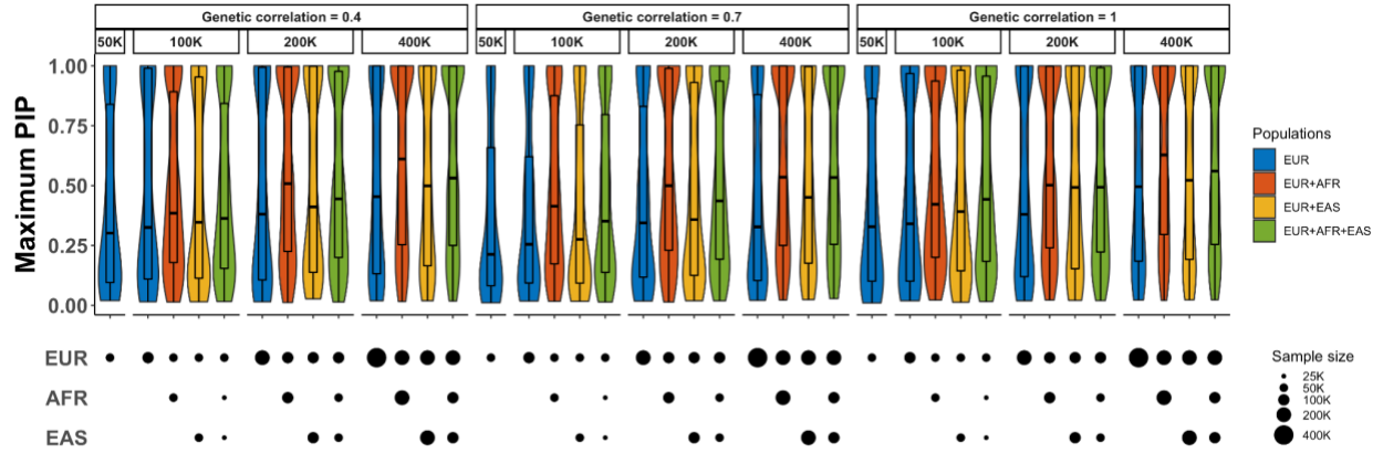
Supplementary Figure 13: The maximum PIP estimated by SuSiEx under varying genetic correlations ( r_g ). The upper and lower bounds of the box indicate the 75th and 25th percentiles, respectively. The middle line in the box indicates the median. The top label of each subpanel indicates the total sample size and the genetic correlation. The bottom panels indicate the sample size from each population. Numerical results are available in Supplementary Table 11.
