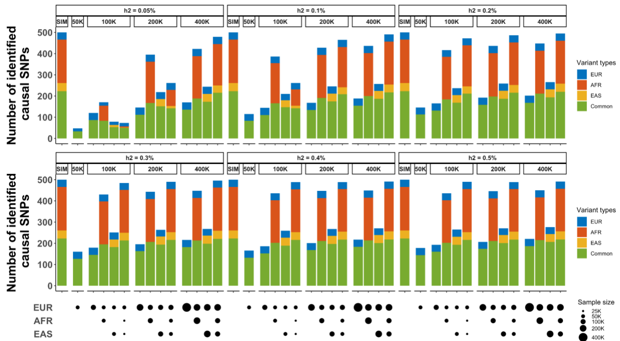
Supplementary Figure 15: The number of causal SNPs identified by SuSiEx under varying local heritability ( h^2 ). The top label of each subpanel indicates the total sample size and the local heritability. The bottom panels indicate the sample size from each population. Numerical results are available in Supplementary Table 12.
