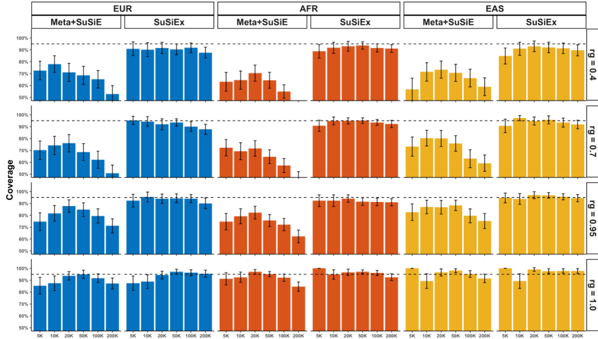
Supplementary Figure 4: The coverage of Meta+SuSiE and SuSiEx when analyzing genetically close populations. The top label of each subpanel indicates the continental population in which the analysis was performed and the fine-mapping method. The label on the right indicates the genetic correlation between the two subpopulations. The x-axis shows the discovery sample size of each subpopulation. The y-axis shows the coverage. The dashed line represents the 95% coverage. The error bar represents the 95% confidence interval. Numerical results are available in Supplementary Table 6.
