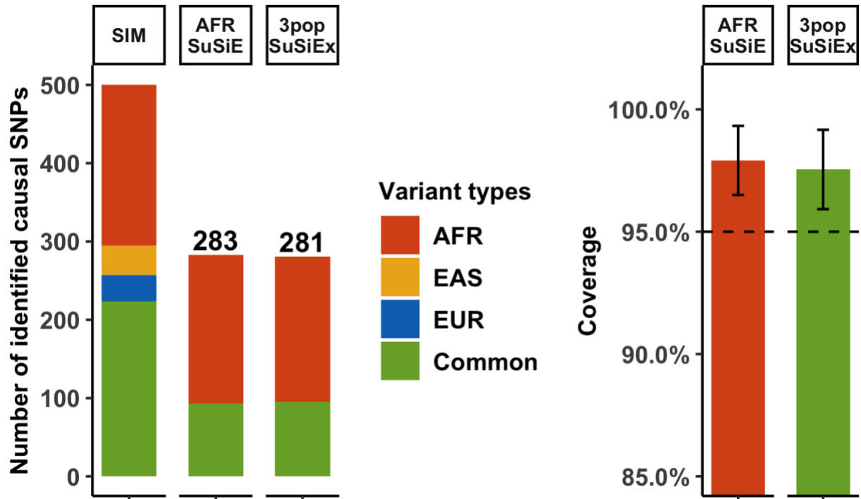
Supplementary Figure 28: Performance of SuSiEx in the presence of African-specific causal variants. Left: The number of identified true causal variants when using single-population SuSiE in the AFR population vs. using cross-population SuSiEx that integrates data from the three populations. Right: The coverage of credible sets. The dashed line represents 95% coverage. The error bar represents the 95% confidence interval. Numerical results are available in Supplementary Table 15.
