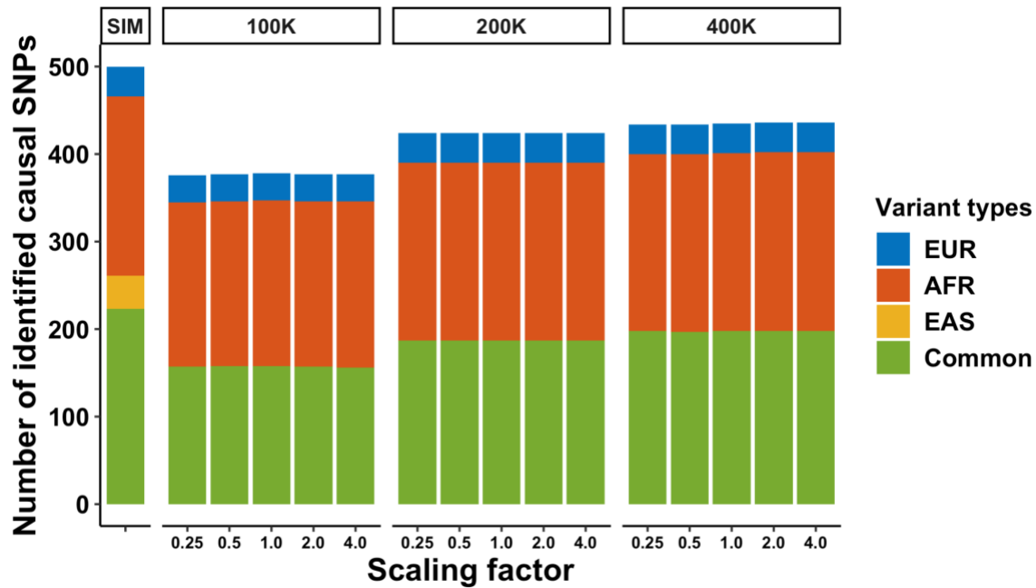
Supplementary Figure 25: The impact of different \tau_s^2 values on the performance of SuSiEx. The top label on each subpanel indicates the discovery sample size of each population. The x-axis shows the factor by which the \tau_s^2 parameter is scaled. The y-axis shows the number of identified true causal variants. Simulations were conducted under the standard parameter setting with a balanced EUR and AFR sample size. The total sample size is shown above each panel. Numerical results are available in Supplementary Table 14.
