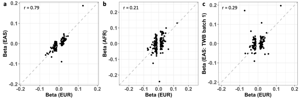
Supplementary Figure 41: The marginal per-allele effect size of the maximum PIP variant across populations. We included variants in single-credible-set loci with PIP >95% estimated by SuSiEx and minor allele frequencies >5% in all populations. a , EUR vs. EAS; b , EUR vs. AFR; c , EUR vs. EAS (TWB batch 1).
