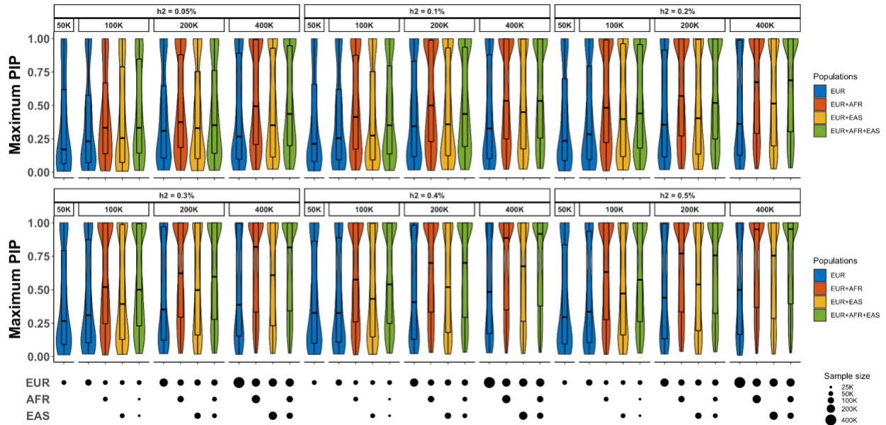
Supplementary Figure 18: The maximum PIP estimated by SuSiEx under varying local heritability ( h^2 ). The upper and lower bounds of the box indicate the 75th and 25th percentiles, respectively. The middle line in the box indicates the median. The top label of each subpanel indicates the total sample size and the local heritability. The bottom panels indicate the sample size from each population. Numerical results are available in Supplementary Table 12.
