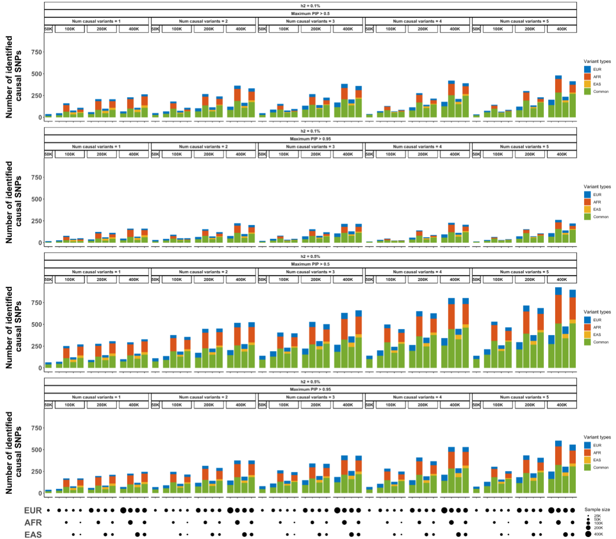
Supplementary Figure 24: The number of confidently identified causal SNPs under varying numbers of causal SNPs per locus ( n_{csi} ). The top label of each subpanel indicates the total sample size and the confidence level for the credible sets. The bottom panels indicate the sample size from each population. Numerical results are available in Supplementary Table 13.
