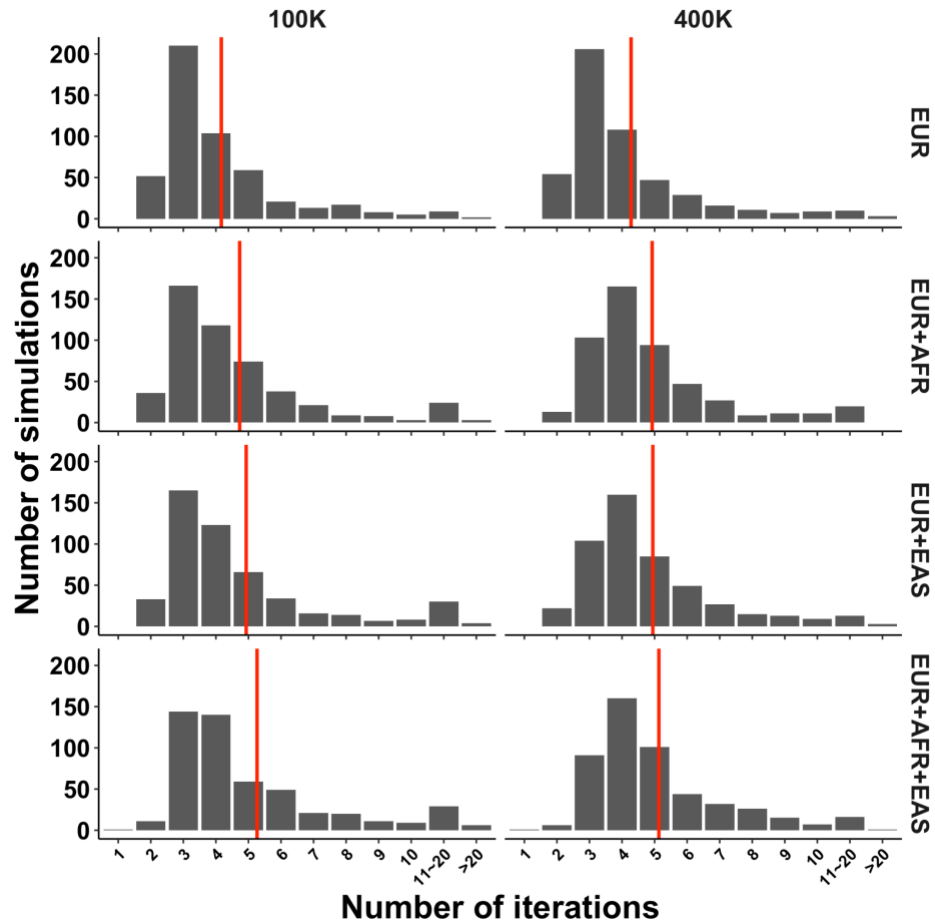
Supplementary Figure 9: The number of iterations before SuSiEx converged under varying sample sizes and population combinations. The histograms show the distributions of the number of iterations before SuSiEx converged. The red vertical line represents the average number of iterations. All analyses were conducted under the standard simulation settings. The total sample size is displayed at the top of each subpanel. The combinations of 'EUR+AFR' and 'EUR+EAS' were analyzed with a balanced sample size, while 'EUR+AFR+EAS' was analyzed with a sample size ratio of EUR:AFR:EAS = 2:1:1. Numerical results are available in Supplementary Table 8.
