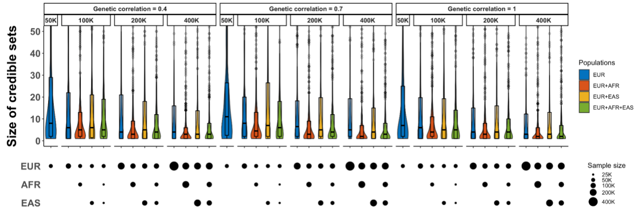
Supplementary Figure 12: The size of credible sets identified by SuSiEx under varying genetic correlations ( r_g ). The upper and lower bounds of the box indicate the 75th and 25th percentiles, respectively. The middle line in the box indicates the median. The top label of each subpanel indicates the total sample size and the genetic correlation. The bottom panels indicate the sample size from each population. Numerical results are available in Supplementary Table 11.
