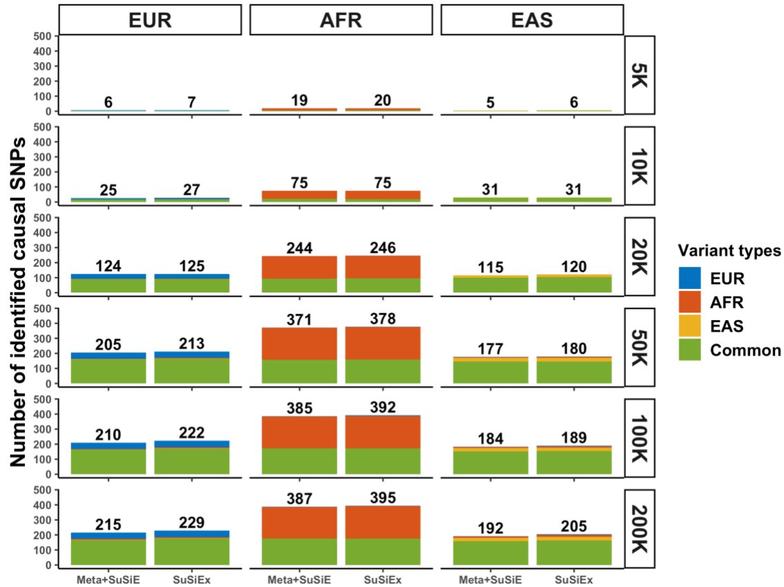
Supplementary Figure 5: The number of causal variants identified by Meta+SuSiE and SuSiEx when analyzing genetically close populations with identical causal effect sizes. The top label on each subpanel indicates the continental population in which the analysis was performed. The label on the right indicates the discovery sample size of each subpopulation. The x-axis shows the fine-mapping method. The y-axis shows the number of identified true causal variants. Numerical results are available in Supplementary Table 6.
