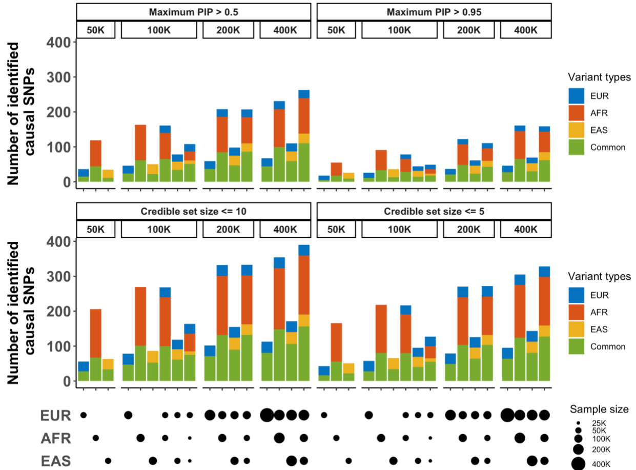
Supplementary Figure 2: The number of confidently identified causal SNPs under the standard simulation setting. The top label of each subpanel indicates the total sample size and the thresholds for selecting the credible sets. The bottom panels indicate the sample size from each population. Numerical results are available in Supplementary Table 4.
