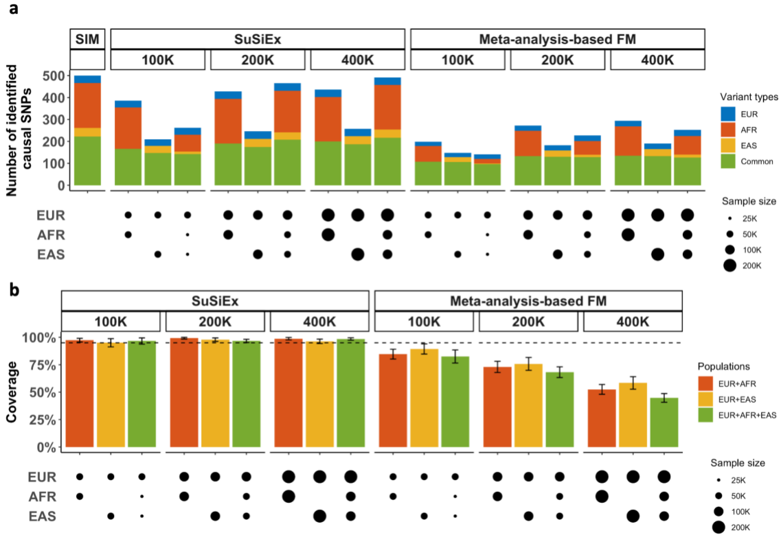
Supplementary Figure 3: Comparison between SuSiEx and the meta-analysis-based fine-mapping method using the standard simulation setting. a , The number of identified true causal variants (true causal variants covered by a credible set). b , The coverage of credible sets. The dashed line represents the 95% coverage. The error bar represents the 95% confidence interval. The top label of each subpanel indicates the total sample size and the fine-mapping method. The bottom panels indicate the sample size from each population. Numerical results are available in Supplementary Table 5.
