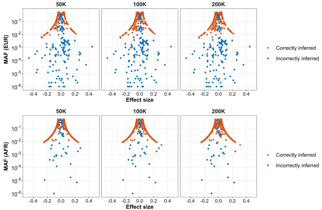
Supplementary Figure 30: The impact of allele frequency and causal effect size on the classification of population-specific causal variants. This plot corresponds to the simulation under the “EUR+AFR” scenario in Supplementary Figure 29. The x-axis shows the simulated effect sizes of the causal variants. The y-axis shows the minor allele frequencies (MAF) of the causal variants in a specific population. The label above each panel indicates the discovery sample size. Red dots represent variants that are correctly inferred to be causal in the population. Blue dots represent variants that are incorrectly inferred to be not causal in the population. Incorrectly inferred variants tend to have low MAF or small effect sizes. Numerical results are available in Supplementary Table 16.
