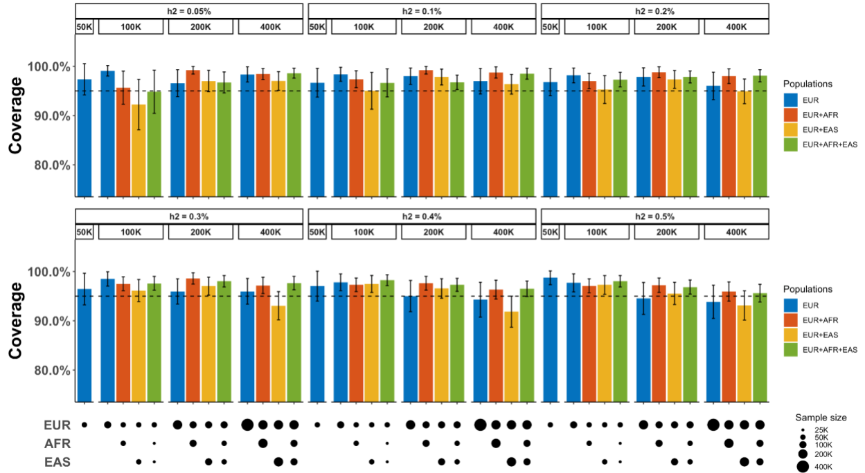
Supplementary Figure 16: The coverage of SuSiEx under varying local heritability ( h^2 ). The dashed line represents the 95% coverage. The error bar represents the 95% confidence interval. The top label of each subpanel indicates the total sample size and the local heritability. The bottom panels indicate the sample size from each population. Numerical results are available in Supplementary Table 12.
