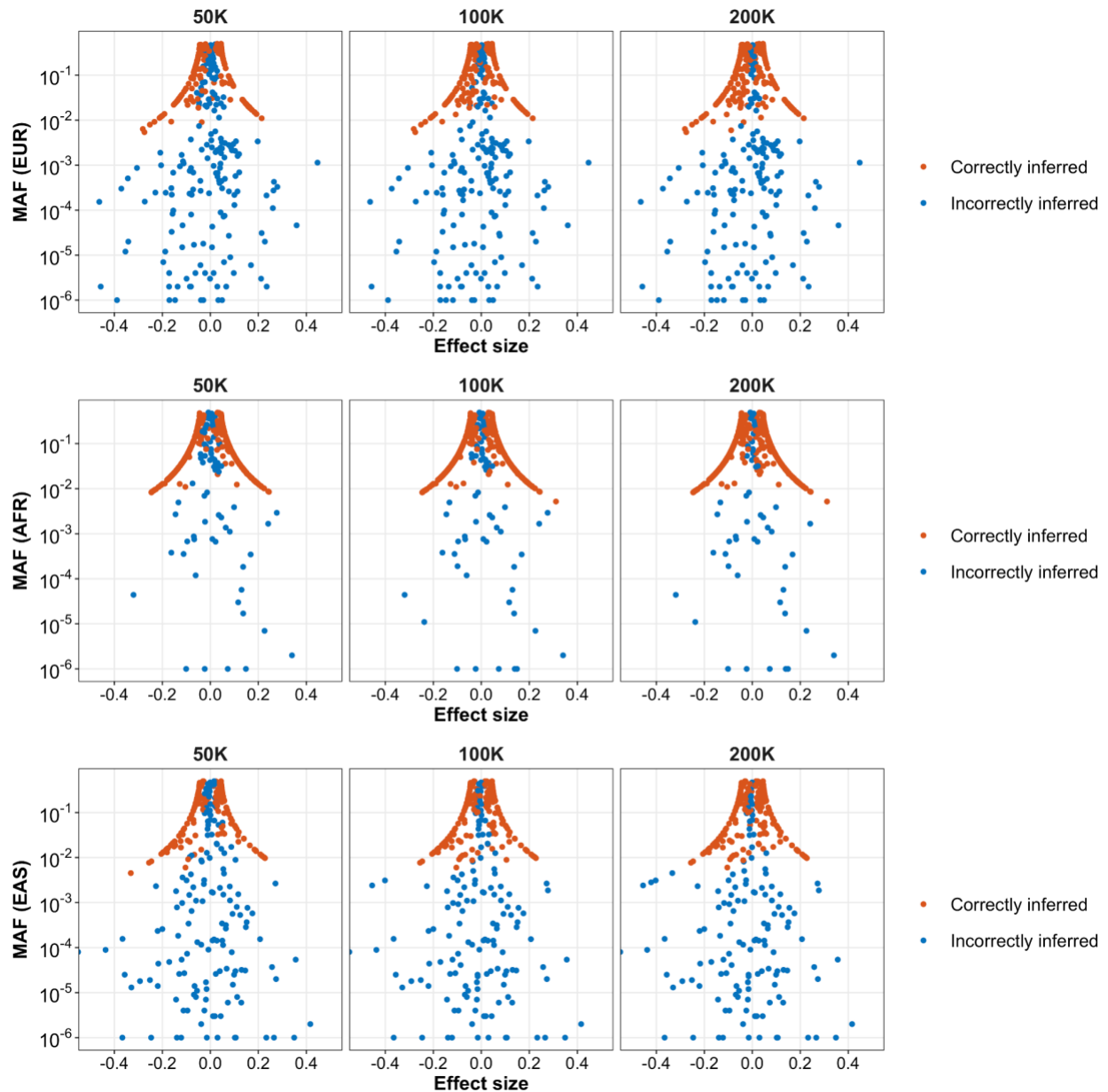
Supplementary Figure 35: The impact of allele frequency and causal effect size on the classification of population-specific causal variants in three-population fine-mapping analysis. This plot corresponds to the simulation under the “EUR+AFR+EAS” scenario in Supplementary Figure 34. The x-axis shows the simulated effect sizes of the causal variants. The y-axis shows the minor allele frequencies (MAF) of the causal variants in a specific population. The label above each panel indicates the discovery sample size. Red dots represent variants that are correctly inferred to be causal in the population. Blue dots represent variants that are incorrectly inferred to be not causal in the population. Incorrectly inferred variants tend to have low MAF or small effect sizes. Numerical results are available in Supplementary Table 17.
