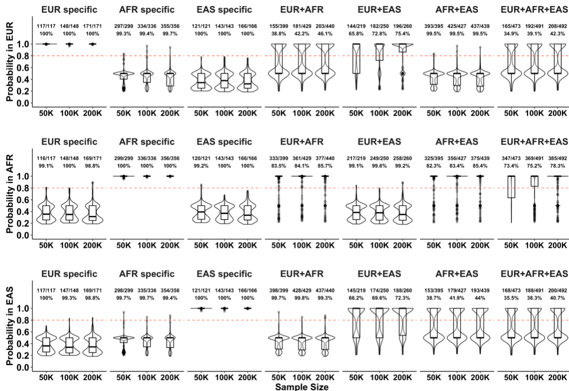
Supplementary Figure 34: The population-specific causal probability under the standard simulation setting in three-population fine-mapping analysis. Analyses were conducted with a balanced EUR, AFR and EAS sample size. The x-axis shows the discovery sample size. The y-axis shows the population-specific causal probability of the identified credible set. The red dashed lines denote the probability of 0.8, which is used as a threshold to infer whether an identified credible set is causal in a population. The label at the top of each panel denotes the ground-truth causal configuration: “EUR specific” indicates that the variant is causal in the EUR population but not in the AFR and EAS populations; “AFR specific” indicates that the variant is causal in the AFR population but not in the EUR and EAS populations; “EAS specific” indicates that the variant is causal in the EAS population but not in the EUR and AFR populations; “EUR+AFR+EAS” indicates that the variant is causal in EUR, AFR and EAS populations. The fractional number on each panel represents “the number of credible sets with correct inference” among “the total number of credible sets identified by SuSiEx”. The percentage represents the accuracy of the inference. Numerical results are available in Supplementary Table 17.
