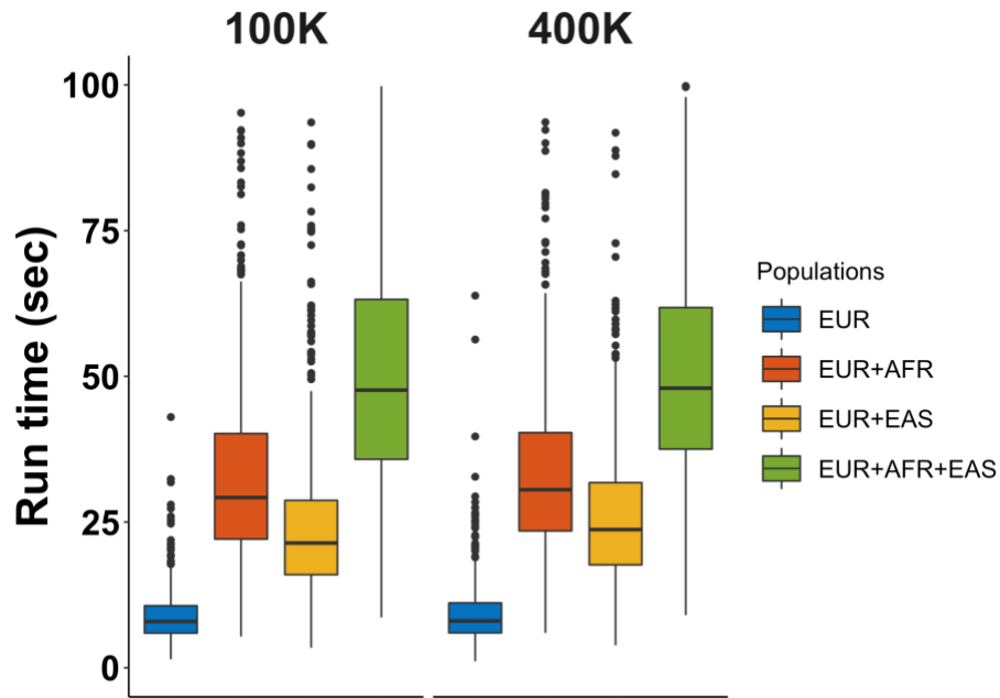
Supplementary Figure 8: The runtime of SuSiEx under varying sample sizes and population combinations. The y-axis shows the runtime of SuSiEx, measured in seconds, using a single CPU. Different colors indicate different population combinations. All analyses were conducted under the standard simulation settings. The total sample size is displayed at the top of each subpanel. The combinations of 'EUR+AFR' and 'EUR+EAS' were analyzed with a balanced sample size, while 'EUR+AFR+EAS' was analyzed with a sample size ratio of EUR:AFR:EAS = 2:1:1. Numerical results are available in Supplementary Table 8.
