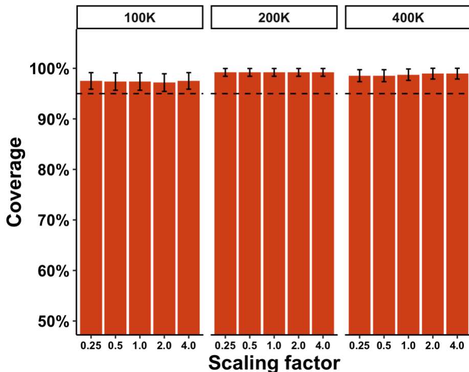
Supplementary Figure 26: The impact of different \tau_s^2 values on the calibration of SuSiEx. The top label on each subpanel indicates the discovery sample size of each population. The x-axis shows the factor by which the \tau_s^2 parameter is scaled. The y-axis shows the coverage. The dashed line represents 95% coverage. The error bar represents the 95% confidence interval. Simulations were conducted under the standard parameter setting with a balanced EUR and AFR sample size. The total sample size is shown above each panel. Numerical results are available in Supplementary Table 14.
