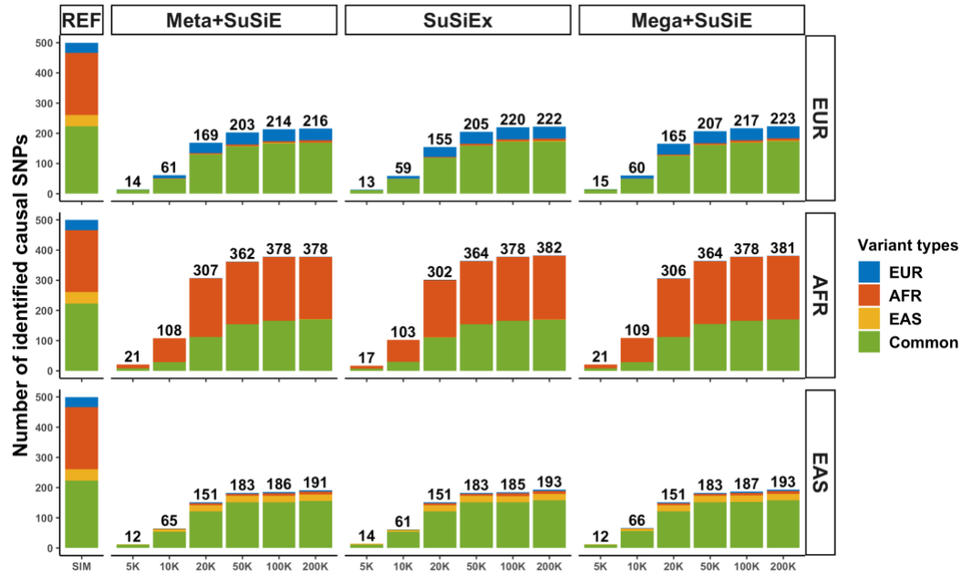
Supplementary Figure 6: The number of causal variants identified by Meta+SuSiE, SuSiEx and Mega+SuSiE when analyzing two independent samples from the same population. The top label on each subpanel indicates the fine-mapping method. The label on the right indicates the continental population in which analysis was performed. The x-axis shows the discovery sample size. The y-axis shows the number of identified true causal variants. The approach that performs GWAS on the merged dataset and applies SuSiE to the resulting GWAS is denoted as Mega+SuSiE. Numerical results are available in Supplementary Table 7.
