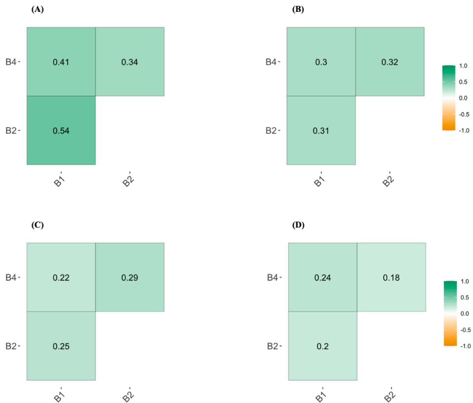
Figure S2. Correlations of measured PM 2.5 (A and B) and CO (C and D) exposures by study visit for control (A and C) and intervention households (B and D). B1 indicates visits at <3m, B2 indicates visits at ~6m, and B4 indicates visits at approximately 12m.
