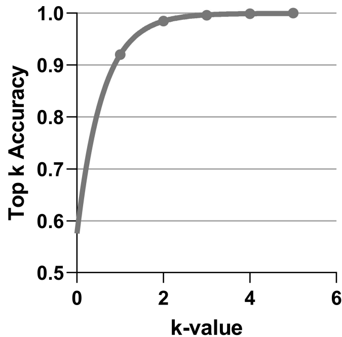
Figure 14: Top K Accuracy
