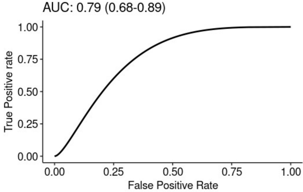
Figure 2: Receiver operator curve (ROC) at 5-years of the International IgAN risk prediction tool in the study population.
