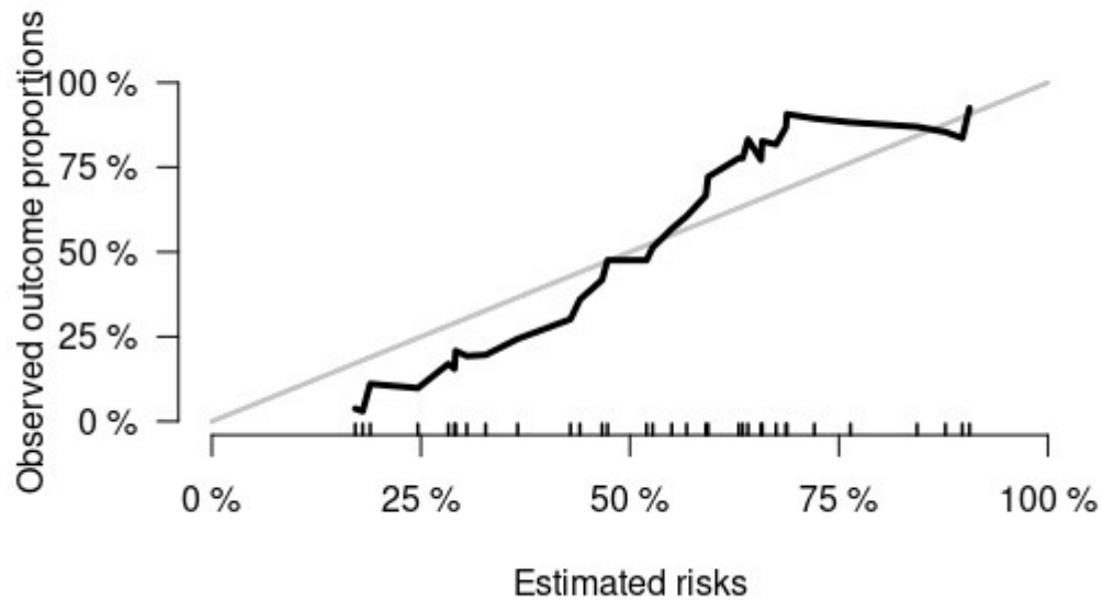
Figure 3: Calibration curve (Estimated risks plotted against Observed risk) at 5 years of the International IgAN risk prediction equation in the study population. Values below and above the 45 degrees line signify over and underprediction, respectively. The rug plot shows the distribution of the estimated risks.
