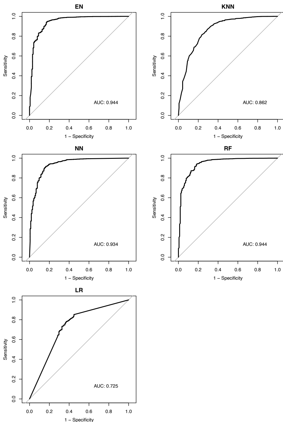
Fig S2. Receiver Operating Characteristics (ROC) Curve Estimating Area Under the Curve (AUC) for Models Classifying Dual Lifetime Tobacco and E-cigarette Use. EN = Elastic Net, KNN = K-nearest neighbors, NN = Neural networks, RF = Random forest, LR = Logistic regression.
