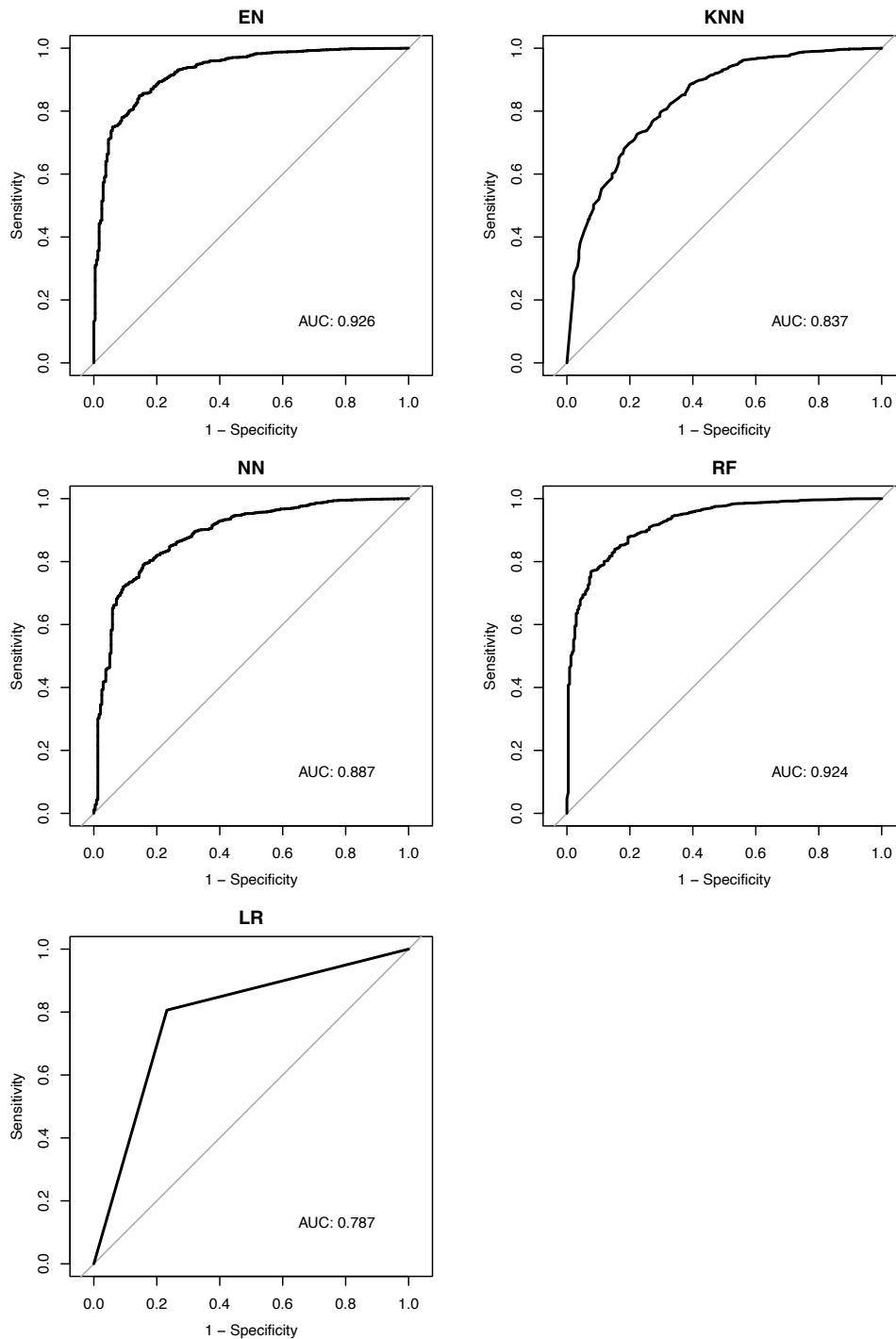
Fig S1. Receiver Operating Characteristics (ROC) Curve Estimating Area Under the Curve (AUC) for Models Classifying Exclusive Lifetime E-cigarette Use. EN = Elastic Net, KNN = K-nearest neighbors, NN = Neural networks, RF = Random forest, LR = Logistic regression.
