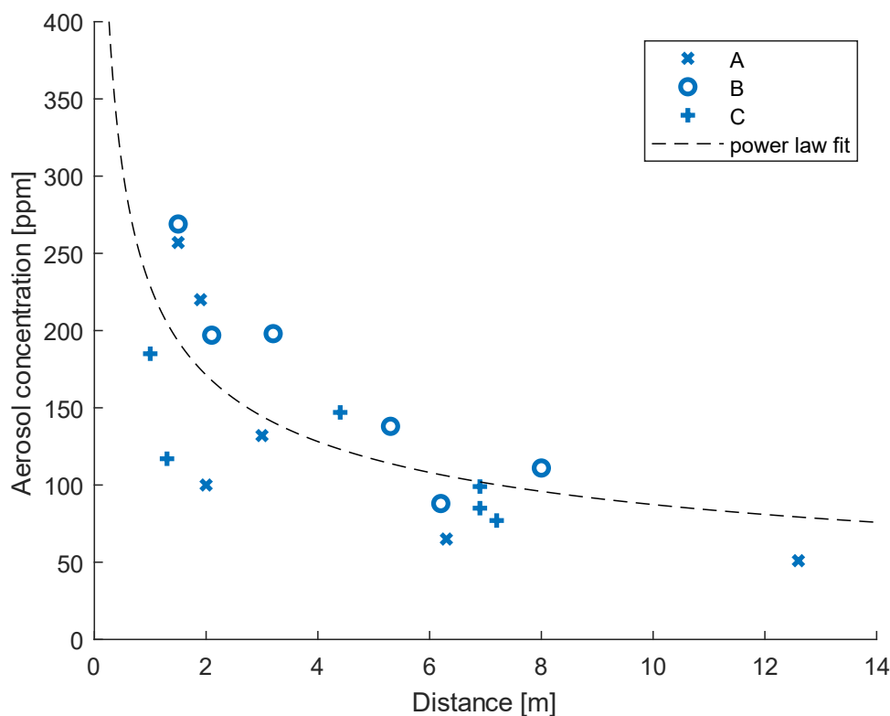
Figure 7: In the MVV, the aerosol amount decreases with increasing distance from the absorbers. This relation can be described with a power law (black curve, f(x) = a \cdot x^b , a = 228.8 , b = -0.418 , R\text{-square} = 0.51 ).
