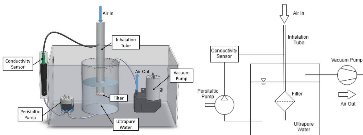
Figure 1: Illustration of an absorber: the aerosol is sucked through the inhalation tube into a closed reservoir filled with ultrapure water by a vacuum pump. The filter attached to the inhalation tube dissolves the NaCl particles in the ultrapure water. The ultrapure water is pumped through the sensor by a peristaltic pump.
