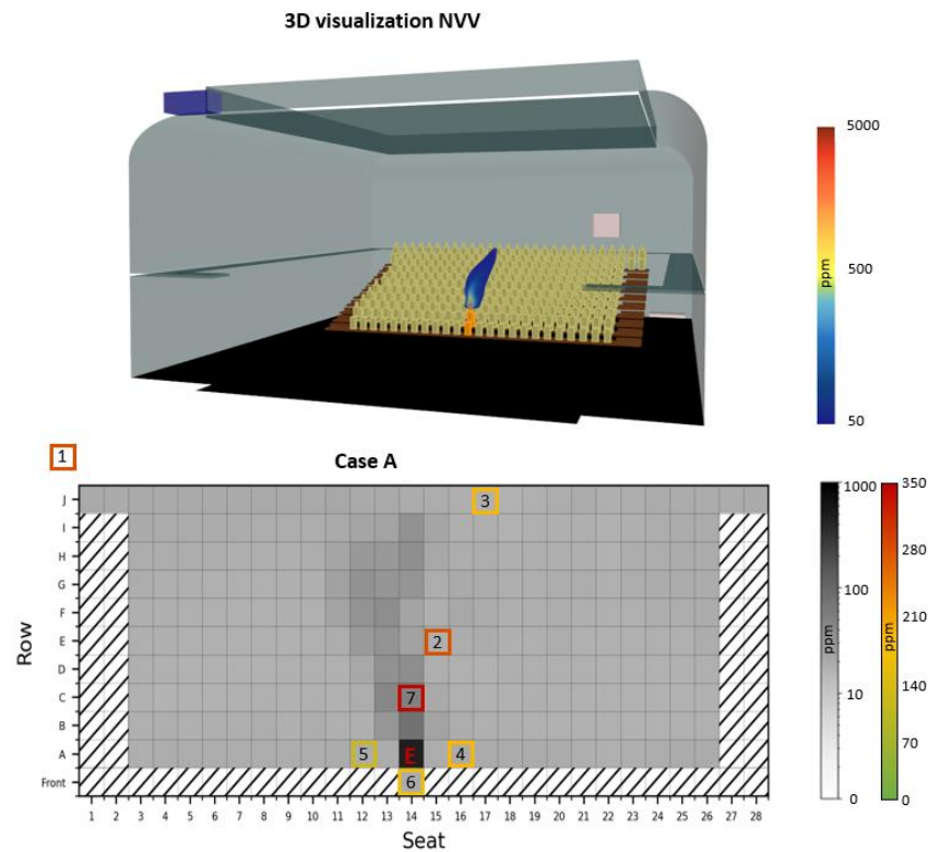
Figure 5: Experimental and simulated results of NVV. In the 3D visualization the yellow dummy represents the position of the aerosol generator measured with the experimental setup. The cloud over the yellow dummy is showing the aerosol plume dispersing in space calculated from numerical data. In Case A, the aerosol generator is positioned in the first row A14.
