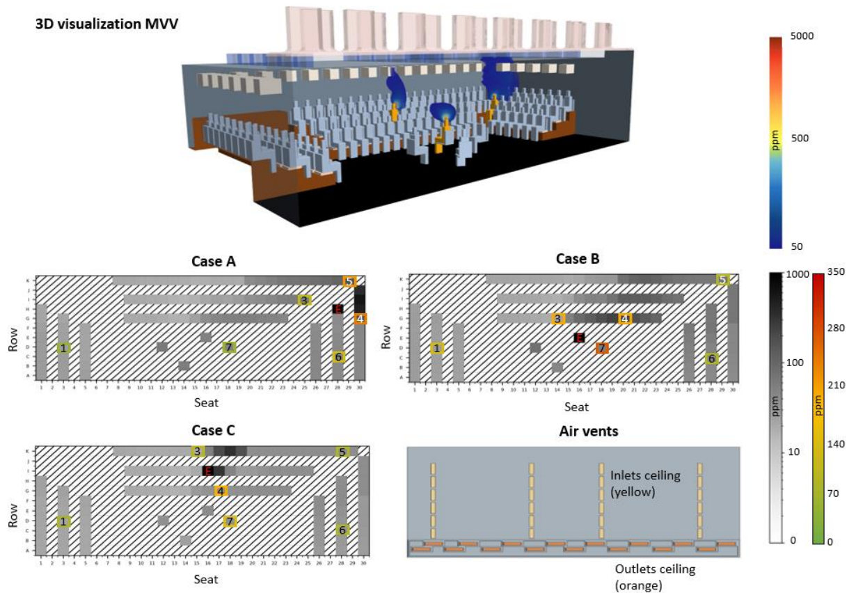
Figure 4: Experimental and simulated results of the three investigated emitter positions in MVV. In the 3D visualization the yellow dummies represent the positions of the aerosol generator measured with the experimental setup. A schematic representation of the air vents is shown (bottom right). The ventilation inlets are displayed in yellow and the ventilation outlets in orange. Both are located at the ceiling. The clouds over the yellow dummies are showing the simulated aerosol plume. The three generator positions are: (Case A) aerosol generator on the right H29, (Case B) aerosol generator on the stage E14 and (Case C) aerosol generator in the back I16. E shows the position of the aerosol generator, number 1-7 the position of the absorbers. The colour of their frame indicates the measured aerosol amount.
