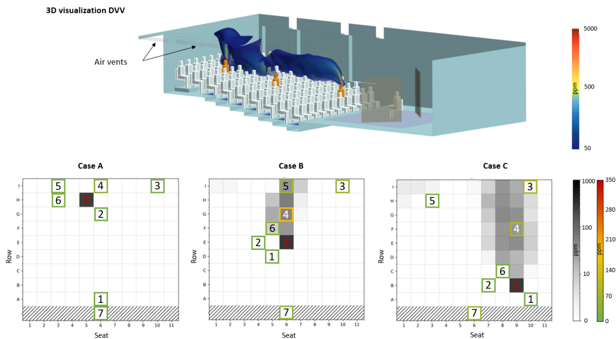
Figure 3: Experimental and simulated results of the three investigated emitter positions in DVV. In the 3D visualization the yellow dummies represent the positions of the aerosol generator measured with the experimental setup. Fresh air is inserted to the room under the seats and the polluted air is removed via air vents at the ceiling. The clouds over the yellow dummies are showing the aerosol plume dispersing in space calculated from numerical data. The three generator positions are: (Case A) aerosol generator in the back H5, (Case B) aerosol generator in the middle E6 and (Case C) aerosol generator in the front B9. E shows the position of the aerosol generator, number 1-7 the position of the absorbers. The colour of their frame indicates the measured aerosol amount. During the measurements heat sources were placed on the seats.
