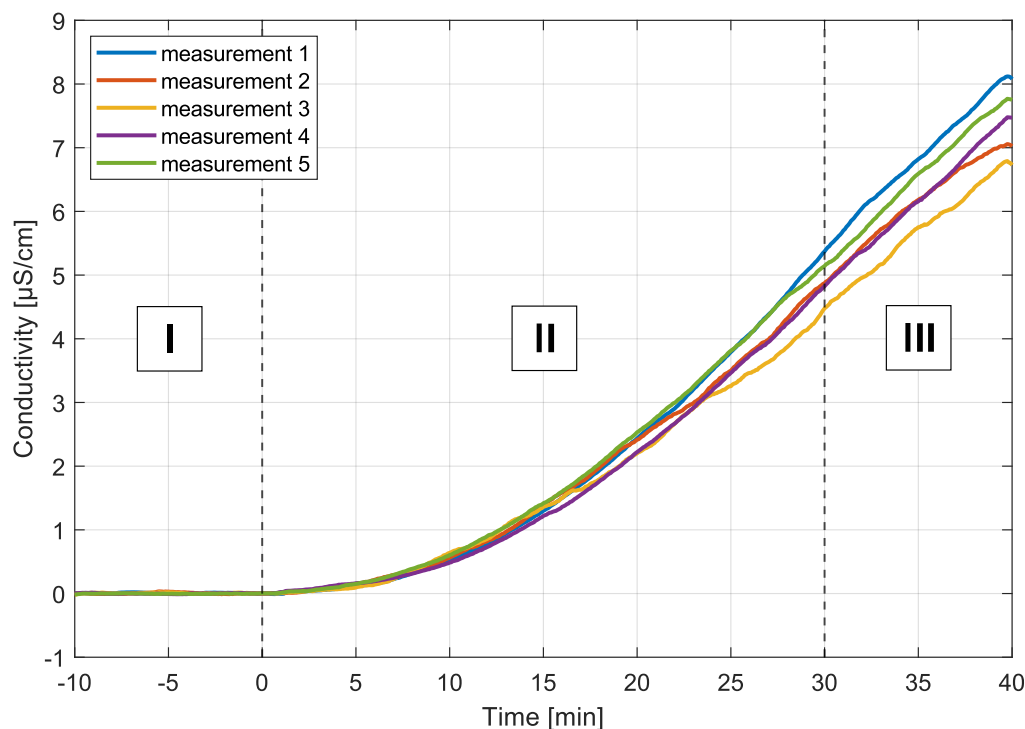
Figure 2: Increase in conductivity over time during a measurement procedure. The measurement procedure can be divided into three periods: lead-in (I), emission (II) and lead-out (III). Each measurement shows the mean value of the conductivity of all absorbers in the room. The lead-in time starts 10 min before the release of the aerosol. Then aerosol is released for 30 min and an increase in conductivity in the absorber can be observed. After 30 min the aerosol release stops, and the increase of the conductivity slows down.
