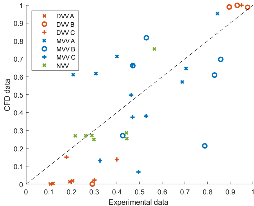
Figure 8: Comparison of normalized data points from CFD simulation and experimental measurements. Each colour represents a different venue. R-square values for the values compared to the perfect match (black dashed line): DVV R-square = 0.8633, MVV R-Square = -0.1845 and NVV R-Square = 0.5155.
