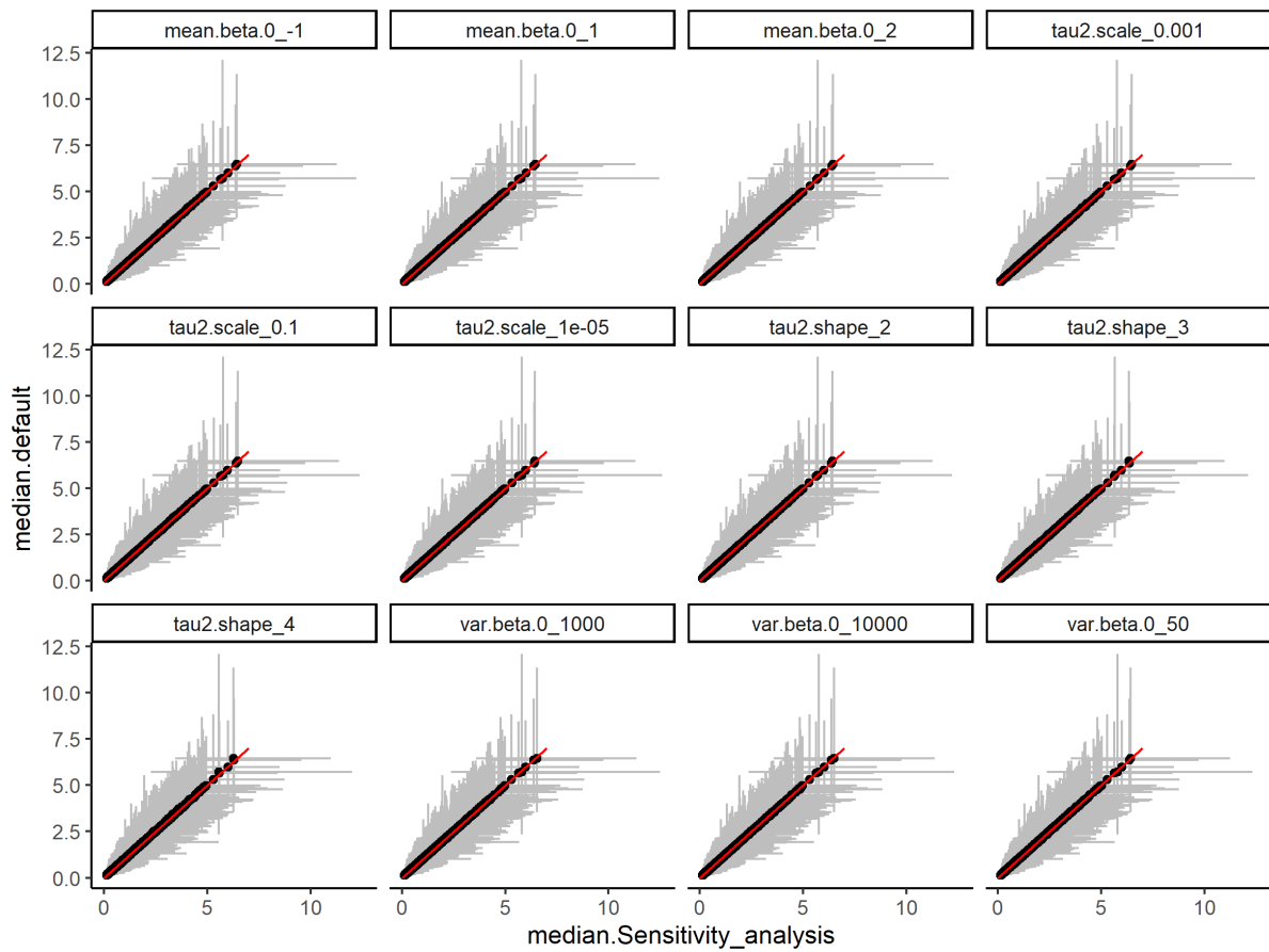
Figure S4; Results of the sensitivity analysis for high dose rate brachytherapy. The y-axis shows the median SSR (and 95% credible interval) for each area using the default value for the hyperprior and the x-axis shows the median SSR (and 95% credible interval) for each area using the hyperprior value specified in the label for the subplot. The line of equality is shown in red to guide the eye.
