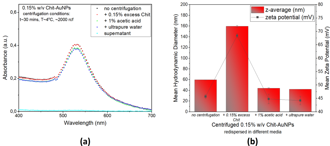
Figure S2: a) UV-Vis spectra, b) DLS and ZP measurements, of the 0.15% (w/v) Chit-AuNPs, after centrifugation and redispersion in different solvents (0.15% (w/v) Chit in 1% (v/v) aqueous acetic acid, 1% (v/v) aqueous acetic acid, ultrapure water).
