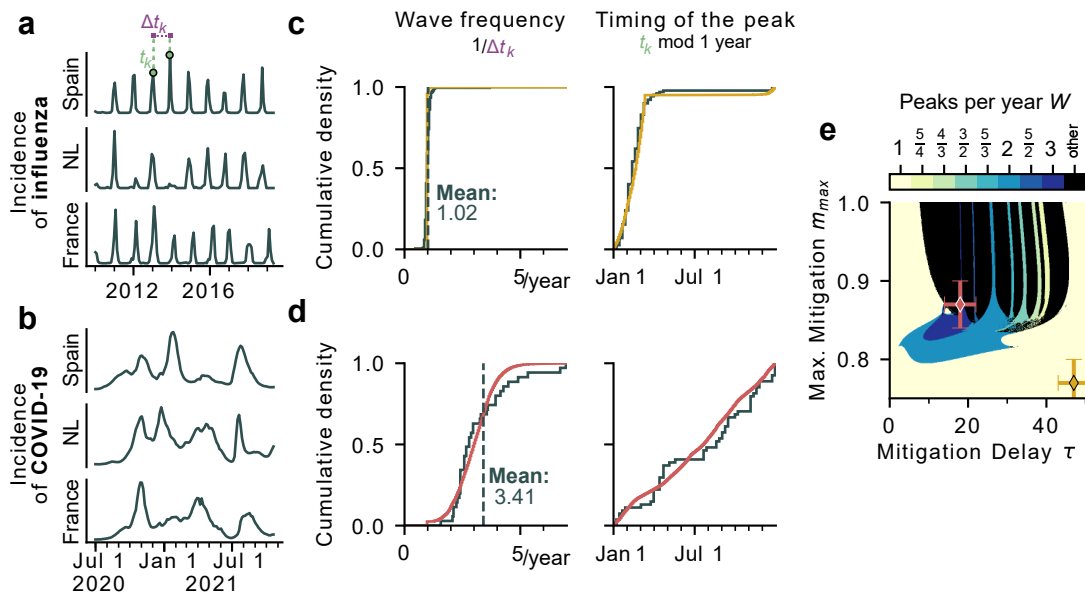
Figure 5: Wave characteristics in northern countries suggest that the spread of COVID-19 lied within the regime of complex dynamics. a,b) We collected timeseries of COVID-19 (summer 2020 until the spread of the Omicron variant) and seasonal influenza (2010 to 2019) incidence in several northern countries (Supplementary Sec. C) and extracted the wave frequency, i.e., the inverse time between consecutive waves, and the time of the year at which incidences peaked. c) Influenza waves show a narrowly peaked distribution of wave frequencies around 1 peak per year with this peak occurring predominantly between January and March. d) Wave frequencies show a broad distribution from 1 to 7 peaks per year in COVID-19 data. These peaks were observed all year long. e) For comparison with our model, we sampled trajectories around points in the \tau - m_{\max} -plane with Gaussian weights to also extract the wave frequencies and peak timings in simulations. The resulting model distributions resemble those observed for COVID-19 in the regimes of complex dynamics (red in d,e) and those of influenza in the regime of yearly peaks and weak mitigation (yellow in c,e). Errorbars in e) indicate the widths of the Gaussian sample ( \sigma_{\tau} = 4 , \sigma_{m_{\max}} = 0.03 ).
