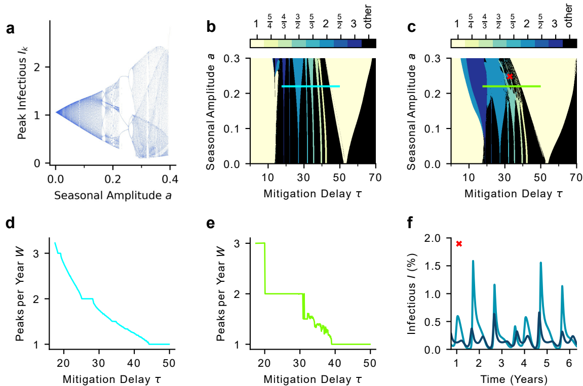
Figure 3: Phase-locking, chaotic wave patterns and coexisting attractors in the SIRSsm model. a) A peak diagram , i.e., a scatter plot of peak incidences I_k of a long timeseries against the seasonal amplitude a . Increasing a leads to transitions between high-periodic, low-periodic, and chaotic behaviour. Parameters used: \tau = 32.5 , m_{\max} = 0.85 . b,c) The averaged number of peaks per year W shows Arnold tongues in the \tau - a plane as the result of phase-locking. For strong maximal mitigation the tongues are well separated ( m_{\max} = 0.86 , panel b) while they overlap for weaker maximal mitigation ( m_{\max} = 0.84 , panel c). Tongues are displayed only for the ratio of small integers. Cross sections through the Arnold tongues at a = 0.22 (green and cyan lines) show a typical Devil’s staircase for m_{\max} = 0.86 (d) but one that includes steep jumps and chaos for m_{\max} = 0.84 (e). f) Areas where different tongues overlap give rise to coexisting attractors, i.e., two or more asymptotic states for the same set of model parameters, approached by different initial conditions. The example uses a = 0.248 , \tau = 32.8 (red cross in c), S(0) = 0.521 and I(0) = 0.001 vs I(0) = 0.361 .
