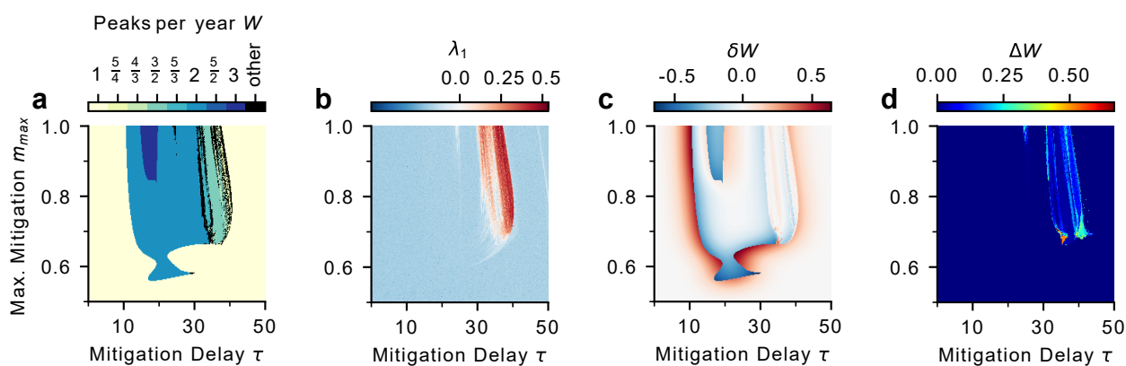
Figure 11: Complexity in the SIRSsm model also arises for a lower spreading rate. Using R_0 = 2 different measures indicate complex dynamics in the \tau - m_{\max} -plane. a) The number of peaks per year W does not show clear Arnold tongues as for R_0 = 5 , but neighbouring areas of different W interrupted by chaotic motion. b) The largest Lyapunov exponent \lambda_1 can get similarly large as for R_0 = 5 , namely \lambda_1 \approx 0.5 , implying significant divergence of initial conditions in about two years. c) Parameter variations obtained by Gaussian-weighted samples of trajectories around each point (with widths \sigma_\tau = 4 , \sigma_{m_{\max}} = 0.03 ) indicate the expected change in peaks per year \delta W as large as \delta W = 0.6 . d) Coexisting attractors also emerge for R_0 = 2 with different numbers of peaks per year as large as \Delta W = 0.75 across attractors.
