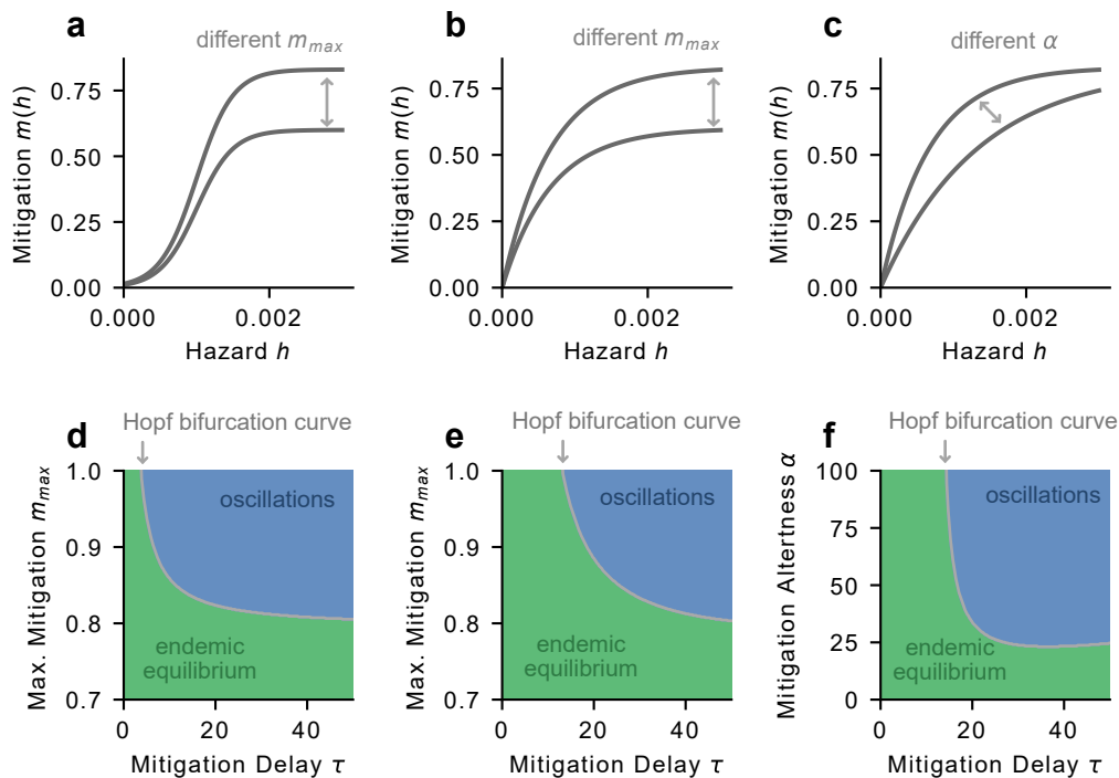
Figure 8: Various mitigation-hazard feedbacks trigger a Hopf bifurcation. The onset of oscillations due to a Hopf bifurcation is not unique to one specific example for the functional form of m(h) . Instead, for different functional shapes of m(h) oscillations emerge when maximal mitigation m_{max} and mitigation delay \tau are large enough (a,d for a logistic feedback, b,e for an exponential feedback). c,f) Mitigation alertness \alpha is the other free variable of the exponential feedback. If it is large enough, namely mitigation increases fast enough with hazard, oscillations emerge. Model parameters used are found in Tab. 1. For b,e \alpha = 1500 was used. For c,f m_{max} = 0.83 was used.
