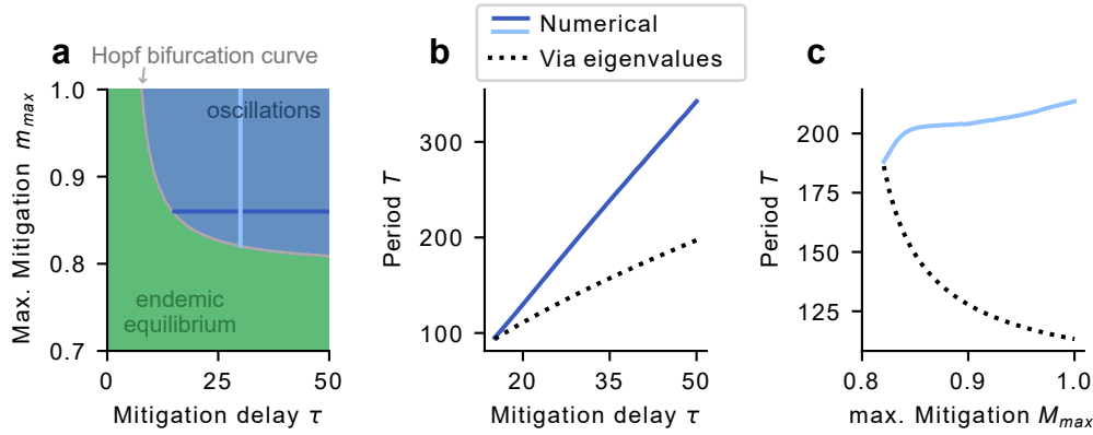
Figure 6: The period of the SIRS model (no seasonality) increases linearly with the mitigation delay. a) For large mitigation delay \tau and strong maximal mitigation m_{\max} the endemic equilibrium turns unstable through a Hopf bifurcation. The period of the oscillation at the bifurcation point is given by the imaginary part of the bifurcating eigenvalues of the Jacobian. b) The period of the oscillations increases linearly with the mitigation delay \tau , though the approximation through the eigenvalues quickly deteriorates beyond the bifurcation curve. c) Maximal mitigation m_{\max} does not influence the period of the oscillations as much.
