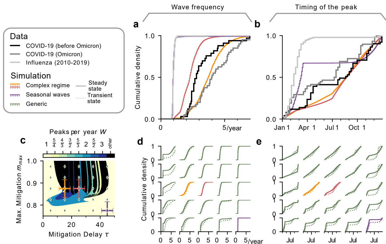
Figure 7: Wave characteristics quickly equilibrate to their steady-state distributions. In Fig. 5 we compared data from the first two years of COVID-19 (leaving out the very first outbreaks and stopping when the Omicron variant emerged) to steady-state model simulations. Here we check the validity of this approach by simulating the model only for two years (leaving out only the first 180 days, i.e. the first outbreaks) and also compare to data for the Omicron variant. Full, coloured lines represent the steady-state distributions as in Fig. 5, dashed lines the two year simulations. a,b ) COVID-19 spread for the Omicron variant (grey curve) has a slightly different distribution of wave frequencies and wave timings than for pre-Omicron COVID-19 (black curve), but is still close to distributions of model simulations in the complex regime (orange and red curves). c-e ) For both the wave frequencies and the wave timings the model parameter sets that match COVID-19 data before Omicron qualitatively in the steady state also match the data in the two-year simulations and for Omicron. A 5x5 grid is placed onto the \tau - m_{max} -plane and distributions are sampled around the centre points of the grid. The distributions are only slightly affected by the steady-state assumptions all over parameter space.
