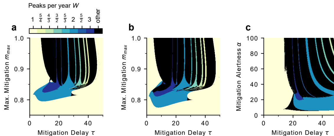
Figure 9: Arnold tongues emerge for different feedbacks m(h) (Fig. 8). a) Arnold tongues for the softplus feedback used in the main text. b) Arnold tongues for a logistic feedback (Eq. 21). c) The number of peaks per year W shows Arnold tongue-like structures using an exponential feedback (Eq. 22) and the mitigation alertness \alpha as free parameter.
