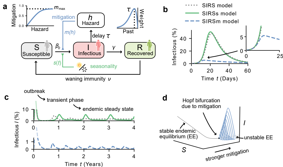
Figure 1: Model overview a) The SIRSsm model: An extended SIRS model including periodic seasonality ( s , green) and mitigation from behavioural feedback ( m , blue). The population is divided into compartments according to their disease status: Susceptible (S), infectious (I) or recovered (R). Mitigation m increases with hazard h and saturates at a maximum mitigation level of m_{\max} . Hazard h is calculated as the convolution of the infectious compartment I with a delaying kernel of mitigation delay \tau (peak of the kernel). Yearly seasonality s(t) periodically modulates the infection rate. b) For a novel disease outbreak, classic SIRS models (with or without seasonality s , resp. green and grey) feature initial exponential growth in incidence, slowed down and eventually stopped only by immunity. In contrast, with behavioural feedback, the incidence is kept considerably lower due to mitigation (blue, see inset). c) Following the initial outbreak and a transient phase, incidence levels settle into their endemic steady state. In SIRS models without feedback, this equilibrium is a constant (grey) or oscillates (with seasonality, green). However, including the behavioural feedback can also lead to periodic waves even in the absence of seasonality. These are triggered by a supercritical Hopf bifurcation (d) . The frequency of these waves is set by the mitigation delay \tau (Supplementary Sec. B). Parameters used in b,c : \beta_0 = 0.5, \gamma = 0.1 . Green: a = 0.25, m_{\max} = 0, \nu = 1/500 , Blue: a = 0, m_{\max} = 0.84, \tau = 30, \nu = 1/100 .
