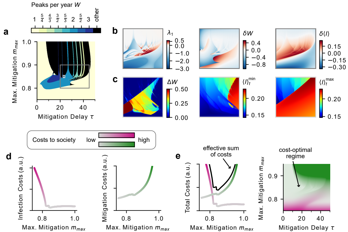
Figure 4: Complex, unpredictable regimes can coincide with cost-optimal regions. a) The number of peaks per year W in the parameter plane spanned by maximal mitigation m_{max} and mitigation delay \tau shows Arnold tongues. The complexity of the dynamics is characterised by different quantities visualised in two insets (grey rectangles): b) Disease prediction is impeded for a large range of parameters (dark grey rectangle in panel a). The largest Lyapunov exponent \lambda_1 is as large as \lambda_1 = 0.62 \text{ years}^{-1} , which corresponds to a Lyapunov time of 1.6 years (left panel). Parameter variations obtained by Gaussian-weighted samples of trajectories around each point (with widths \sigma_\tau = 4 , \sigma_{m_{max}} = 0.03 ) indicate the expected change in peaks per year \delta W as large as \delta W = 0.53 (mid panel) and the expected change of average infections \delta \langle I \rangle_t as large as \delta \langle I \rangle_t = 0.27\% (right panel). c) High complexity manifests already in small regions of mitigation parameter space (light grey rectangle in panel a): At fixed parameters both the number of peaks per year W and average infections \langle I \rangle_t differ between coexisting attractors, approached by different initial conditions. This can lead to one additional peak every two years ( \Delta W = 0.5 , left panel) and up to 50% more infections (local difference between the attractors with minimal infections \langle I \rangle_t^{\min} (mid panel) and maximal infections \langle I \rangle_t^{\max} (right panel)). d) Both infections and the implementation of mitigation strategies come at a cost to society. Assuming that the costs of infections C_I(t) are proportional to infections I , the average costs over time \langle C_I \rangle_t are over-proportionally high if maximal mitigation is not sufficient (here for \tau = 20 ). e) Average costs of mitigation \langle C_m \rangle_t are high for strong maximal mitigation; we assumed costs to diverge for m_{max} \rightarrow 1 (using C_m(t) \propto \frac{1}{1-m(h(t))} - 1 ). f) A cost-optimal regime emerges as a balance between the individual costs for infections and mitigation. g) The cost-optimal region can coincide with the region of chaotic motion and sensitive parameter dependence. The costs are visualised by adapting the colour opacity, not explicitly weighing the costs.
