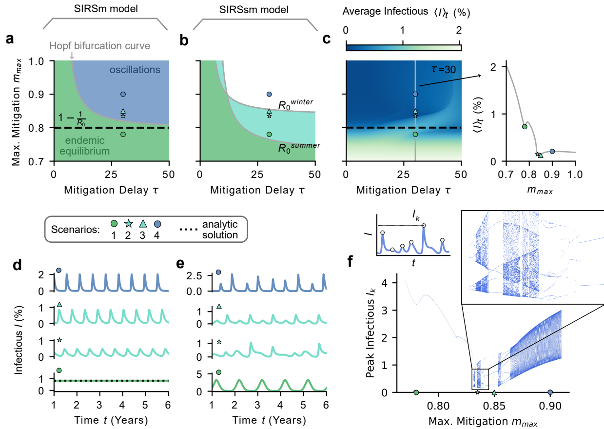
Figure 2: The interplay between seasonality and behavioural feedback opens a rich variety of dynamical regimes. We illustrate different regimes in four scenarios indicated by markers. a) Without seasonality (i.e., seasonal amplitude a = 0 ), the system has a fixed point that turns unstable through a Hopf bifurcation if maximal mitigation m_{\max} and delay \tau are large enough ( m_{\max} \geq 1 - \frac{1}{R_0} = 0.8 , blue zone). b) With seasonality (here a = 0.25 ), the non-autonomous system ceases to possess a fixed point. Computing bifurcation curves with fixed summer- and winter-adjusted spreading rates ( R_0^{\text{summer}} = R_0(1 - a) , R_0^{\text{winter}} = R_0(1 + a) ) allows to separate different regimes: Seasonality-dominated (green), mitigation-dominated (blue) and balanced (cyan). c) Average infections \langle I \rangle_t (colour coded) in the endemic steady state decrease strongly if mitigation can effectively be stronger than the spread, i.e., if m_{\max} > 1 - \frac{1}{R_0} (here computed with seasonality, a = 0.25 ). d) In the endemic steady state without seasonality, scenario 1 has a stable equilibrium and scenarios 2-4 display oscillations. e) With seasonality, scenarios 1-4 show four qualitatively different dynamics: Sc. 1 shows yearly waves of infections. Sc. 2 shows chaotic dynamics whereas Sc. 3, which only differs slightly in m_{\max} , shows two waves per year. Sc. 4 displays high periodic dynamics. f) For a long timeseries, all peak heights are plotted against the parameter m_{\max} , resulting in a peak diagram. Scenario parameters: a = 0.25 , \tau = 30 , m_{\max} = 0.78, 0.835, 0.85, 0.9 .
