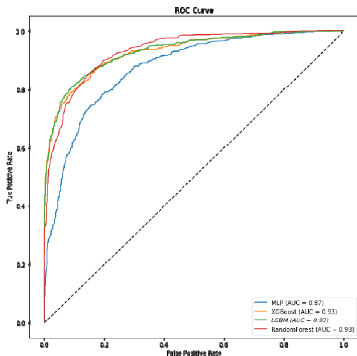
Figure 3. ROC-AUC curve
