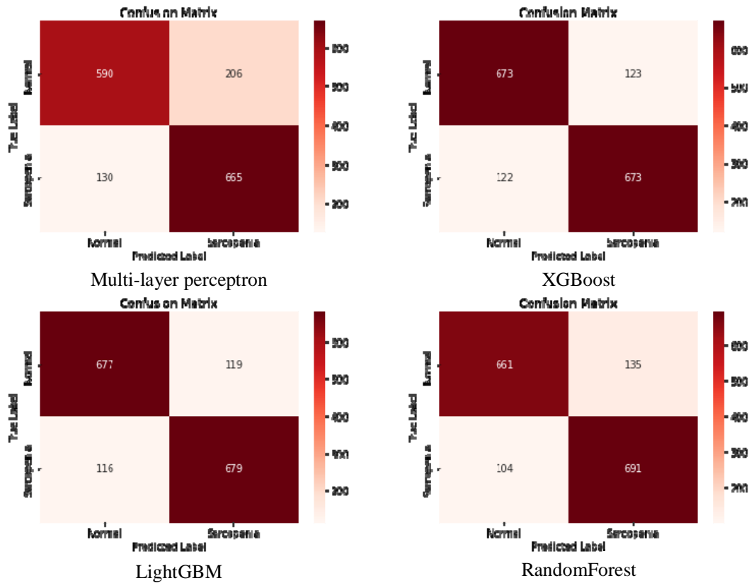
Figure 2. Confusion matrix of sarcopenia prediction model
