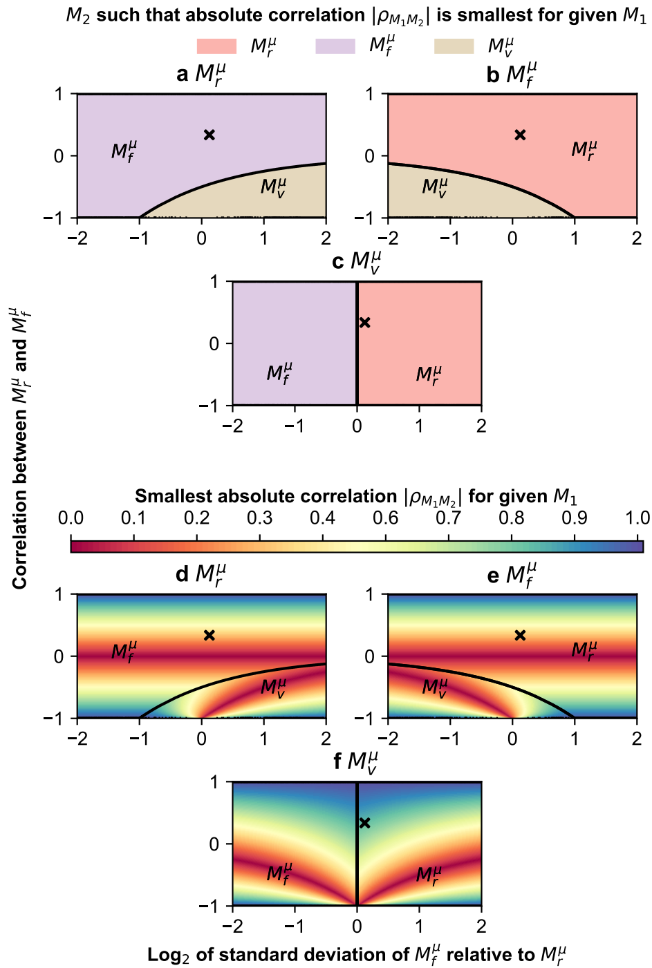
Fig. S13. When using the regional expected fake news detection ability score as the first predictor in regressing for regional outcomes, using the regional expected real news detection ability score as the second predictor minimizes collinearity when predicting regional outcomes. x -axis indicates logarithm of the standard deviation \sigma_{rf} of M_f^\mu relative to M_r^\mu , and y -axis indicates the linear correlation \rho_{rf} between M_r^\mu, M_f^\mu . (Top) Parameter space identifying the second predictor having the smallest absolute value of linear correlation with the given first predictor: see Eq. S34. (Bottom) Smallest possible absolute value of linear correlation between the second predictor and the given first predictor. Marker \times indicates the location \sigma_{rf} = 1.076, \rho_{rf} = 0.333 corresponding to the posterior means of the poststratified expectation of real and fake news detection ability scores in the United Kingdom.
