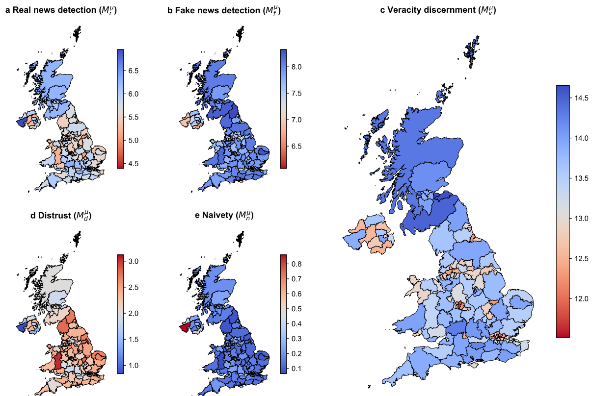
Fig. S9. Misinformation susceptibility test (MIST) scores mapped across the United Kingdom (UK). Panels a-e indicate poststratified regional estimates of expected ability scores of real news detection ( M_r^\mu , a ), fake news detection ( M_f^\mu , b ), veracity discernment ( M_v^\mu , c ), and expected bias scores of distrust ( M_d^\mu , d ), and naivety ( M_n^\mu , e ). Colors indicate posterior means of the poststratified estimate of expected MIST scores in every region, with blue (red) indicating higher ability (bias) scores and thus lower (higher) misinformation susceptibility. See Table S11 for full posterior values.
