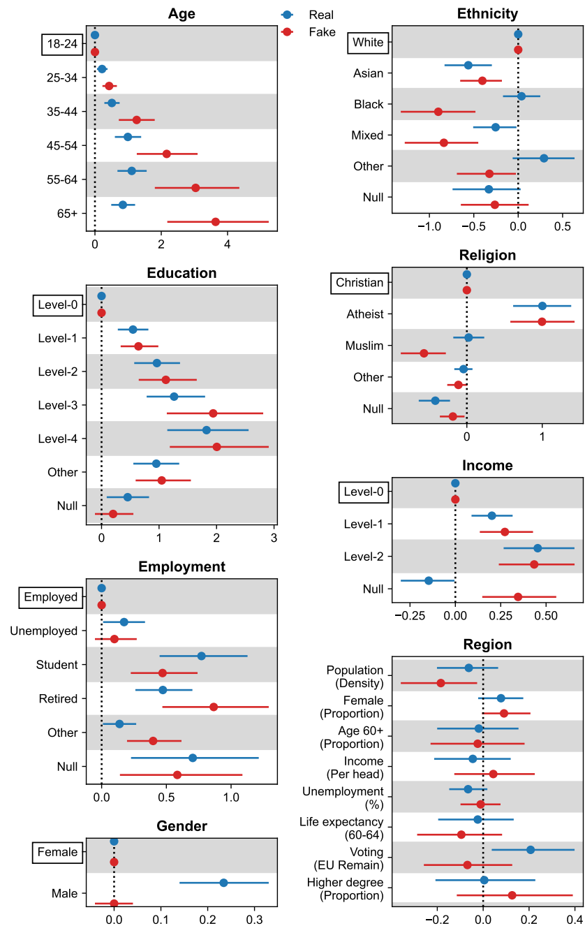
Fig. S8. Being older, more educated, atheist, of white ethnicity, and earning higher income, are individual characteristics associated with improved abilities to detect real and fake news headlines in Great Britain. Those who are students or retired have higher real and fake news detection abilities, while those who are Asian or have a mixed ethnicity have lower real and fake news detection abilities. Being male is associated with a higher real news detection ability, while being Black or Muslim is associated with a lower fake news detection ability. At the region level, residing in a region with a larger proportion of those who voted to “remain” in the EU referendum is strongly indicative of a higher real news detection ability, whereas those in densely populated regions have a lower fake news detection ability. Panels correspond to different individual covariates, except for the last panel “Region” that corresponds to regional covariates. “Null” corresponds to undisclosed socio-demographic identity; see Table S2 for full variable recodes. Markers indicate posterior means while bars indicate 95% HPDIs. For each individual covariate, the reference group is indicated by a bounding box and markers at 0 and bars of 0 length. See Table S9 for full posterior values.
