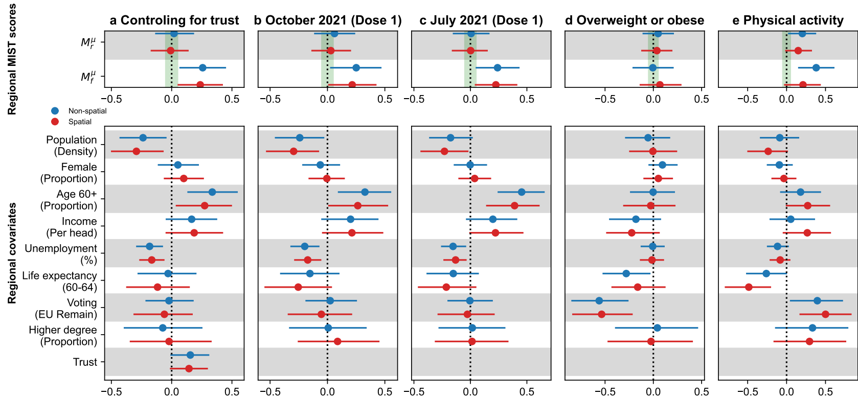
Fig. S19. Posterior estimates of standardized coefficients in a secondary set of regression models for COVID-19 vaccine’s second dose (while controlling for trust in experts; a ) and first dose regional uptake rates in England and Scotland (at two timepoints; b, c ), and two placebo outcomes in England ( d, e ). Markers indicate posterior means while bars indicate 95% HPDIs of the standardized coefficients of real ( M_f^H ) and fake ( M_f^L ) news detection ability scores, both before (blue) and after (red) controlling for spatial effects of regional adjacency, with the green shaded region indicating the preregistered region of practical equivalence (ROPE) to null effects of (-0.05, 0.05) . The models control for a set of regional covariates, and dotted line indicates the reference value of 0. See Tables S15 and S17 for full posterior values.
