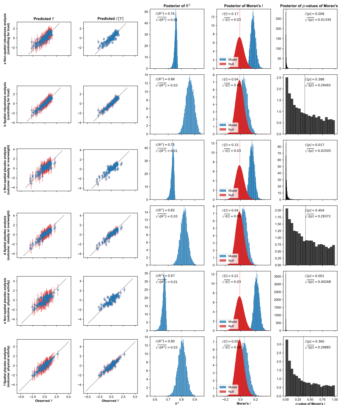
Fig. S21. Posterior distributions of R^2 of vaccine uptake (a, b) and other placebo outcomes (c-f), and Moran's I statistic for different regional regression models. Additional analyses checked for explicit confounding by considering the outcome of second dose uptake as of 1 October 2021 while controlling for trust in expert sources of COVID-19 information (a, b), while placebo analyses considered various placebo outcomes that are expected to be influenced by trust in expert authority or willingness to follow expert advice but not by misinformation exposure—namely the proportion of obese or overweight adult population (c, d) and the proportion of physically active adult population (e, f)—both before (a, c, e) and after (b, d, f) controlling for spatial effects of regional adjacency. All models include regional real and fake news detection ability scores as predictors, while controlling for a set of regional covariates. For the two leftmost columns, markers indicate posterior means while bars indicate 95% HPDIs, while the other columns display entire posterior distributions. Posterior means of the p -value (rightmost column) for Moran's I are less than 0.05 for non-spatial models, indicating “significant” spatial structure in the residuals of model predictions at level \alpha = 0.05 . Mean of the posterior of R^2 values is smaller throughout the non-spatial models when compared to spatial models, suggesting that the spatial structure explains a significant amount of variance in outcomes considered. For a residual analysis see Fig. S23.
