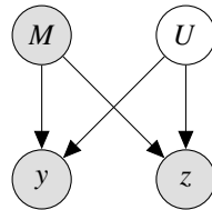
(c) Large \beta_M^z consistent with no confounding
