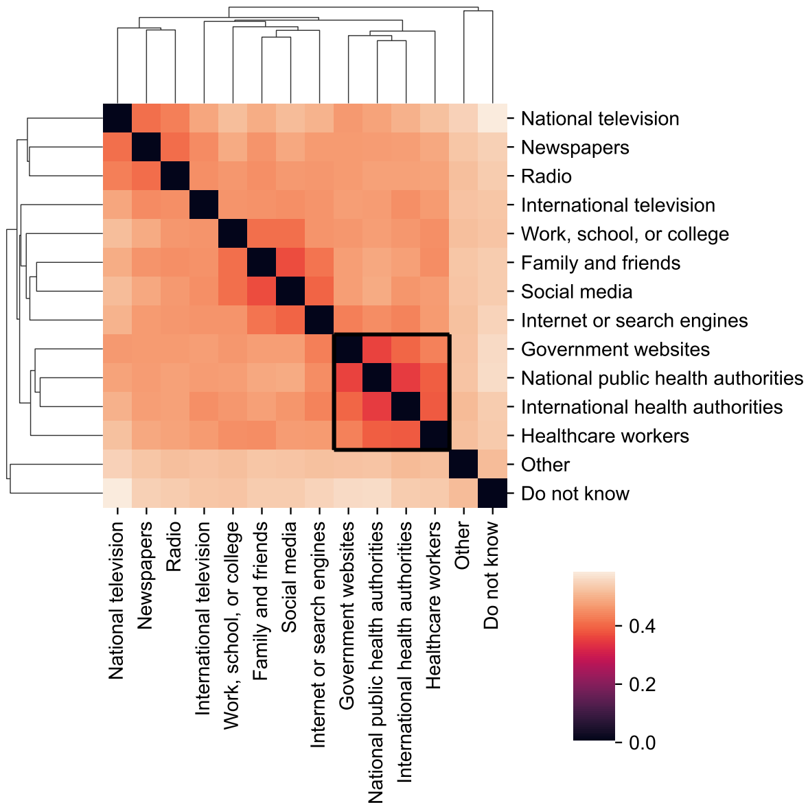
Fig. S16. Sources of information regarding the COVID-19 pandemic naturally cluster into expert and non-expert sources based on whether they are trusted. Binary responses indicating which sources of information regarding the COVID-19 pandemic were trusted by survey respondents (see Questionnaire ) were used to compute a “distance” (color) between every source pair a, b —given by \frac{1-\varphi_{ab}}{2} where \varphi_{ab} \in [-1, 1] indicates the phi-coefficient, a balanced measure of similarity between binary responses [S34] equivalent to the standard Pearson’s correlation coefficient for binary responses—and clustered using agglomerative clustering [S35] with the average linkage criterion [S36] as implemented in SciPy [S33]. Consequently, the sources of information can be naturally bi-partitioned into “expert” sources—government websites, public health authorities and healthcare workers (see black square)—and “non-expert” sources—the rest.
