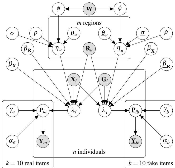
Fig. S2. Graphical representation for the social-IRT models inferring individuals' abilities to detect real and fake news. Observed variables are shaded gray, latent variables are colored white, and hyperparameters are excluded for clarity. Variables specific to fake news detection appear underlined. The 2-parameter item response theory models encode for the latent item parameters of “difficulty” \alpha and “discrimination” \gamma , and the latent ability of individuals \lambda to correctly identify a real/fake news headline \mathbf{Y}/\underline{\mathbf{Y}} : see Eq. 1. The latent ability is a function of individual covariates \mathbf{X} , regional covariates \mathbf{R} and random effects \eta corresponding to the individual's region of residence \mathbf{G} : see Eq. 2. Regional random effects \eta are decomposed into an unstructured component \theta , and a structured component \phi that accounts for regional covariance as per inter-regional “connectivity strengths” \mathbf{W} : see Eqs. 3 and 5. The parameter \rho encodes the contribution of structured random effects, while \sigma encodes overall scale of random effects. This graphical model encodes the conditional independence of \mathbf{Y} and \underline{\mathbf{Y}} given the individuals' abilities \lambda and \underline{\lambda} , allowing for two separate models to be inferred for real and fake news detection abilities respectively.
