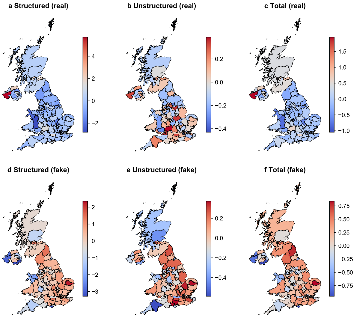
Fig. S7. Random effects of the social-IRT models based on social connectivity volumes between regions, for modeling real (a-c) and fake (d-f) news detection abilities, mapped across the United Kingdom (UK). Panels a, d indicate the structured effect, b, e indicate the unstructured effects, and c, f indicate the total random effect of the models. Colors indicate posterior means of the random effects.
