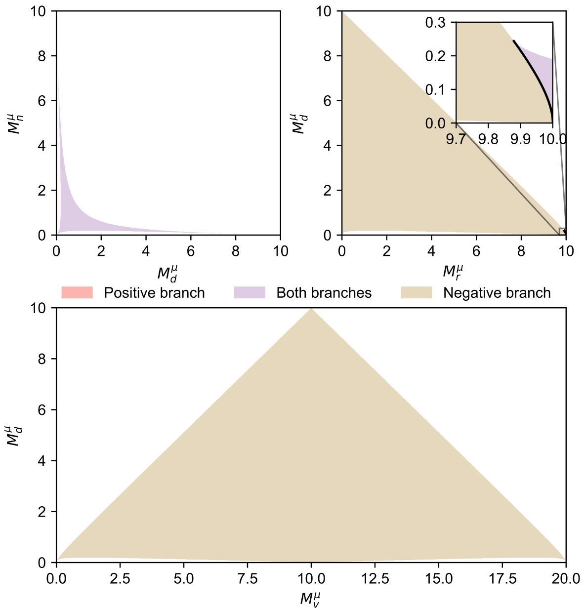
Fig. S15. MIST bias scores are insufficient as exogenous MIST predictors when predicting regional outcomes. For each given pair of regional MIST scores, each panel shows the parameter space that yields one or more valid solutions for the remaining MIST scores, using Eq. S33 with k = 10 items. Regional distrust bias score M_d^\mu completely determines the remaining MIST scores only alongside the veracity discernment ability score M_v^\mu .
