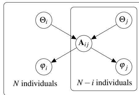
Fig. S3. Graphical representation for individual random effects under a statistical network model. Individual-level random effects \varphi depend on whether there is a direct connection between two individuals in the social network, as encoded in the network's adjacency matrix \mathbf{A} : see Eq. S1. In turn, the existence of a connection between any two individuals depends entirely on their location in some d -dimensional space \Theta : see Eq. S5. This graphical model encodes the conditional independencies in Eqs. S3 and S4.
