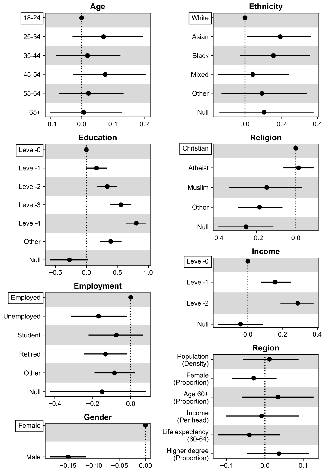
Fig. S17. Individual-level regression models for self-reported trust in an expert source of COVID-19 information. Markers indicate posterior means while bars indicate 95% HPDIs of the coefficients of individual socio-demographics and regional fixed effects (“ Region ”), while including random effects structured by social connectivity volumes. For each individual covariate, the reference group is indicated by a bounding box and markers at 0 and bars of 0 length. “Null” corresponds to undisclosed socio-demographic identity; see Table S2 for full variable recodes. The dotted line indicates the reference value of 0. See Table S19 for full posterior values.
