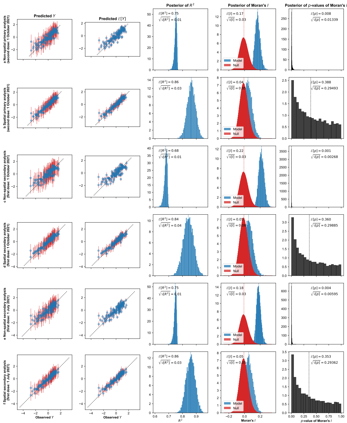
Fig. S20. Posterior distributions of R^2 of vaccine uptake and Moran's I statistic for different vaccine uptake models. Primary analyses considered second dose uptake as of 1 October 2021 ( a, b ), while secondary analyses considered first dose uptake as of 1 October 2021 ( c, d ) and 1 July 2021 ( e, f ), both before ( a, c, e ) and after ( b, d, f ) controlling for spatial effects of regional adjacency. All models include regional real and fake news detection ability scores as predictors, while controlling for a set of regional covariates. For the two leftmost columns, markers indicate posterior means while bars indicate 95% HPDIs, while the other columns display entire posterior distributions. Posterior means of the p -value (rightmost column) for Moran's I are less than 0.05 for non-spatial models, indicating “significant” spatial structure in the residuals of model predictions at level \alpha = 0.05 . Mean of the posterior of R^2 values is smaller throughout the non-spatial models when compared to spatial models, suggesting that the spatial structure explains a significant amount of variance in uptake. For a residual analysis see Fig. S22.
