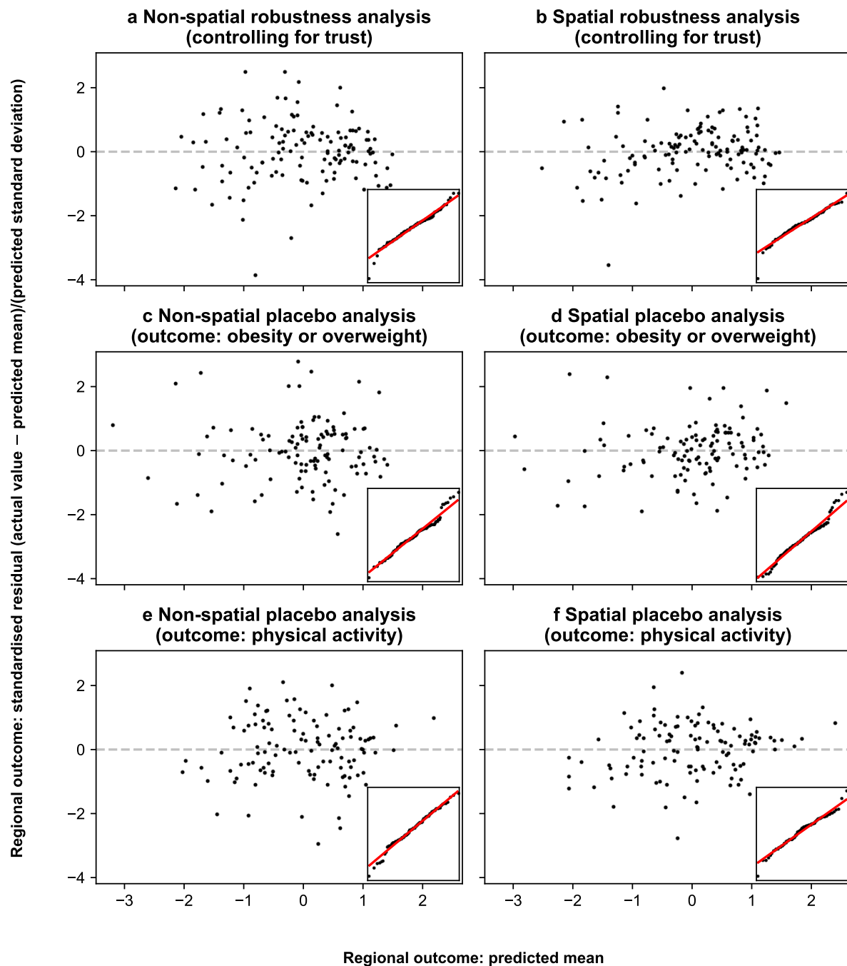
Fig. S23. Posterior means of standardised residuals of vaccine uptake (a, b) and other placebo outcomes (c-f) for different regional regression models. Additional analyses checked for explicit confounding by considering the outcome of second dose uptake as of 1 October 2021 while controlling for trust in expert sources of COVID-19 information (a, b), while placebo analyses considered various placebo outcomes that are expected to be influenced by trust in expert authority or willingness to follow expert advice but not by misinformation exposure—namely the proportion of obese or overweight adult population (c, d) and the proportion of physically active adult population (e, f)—both before (a, c, e) and after (b, d, f) controlling for spatial effects of regional adjacency. All models include regional real and fake news detection ability scores as predictors, while controlling for a set of regional covariates. Main plots show the posterior mean of the standardised residuals (on the y-axis) against the posterior mean of the outcome (on the x-axis)—we observe no apparent trend in the residuals suggesting homoscedasticity. Inset plots show the quantile-quantile plot for the standard normal distribution on the x-axis and for the (posterior mean of) standardised residuals on the y-axis, with the reference line in red—we observe a good fit suggesting that residuals are normally distributed.
