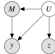
(b) Large \beta_M^z consistent with confounding
