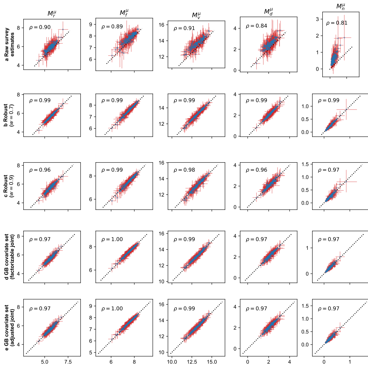
Fig. S11. Regional MIST scores are robust to different inclusion criteria for the United Kingdom, and to using an expanded set of covariates for Great Britain (GB). x -axis indicates posterior estimates of the poststratified expected MIST scores in the primary model, while the y -axis indicates raw survey estimates (a) and poststratified estimates from robustness checks (b, c) and secondary models (d, e) . Columns refer to different MIST scores: real news detection M_r^\mu , fake news detection M_f^\mu , veracity discernment M_v^\mu , distrust M_d^\mu , and naivety M_n^\mu . Row (a) indicates raw estimates of the mean MIST scores from the survey sample: markers indicate the sample mean on the y -axis while bars along the y -axis indicate 95% Bayesian confidence intervals of the mean [S32, S33]. Rows (b, c) indicate results when social-IRT models are inferred with different threshold w indicating the probability of an individual with a given outward postcode to map to a given grouped NUTS-3 region, since some outward postcodes may match to multiple grouped NUTS-3 regions. The primary model uses w = 0.5 (50 samples removed), whereas robustness checks consider more strict thresholds of w = 0.7 (b) and w = 0.9 (c) , with 765 and 2343 samples removed in total, respectively. Rows (d, e) indicate the results of secondary models for England, Scotland and Wales using the expanded covariate set. In particular, poststratification along an individual's income is performed either by assuming a factorizable joint distribution (d) or assuming an adjusted joint distribution (e) (see Supplementary methods: Poststratification with income variable ). For rows (b-e) markers indicate posterior means while bars indicate 95% HPDIs. \rho indicates the linear correlation coefficient between markers' values on the x - and y -axes.
