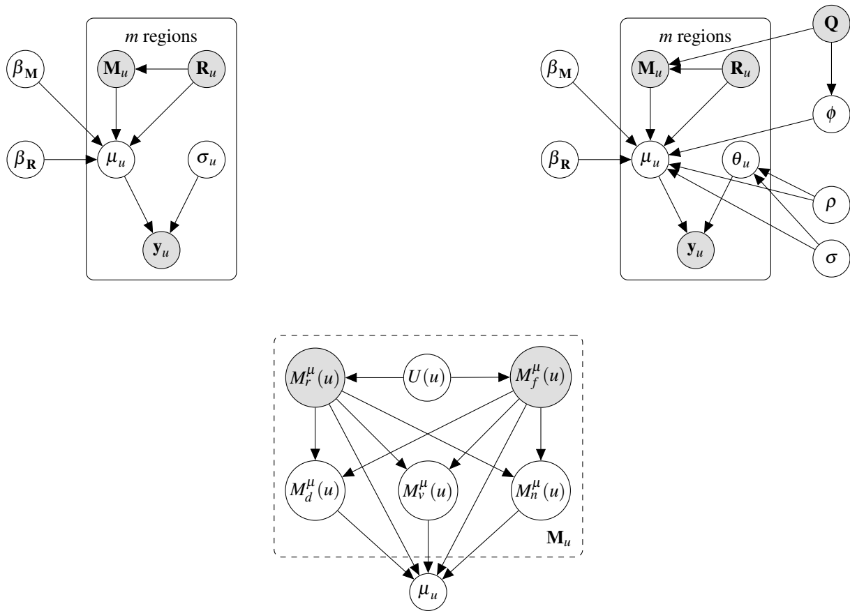
Fig. S5. Graphical representation for vaccine uptake models. Observed variables are shaded gray, latent variables are colored white, and hyperparameters are excluded for clarity. (Top left) The non-spatial model considers every region’s vaccine uptake rate \mathbf{y} as an independent outcome conditioned on the MIST scores \mathbf{M} , while controlling for regional covariates \mathbf{R} that are expected to confound the effect of \mathbf{M} on \mathbf{y} : see Eq. 15. (Top right) The spatial model allows for structured random effects \phi conditioned on regional adjacency matrix \mathbf{Q} , thus controlling for regional adjacency that is expected to confound the effect of \mathbf{M} on \mathbf{y} : see Eq. 17. (Bottom) Analyzing the dependency structure of MIST scores, the dominance of MIST scores in determining vaccine uptake, and the multicollinearity between pairs of MIST scores, reveals that the regional expectation of real and fake news detection ability scores ( M_r^\mu, M_f^\mu ) completely determine the regional expectations of remaining MIST scores: see Supplementary methods: Predicting regional outcomes from MIST scores . Thus, models determining the effect of regional misinformation susceptibility on regional vaccine uptake use M_r^\mu, M_f^\mu as the (exogenous) MIST predictors—eliminating confounding due to underlying common causes of susceptibility U .
