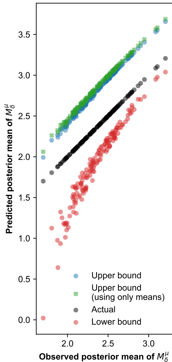
Fig. S14. Regional expectation of real and fake news detection ability scores explain all variation in regional expectation of distrust and naivety bias scores. x -axis indicates the observed posterior means of the poststratified expectation of M_{\delta}^{\mu} = |M_r^{\mu} - M_f^{\mu}| , and y -axis indicates the bounds on M_{\delta}^{\mu} from Eq. S28 (lower and upper bounds) and from Eq. S31 (upper bound using only means/expectations). The upper bound using only the expectations explains all the variation in M_{\delta}^{\mu} ( R^2 = 0.997 ), i.e. from Eq. S32 the regional expectation of real and fake news detection ability scores explain all variation in the regional expectation of bias scores.
