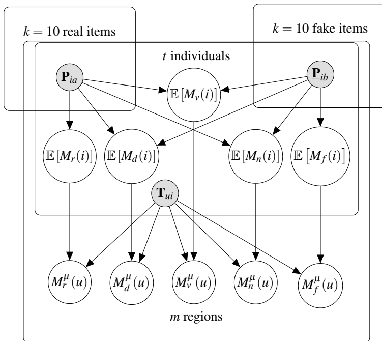
Fig. S4. Graphical representation for poststratifying MIST scores to the region level. The expectation of the misinformation susceptibility test (MIST) scores of an individual is given by the probabilities \mathbf{P}/\underline{\mathbf{P}} of correctly identifying real/fake news headlines, conditioned on the individual's socio-demographics and region of residence: see Eq. 10. The counts \mathbf{T} of people in a given region with a given socio-demographic coordinate can be used to poststratify the expectation of MIST scores to the region level: see Eq. 13.
