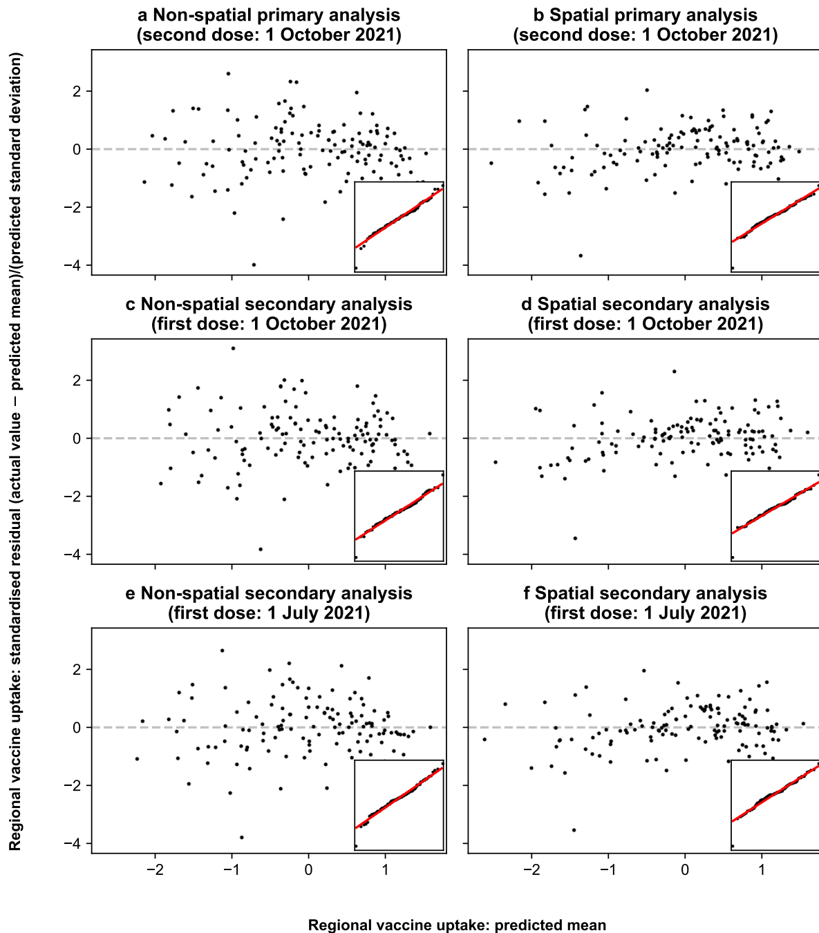
Fig. S22. Posterior means of standardised residuals of vaccine uptake for different vaccine uptake models. Primary analyses considered second dose uptake as of 1 October 2021 ( a, b ), while secondary analyses considered first dose uptake as of 1 October 2021 ( c, d ) and 1 July 2021 ( e, f ), both before ( a, c, e ) and after ( b, d, f ) controlling for spatial effects of regional adjacency. All models include regional real and fake news detection ability scores as predictors, while controlling for a set of regional covariates. Main plots show the posterior mean of the standardised residuals (on the y -axis) against the posterior mean of the outcome (on the x -axis)—we observe no apparent trend in the residuals suggesting homoscedasticity. Inset plots show the quantile-quantile plot for the standard normal distribution on the x -axis and for the (posterior mean of) standardised residuals on the y -axis, with the reference line in red—we observe a good fit suggesting that residuals are normally distributed.
