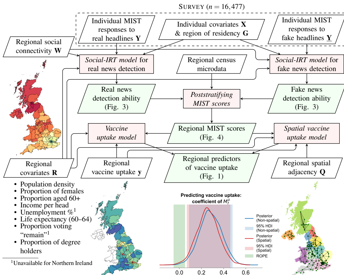
Fig. S1. Overview of the study and statistical modeling. A large-sample ( n = 16,477 ) nationally representative survey was used to test whether misinformation susceptibility, as measured by the psychometrically validated misinformation susceptibility test (MIST [S22, S23]), informs actual COVID-19 vaccine uptake at the region level of grouped NUTS-3 regions in the United Kingdom (UK). Given the survey responses, “social” item response theory (IRT) models inferred latent abilities of individuals to correctly identify (1) real and (2) fake news items, conditioned on a large set of individual and regional covariates (Fig. 3), and the online social connectivity volumes between regions. These two abilities define five “MIST scores” that measure different dimensions of misinformation susceptibility; census microdata were used to aggregate scores to the region level via poststratification [S14] (Fig. 4). Regional MIST scores were then used as predictors for uptake rates of the second dose of a COVID-19 vaccine in England and Scotland to test the primary hypotheses (Fig. 1) by considering the highest posterior density intervals (HPDI) of the coefficients against a preregistered region of practical equivalence (ROPE) to null effects [S24]. While this study was not designed to measure causal effects, a large set of potential region-level confounders were controlled for, including spatial autocorrelations, that ensures the robustness of results.
