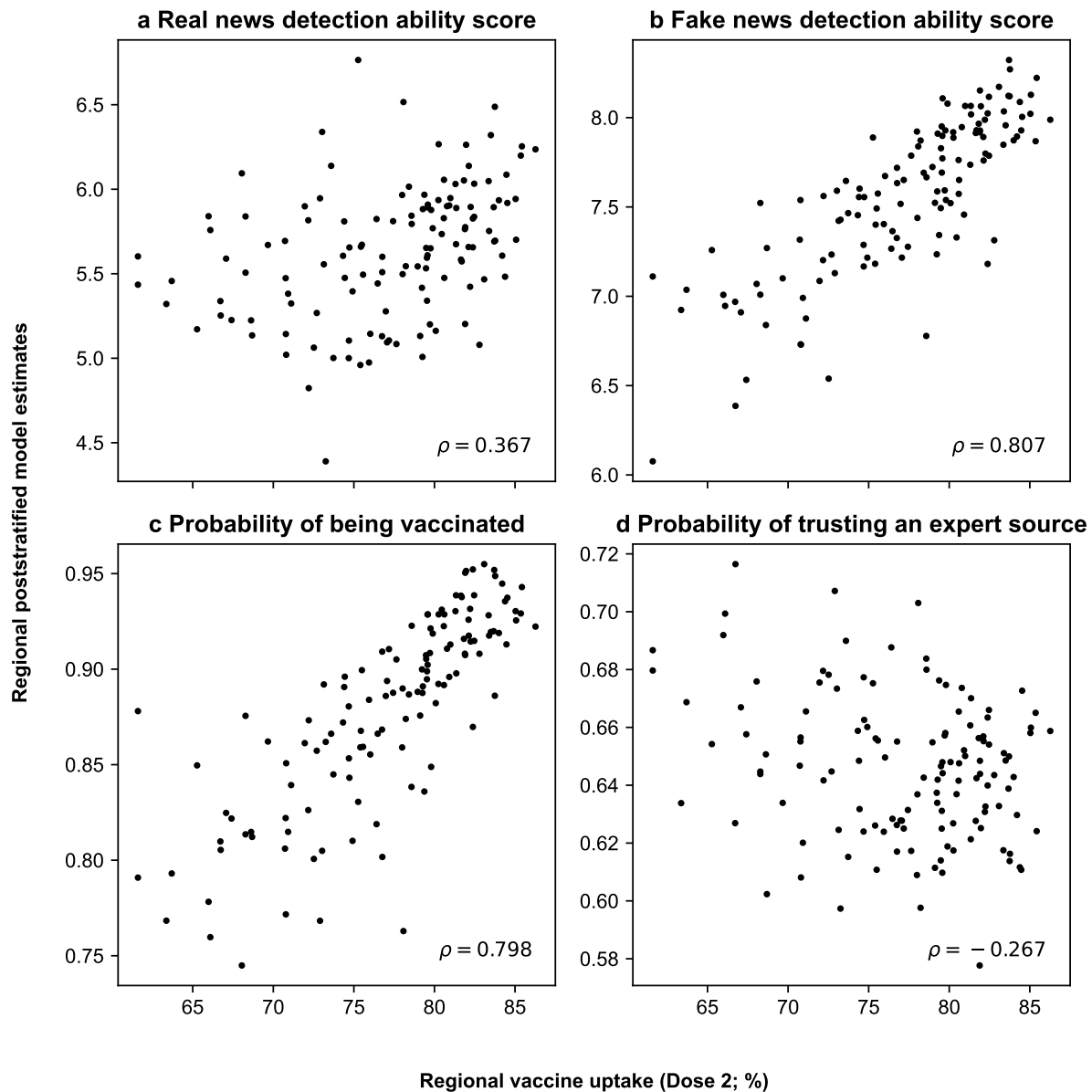
Fig. S18. Bivariate relationship of regional vaccine uptake with regional poststratified model estimates of various key statistics. x -axis indicates observed regional COVID-19 vaccine uptake rates across 129 regions of England and Scotland [S37], while y -axis indicates regional poststratified model estimates of key statistics: real ( M_r^H ; a ) and fake ( M_f^H ; b ) news detection ability scores, the probability of being vaccinated as derived from self-reported vaccination status ( c ; see Questionnaire ), and the probability of trusting an expert source of COVID-19 information ( d ; see Fig. S16). Pearson's correlation coefficient is indicated in the bottom-right of each sub-panel. Evidently, there is a strong positive relationship between self-reported and actual uptake rates ( b ) and fake news detection ability scores and actual uptake rates ( c ).
