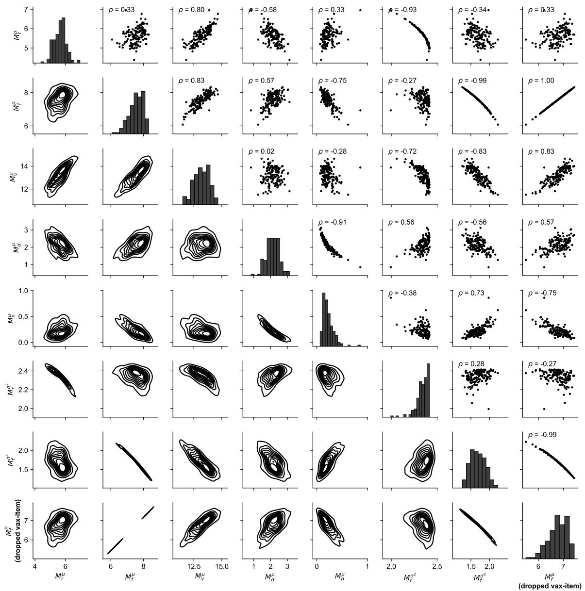
Fig. S12. Bivariate relationships of regional MIST statistics in the United Kingdom. Markers indicate posterior means of poststratified estimates of pairs of statistics for every region, with contours indicating bivariate joint densities and bar plots indicating univariate marginal distributions. Poststratified expectation (variance) of MIST scores is computed from Eq. 13 (Eq. S29). The last row and column correspond to the expected fake news detection ability score computed after dropping the vaccine-specific fake news item (see MIST_6 in Questionnaire ) from the summation in Eq. 13b; its near perfect correlation with the original expected fake news detection ability score indicates robustness of the MIST to individual items. See Table S13 for more details on multicollinearity when predicting vaccine uptake rates from MIST scores.
