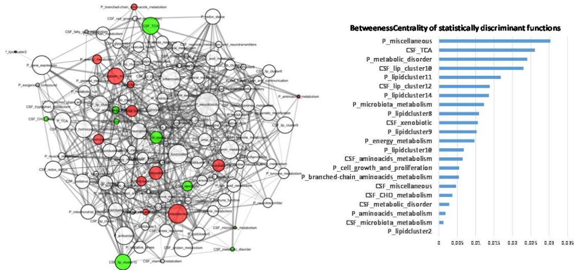
Figure 4. Minimum pairwise partial correlation network integrating all the metabolic functions and lipid clusters in DCI+ patients, and cleaned up from the edges of DCI- patients. The significant functions and clusters of Figure 4 are mapped in the network, with red nodes for plasma and green nodes for cerebrospinal fluid. Edge size is proportional to the p -value of the pairwise relationships. Node size relates to the value of the betweenness centrality coefficients calculated in Cytoscape. These coefficients used for selection of the 22 significant nodes are also reported in decreasing order in the right insight.
