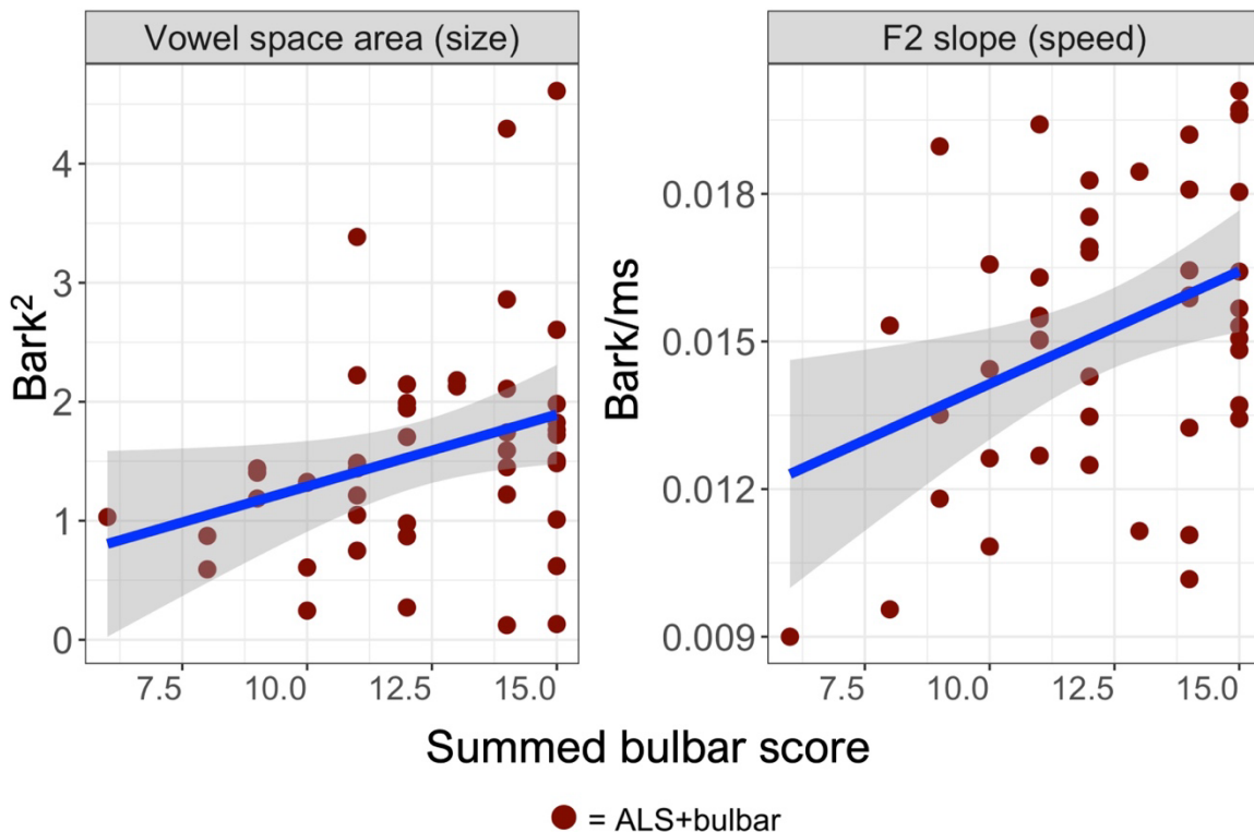
Figure 2. Worse bulbar disease (lower summed bulbar scores composed of ALSFRS-r bulbar and PUMNs bulbar scores) is significantly associated with smaller vowel space area and shallower F2 slopes in ALS+bulbar patients.
