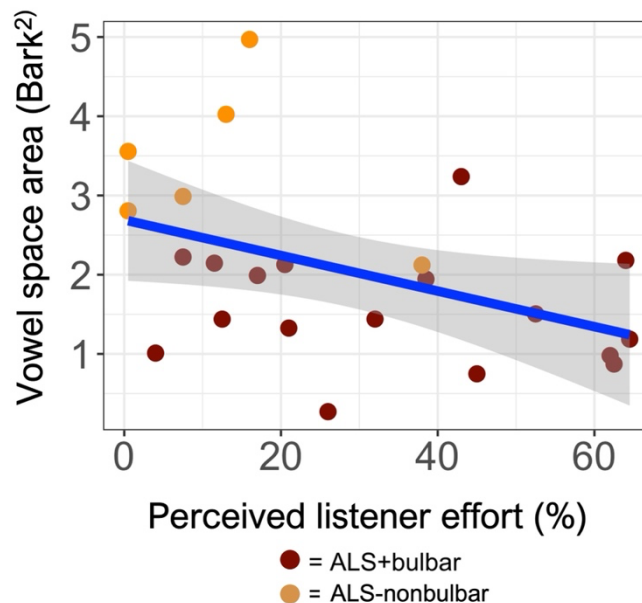
Figure 3. Greater perceived listener effort is significantly associated with smaller vowel space area in ALS.
