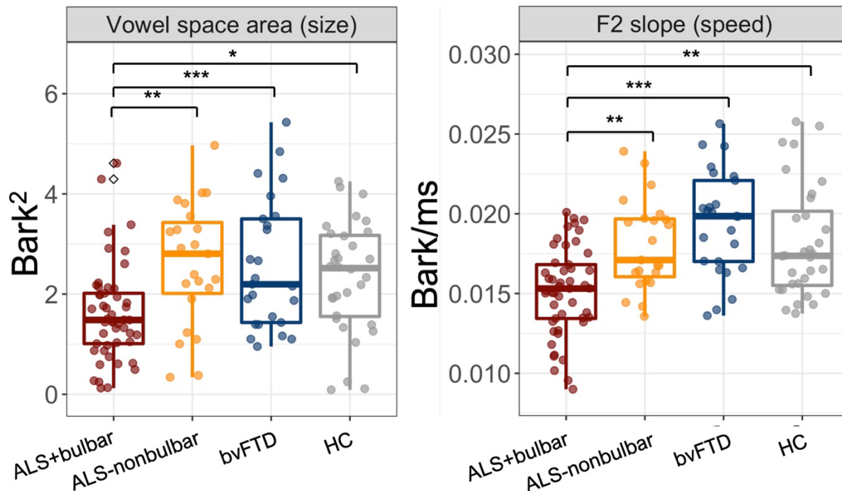
Figure 1. Vowel space area (measure of tongue movement size) and mean F2 slope (measure of speed) are significantly reduced in ALS patients with bulbar motor disease (ALS+bulbar) compared to ALS patients without bulbar disease (ALS-nonbulbar), behavioural variant frontotemporal dementia (bvFTD), and healthy controls (HC). All other contrasts were non-significant, p > 0.05 . * = p < 0.05 , ** = p < 0.01 , *** = p < 0.001 ; Tukey's adjusted HSD.
