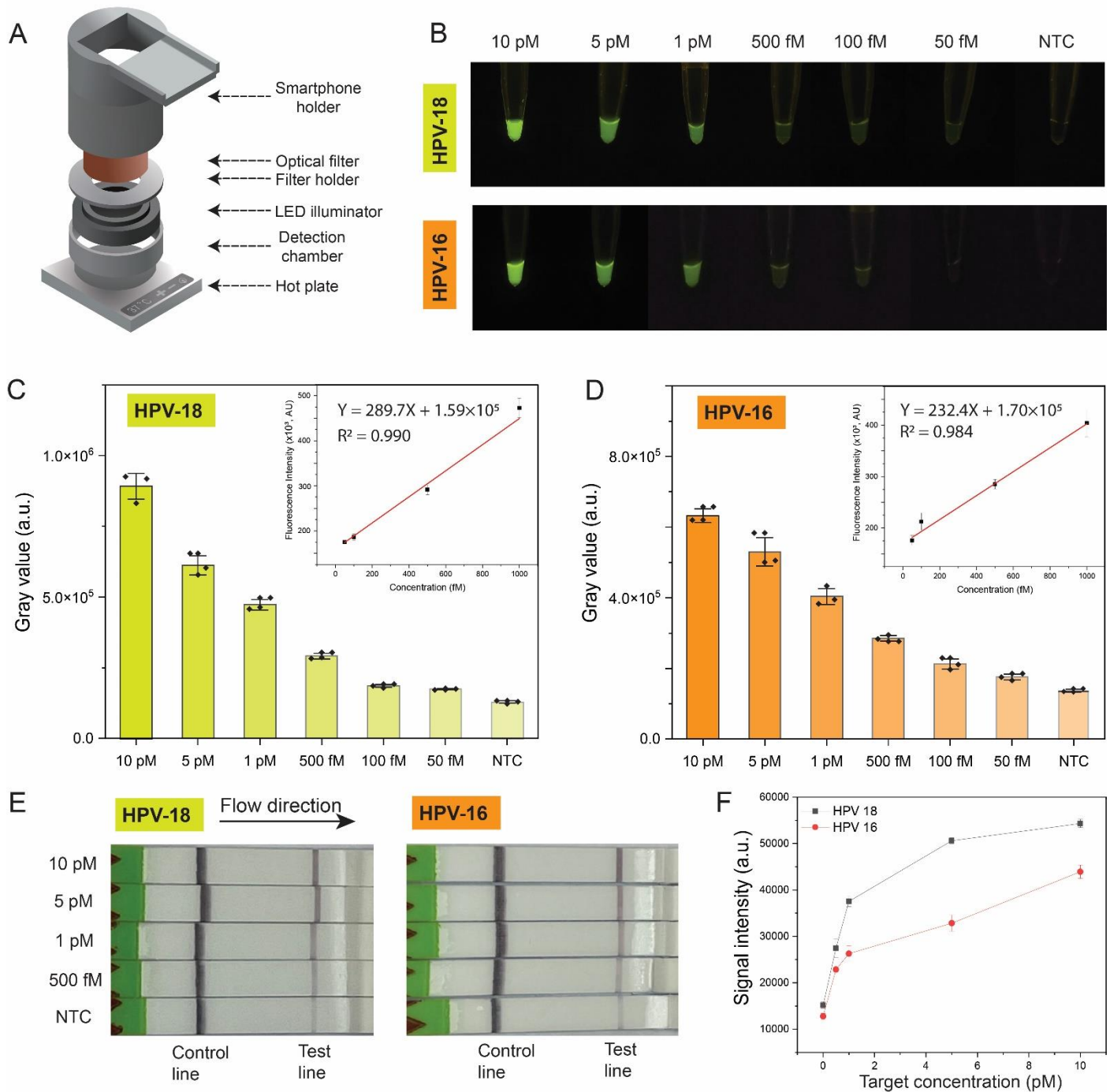
Fig. 6. SPEEDi-CRISPR assay for point-of-care testing. (A) The exploded view of a portable home-made device assembled with an optical filter, the 3D-printed body parts, a blue LED illuminator, and a consumer digital hotplate. (B) Representative fluorescence images of two HPV targets at variable concentrations (10 pM, 5 pM, 1 pM, 500 fM, 100 fM, 50 fM, and NTC) captured by the smartphone. (C-D) Quantitative analyses and calibration curves for the detection of HPV-18 (C) and HPV-16 (D) using the portable device-coupled SPEEDi-CRISPR assay. The grayscale analysis of the fluorescence signal in each tube is achieved by ImageJ. The LoD was determined by 3\sigma rule (47.0 fM for HPV-18 and 48.3 fM for HPV-16). Error bars: one S.D. ( n = 3 or 4). (E) Representative photos of LFA assay for two HPV targets at variable concentrations (10 pM, 5 pM, 1 pM, 500 fM, and NTC). (F) Measurements of test line band intensity for HPV-18 (black) and HPV-16 (red) by ImageJ. Error bar: one S.D. ( n = 2 ).
