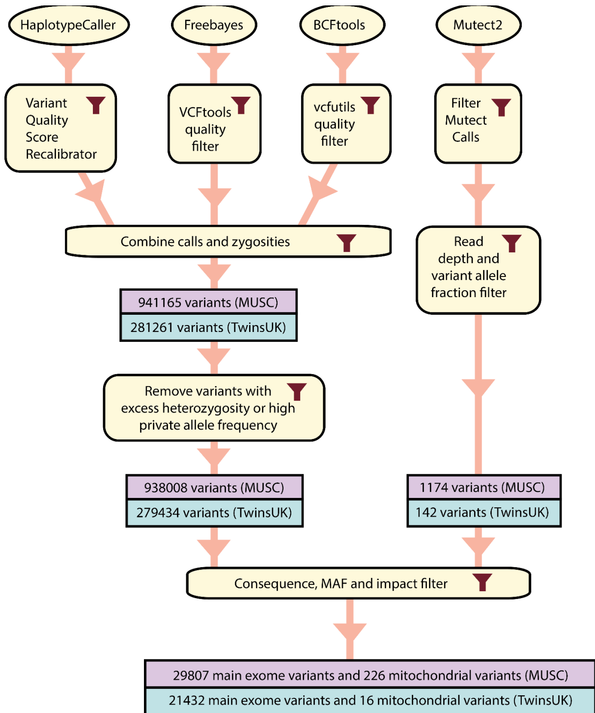
Suppl. Figure 3. Flow chart showing the variant filtering pipeline. See Suppl. Table 2 for details of the filter settings.
