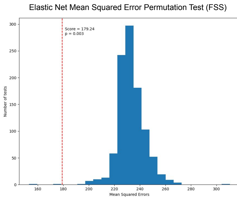
Figure S3: Null distribution (based on mean squared error, MSE) for the elastic net regression model predicting FSS fatigue scores ( N=62 ) from all 15 measurements. Dashed red line shows the MSE of the unpermuted prediction. Blue bars show the MSE distribution ( N=999 ) when permuting scores.
