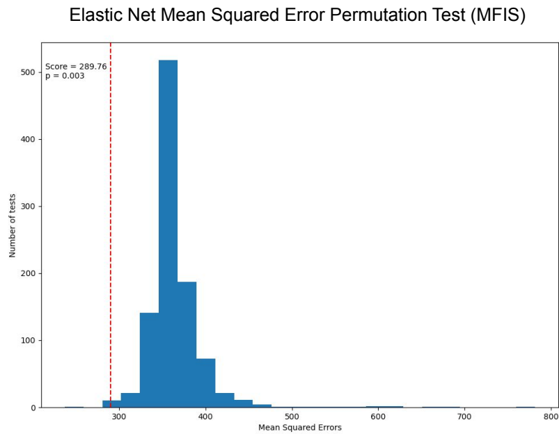
Figure S2: Null distribution (based on mean squared error, MSE) for the elastic net regression model predicting MFIS fatigue scores ( N=52 ) from all 15 measurements. Dashed red line shows the MSE of the unpermuted prediction. Blue bars show the MSE distribution ( N=999 ) when permuting scores.
