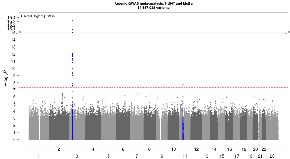
Supplementary Figure 1: Manhattan plot [arsenic]: Novel (blue) genetic loci (index variant \pm 500 kilobase pairs) associated with whole blood arsenic concentrations at genome-wide significance ( p\text{-value} < 5 \times 10^{-8} , threshold indicated by red dotted line) in HUNT and MoBa. Genetic variants plotted according to chromosome and position (x-axis) and the -\log_{10}(p\text{-value}) for the variant-arsenic level association (y-axis). Sample size N=5591 . HUNT=The Trøndelag Health Study. MoBa=The Norwegian Mother, Father, and Child Cohort Study.
