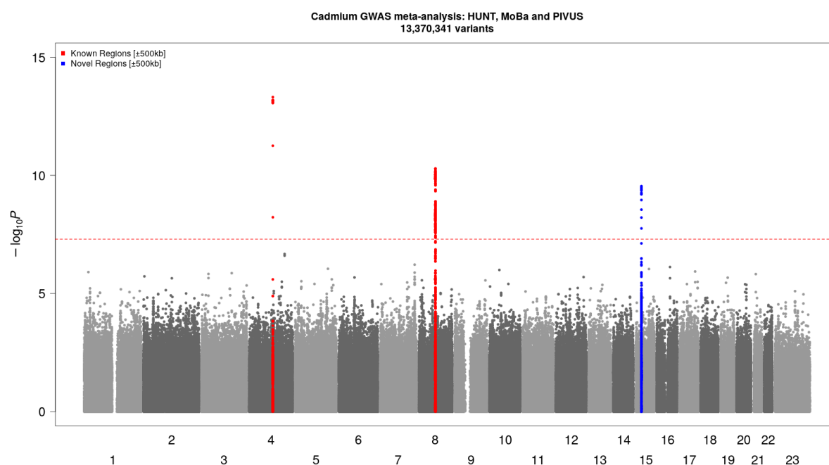
Supplementary Figure 3: Manhattan plot [cadmium]: Novel (blue) and known (red) genetic loci (index variant \pm 500 kilobase pairs) associated with whole blood cadmium concentrations at genome-wide significance ( p\text{-value} < 5 \times 10^{-8} , threshold indicated by red dotted line) in HUNT, MoBa and PIVUS. Genetic variants plotted according to chromosome and position (x-axis) and the -\log_{10}(p\text{-value}) for the variant-cadmium level association (y-axis). Sample size N=6542 . HUNT=The Trøndelag Health Study. MoBa=The Norwegian Mother, Father, and Child Cohort Study. PIVUS=The Prospective Investigations of the Vasculature in Uppsala Seniors study.
