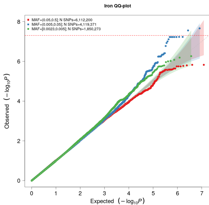
Supplementary Figure 22: QQ plot [iron]: The expected -\log_{10}(p\text{-value}) given no true associations are given on the x-axis, and the observed -\log_{10}(p\text{-value}) from the GWAS of iron concentrations in HUNT are given on the y-axis, stratified by minor allele frequency (MAF) categories: Common ( MAF > 0.05 ) variants (red), low-frequency ( 0.005 < MAF < 0.05 ) variants (blue) and rare ( MAF < 0.005 ) variants (green). HUNT=The Trøndelag Health Study.
