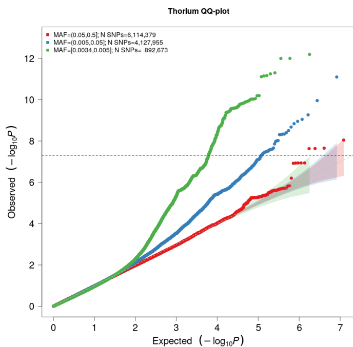
Supplementary Figure 45: QQ plot [thorium (excluded)]: The expected -\log_{10}(p -value) given no true associations are given on the x-axis, and the observed -\log_{10}(p -value) from the GWAS of thorium concentrations in HUNT are given on the y-axis, stratified by minor allele frequency (MAF) categories: Common ( MAF > 0.05 ) variants (red), low-frequency ( 0.005 < MAF < 0.05 ) variants (blue) and rare ( MAF < 0.005 ) variants (green). Deviations from the expected values at small -\log_{10}(p -values) indicate highly inflated test statistics for low-frequency and rare variants. HUNT=The Trøndelag Health Study.
