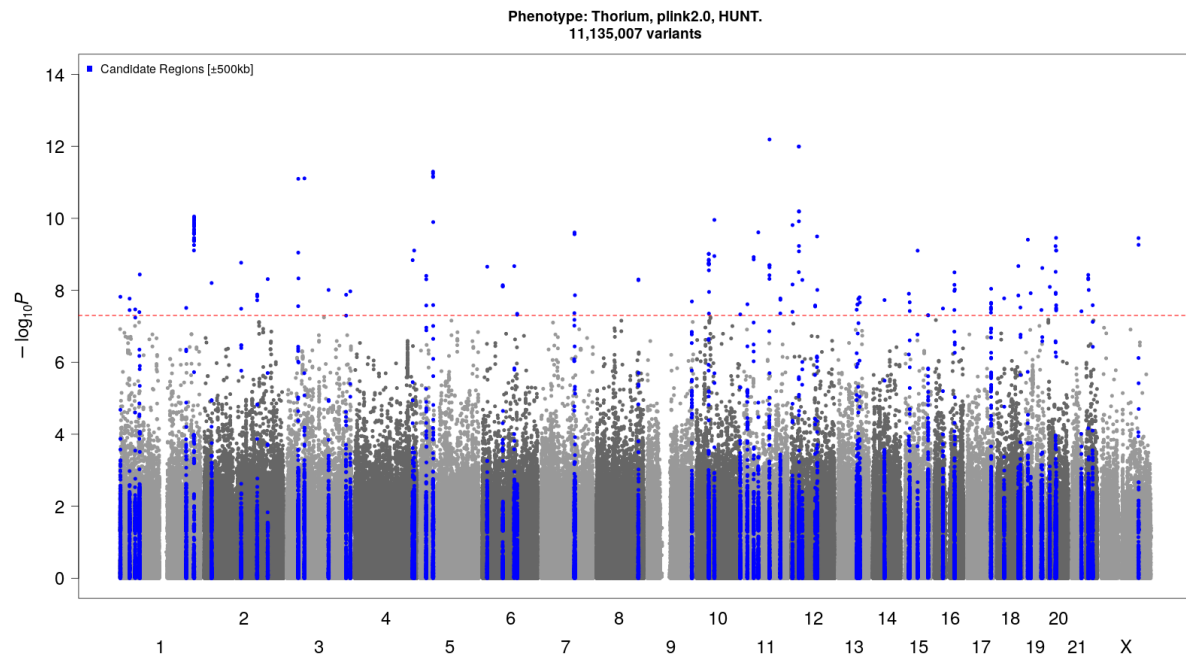
Supplementary Figure 44: Manhattan plot [thorium (excluded)]: Inflated test statistics of thorium concentrations give a high number of apparently associated (index variant \pm 500 kilobase pairs) genetic loci at genome-wide significance ( p -value < 5 \times 10^{-8} , threshold indicated by red dotted line) in HUNT, and the results were therefore excluded. Genetic variants plotted according to chromosome and position (x-axis) and the -\log_{10}(p -value) for the variant-thorium level association (y-axis). Sample size N=1479 . HUNT=The Trøndelag Health Study.
