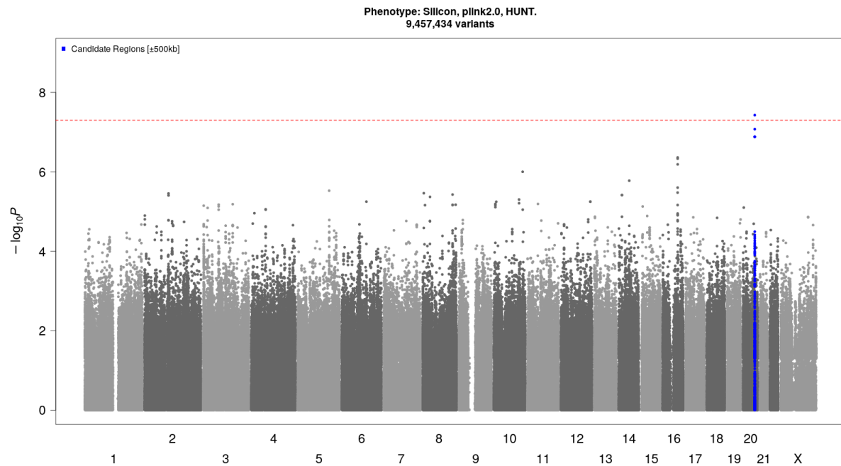
Supplementary Figure 27: Manhattan plot [silicon]: Novel (candidate) genetic loci (index variant \pm 500 kilobase pairs) associated with whole blood silicon concentrations at genome-wide significance ( p -value < 5 \times 10^{-8} , threshold indicated by red dotted line) in HUNT. Genetic variants plotted according to chromosome and position ( x -axis) and the -\log_{10}(p -value) for the variant-silicon level association ( y -axis). Sample size N=688 . HUNT=The Trøndelag Health Study.
