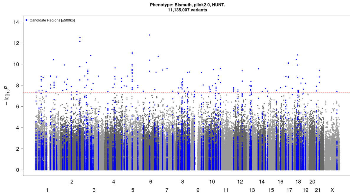
Supplementary Figure 42: Manhattan plot [bismuth (excluded)]: Inflated test statistics of bismuth concentrations give a high number of apparently associated (index variant \pm 500 kilobase pairs) genetic loci at genome-wide significance ( p -value < 5 \times 10^{-8} , threshold indicated by red dotted line) in HUNT, and the results were therefore excluded. Genetic variants plotted according to chromosome and position (x-axis) and the -\log_{10}(p -value) for the variant-bismuth level association (y-axis). Sample size N=1539 . HUNT=The Trøndelag Health Study.
