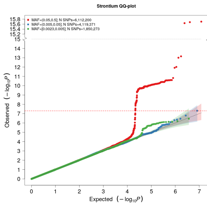
Supplementary Figure 32: QQ plot [strontium]: The expected -\log_{10}(p\text{-value}) given no true associations are given on the x-axis, and the observed -\log_{10}(p\text{-value}) from the GWAS of strontium concentrations in HUNT are given on the y-axis, stratified by minor allele frequency (MAF) categories: Common ( MAF > 0.05 ) variants (red), low-frequency ( 0.005 < MAF < 0.05 ) variants (blue) and rare ( MAF < 0.005 ) variants (green). HUNT=The Trøndelag Health Study.
