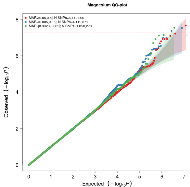
Supplementary Figure 24: QQ plot [magnesium]: The expected -\log_{10}(p\text{-value}) given no true associations are given on the x-axis, and the observed -\log_{10}(p\text{-value}) from the GWAS of magnesium concentrations in HUNT are given on the y-axis, stratified by minor allele frequency (MAF) categories: Common ( MAF > 0.05 ) variants (red), low-frequency ( 0.005 < MAF < 0.05 ) variants (blue) and rare ( MAF < 0.005 ) variants (green). HUNT=The Trøndelag Health Study.
