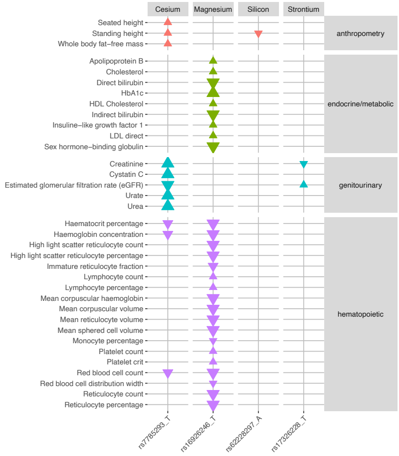
Supplementary Figure 41: Phenome-wide associations between index variants from GWAS in HUNT and phecodes, continuous traits and biomarkers in the UK Biobank. Each triangle represents a statistically significant ( p\text{-value} < 9.7 \times 10^{-7} ) association between an index variant from trace element GWASs in HUNT (x-axis, grouped by trace element) and an outcome in the UK Biobank (y-axis, grouped and colored according to biological domain). Larger triangles represent lower p-values, and the direction indicates if the direction of effect for the indicated allele is the same (up) or opposite (down) as the association with the trace element.
