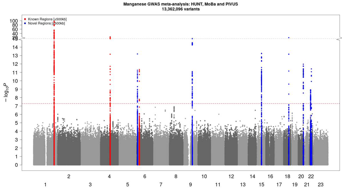
Supplementary Figure 9: Manhattan plot [manganese]: Novel (blue) and known (red) genetic loci (index variant \pm 500 kilobase pairs) associated with whole blood manganese concentrations at genome-wide significance ( p\text{-value} < 5 \times 10^{-8} , threshold indicated by red dotted line) in HUNT, MoBa and PIVUS. Genetic variants are plotted according to chromosome and position (x-axis) and the -\log_{10}(p\text{-value}) for the variant-manganese level association (y-axis). Sample size N=6564 . HUNT=The Trøndelag Health Study. MoBa=The Norwegian Mother, Father, and Child Cohort Study. PIVUS=The Prospective Investigations of the Vasculature in Uppsala Seniors study.
