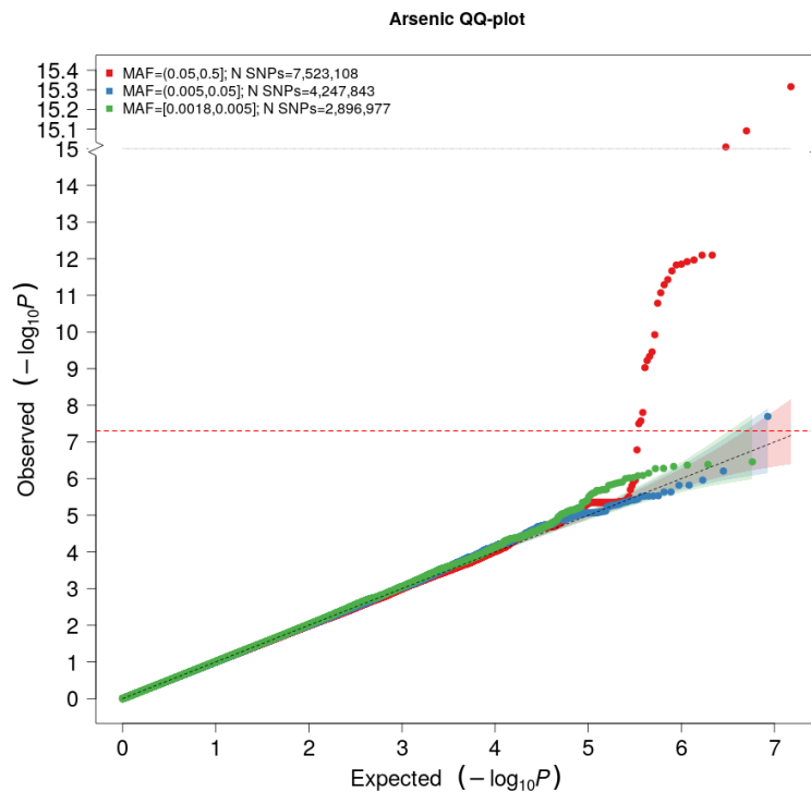
Supplementary Figure 2: QQ plot [Arsenic]: The expected -\log_{10}(p\text{-value}) given no true associations are given on the x-axis, and the observed -\log_{10}(p\text{-value}) from the GWA meta-analysis of arsenic concentrations in HUNT and MoBa are given on the y-axis, stratified by minor allele frequency (MAF) categories: Common ( \text{MAF} > 0.05 ) variants (red), low-frequency ( 0.005 < \text{MAF} < 0.05 ) variants (blue) and rare ( \text{MAF} < 0.005 ) variants (green). HUNT=The Trøndelag Health Study. MoBa=The Norwegian Mother, Father, and Child Cohort Study.
