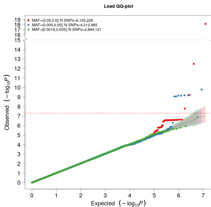
Supplementary Figure 8: QQ plot [lead]: The expected -\log_{10}(p -value) given no true associations are given on the x-axis, and the observed -\log_{10}(p -value) from the GWA meta-analysis of lead concentrations in HUNT, MoBa and PIVUS are given on the y-axis, stratified by minor allele frequency (MAF) categories: Common (MAF > 0.05 ) variants (red), low-frequency ( 0.005 < \text{MAF} < 0.05 ) variants (blue) and rare (MAF < 0.005 ) variants (green). HUNT=The Trøndelag Health Study. MoBa=The Norwegian Mother, Father, and Child Cohort Study. PIVUS=The Prospective Investigations of the Vasculature in Uppsala Seniors study.
