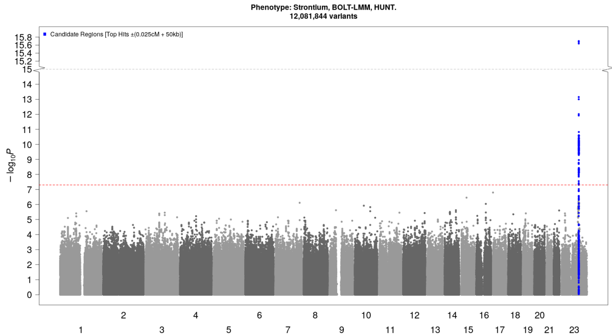
Supplementary Figure 31: Manhattan plot [strontium]: Novel (candidate) genetic loci (index variant \pm 500 kilobase pairs) associated with whole blood strontium concentrations at genome-wide significance ( p\text{-value} < 5 \times 10^{-8} , threshold indicated by red dotted line) in HUNT. Genetic variants plotted according to chromosome and position (x-axis) and the -\log_{10}(p\text{-value}) for the variant-strontium level association (y-axis). Sample size N=2197 . HUNT=The Trøndelag Health Study.
