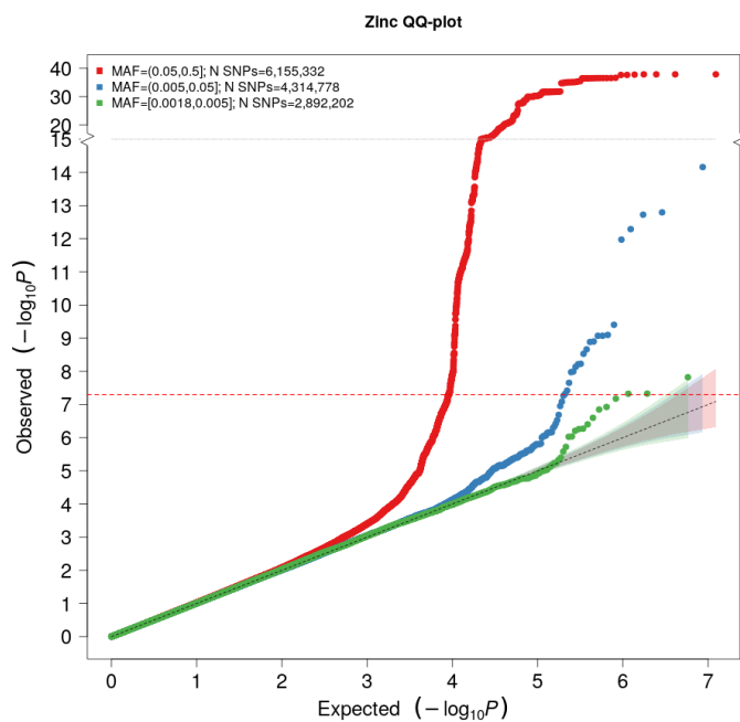
Supplementary Figure 14: QQ plot [zinc]. The expected -\log_{10}(p\text{-value}) given no true associations are given on the x-axis, and the observed -\log_{10}(p\text{-value}) from the GWA meta-analysis of whole blood zinc concentrations in HUNT, MoBa and PIVUS are given on the y-axis, stratified by minor allele frequency (MAF) categories: Common ( MAF > 0.05 ) variants (red), low-frequency ( 0.005 < MAF < 0.05 ) variants (blue) and rare ( MAF < 0.005 ) variants (green). HUNT=The Trøndelag Health Study. MoBa=The Norwegian Mother, Father, and Child Cohort Study. PIVUS=The Prospective Investigations of the Vasculature in Uppsala Seniors study.
