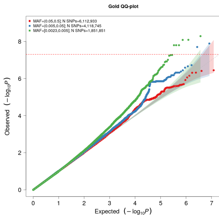
Supplementary Figure 18: QQ plot [gold]. The expected -\log_{10}(p -value) given no true associations are given on the x-axis, and the observed -\log_{10}(p -value) from the GWA meta-analysis of whole blood gold concentrations in HUNT are given on the y-axis, stratified by minor allele frequency (MAF) categories: Common ( MAF > 0.05 ) variants (red), low-frequency ( 0.005 < MAF < 0.05 ) variants (blue) and rare ( MAF < 0.005 ) variants (green). HUNT=The Trøndelag Health Study.
