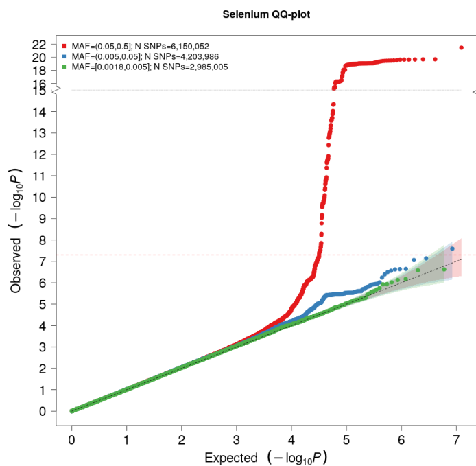
Supplementary Figure 12: QQ plot [selenium]: The expected -\log_{10}(p\text{-value}) given no true associations are given on the x-axis, and the observed -\log_{10}(p\text{-value}) from the GWA meta-analysis of selenium concentrations in HUNT and MoBa are given on the y-axis, stratified by minor allele frequency (MAF) categories: Common ( \text{MAF} > 0.05 ) variants (red), low-frequency ( 0.005 < \text{MAF} < 0.05 ) variants (blue) and rare ( \text{MAF} < 0.005 ) variants (green). HUNT=The Trøndelag Health Study. MoBa=The Norwegian Mother, Father, and Child Cohort Study.
