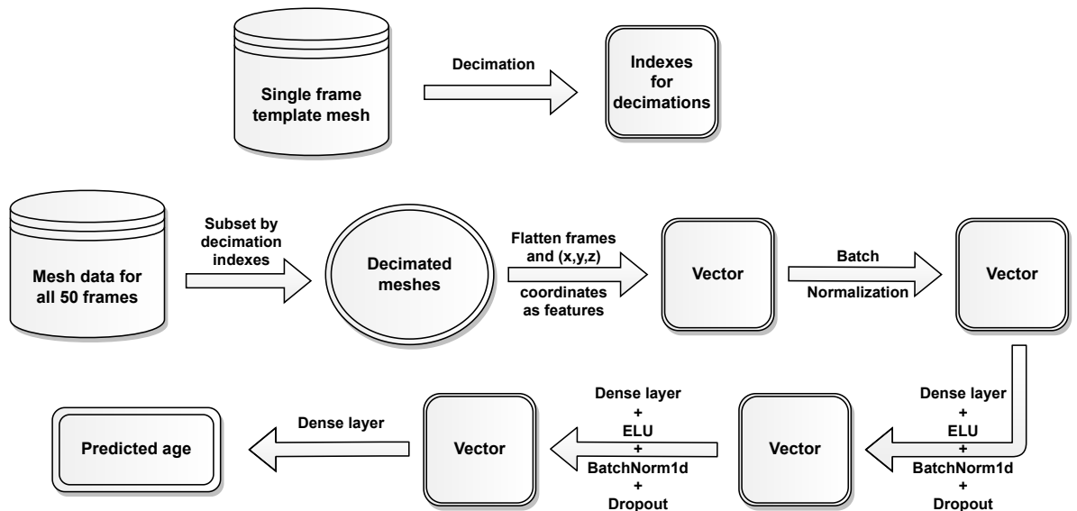
Figure 3. Details of the dense neural network structure.
