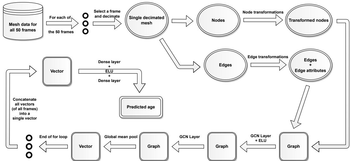
Figure 2. Details of the graph neural network structure, where nodes are transformed using a concatenation of constant, position and FPFH features transformations, while edge attributes are generated as spherical coordinates of the edges.
