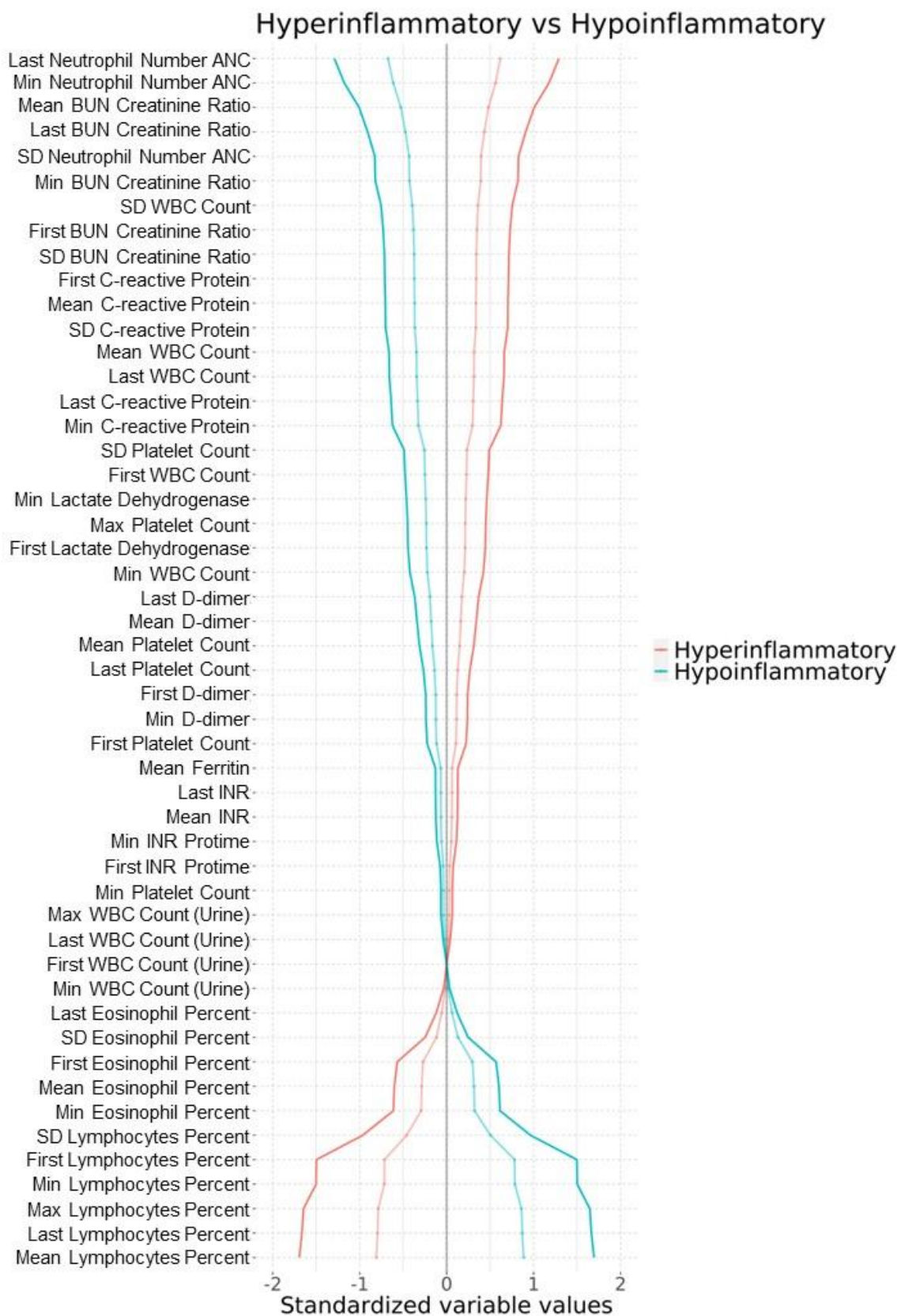
Figure 2: Standardized Variable Plots of Hyper vs Hypoinflammatory Clusters. Standardized mean values are computed by taking the mean of a specific feature in a group and comparing to the mean of another group (solid lines) Faded lines represent comparisons of a cluster to all patients.
