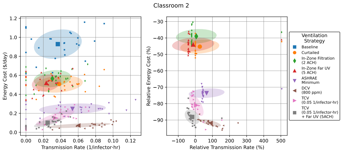
Figure 4: Energy versus transmission rate tradeoffs for hypothetical ventilation scenarios in Classroom 2. Small points show individual daily values, while large points with error bars show mean \pm standard deviation. Right plot is relative to “Baseline” for each day.
