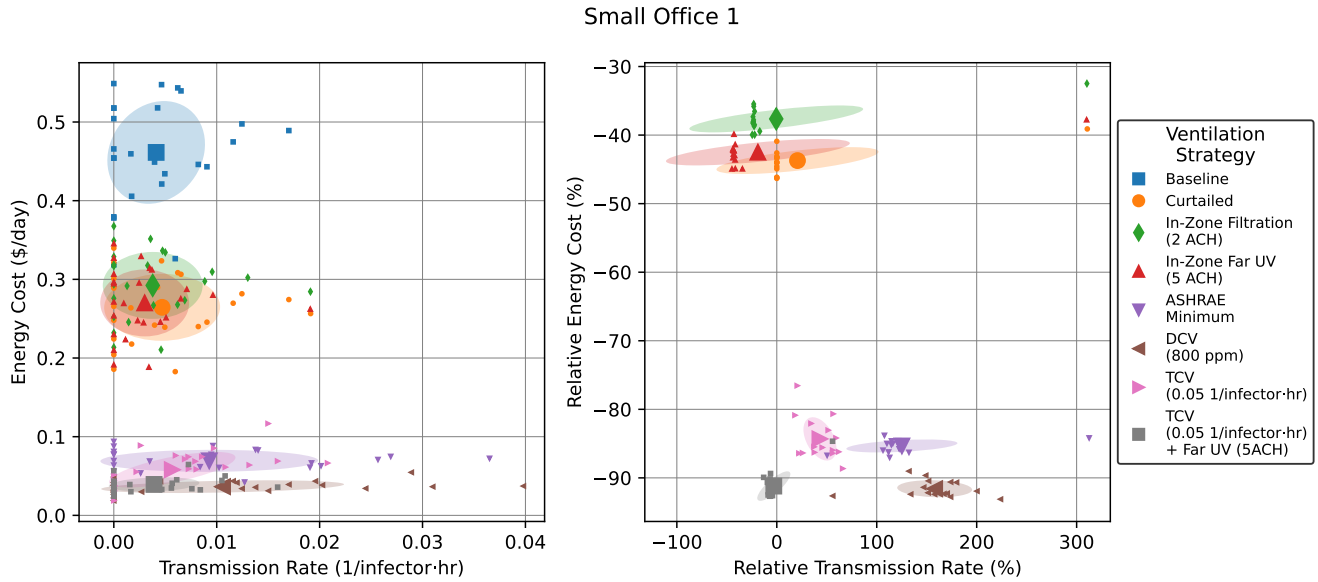
Figure 20: Energy versus transmission rate tradeoffs for hypothetical ventilation scenarios in Small Office 1. Small points show individual daily values, while large points with error bars show mean \pm standard deviation.
