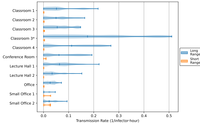
Figure 23: Distributions of short-range and long-range transmission rates in monitored spaces. Short-range rates are calculated from an empirical model based on the results of [9], while long-range rates use the pseudo-steady model from the main paper. As in Figure 5, the distributions are weighted based on the number of occupants in the space at each time point.
