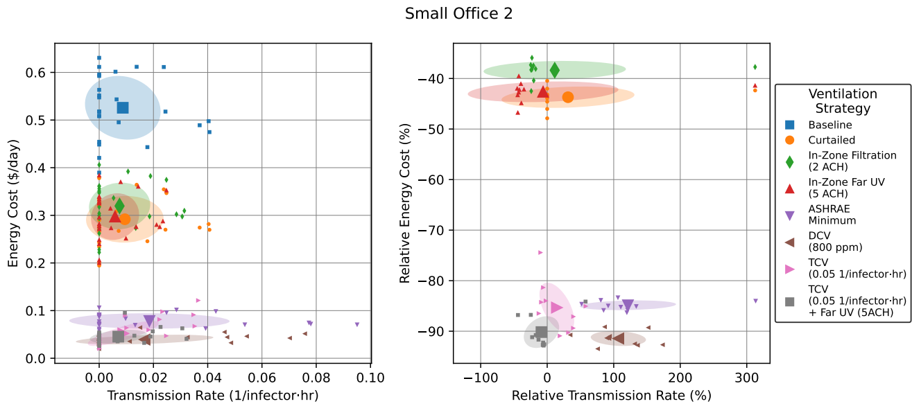
Figure 22: Energy versus transmission rate tradeoffs for hypothetical ventilation scenarios in Small Office 2. Small points show individual daily values, while large points with error bars show mean \pm standard deviation. Right plot is relative to “Baseline” for each day.
