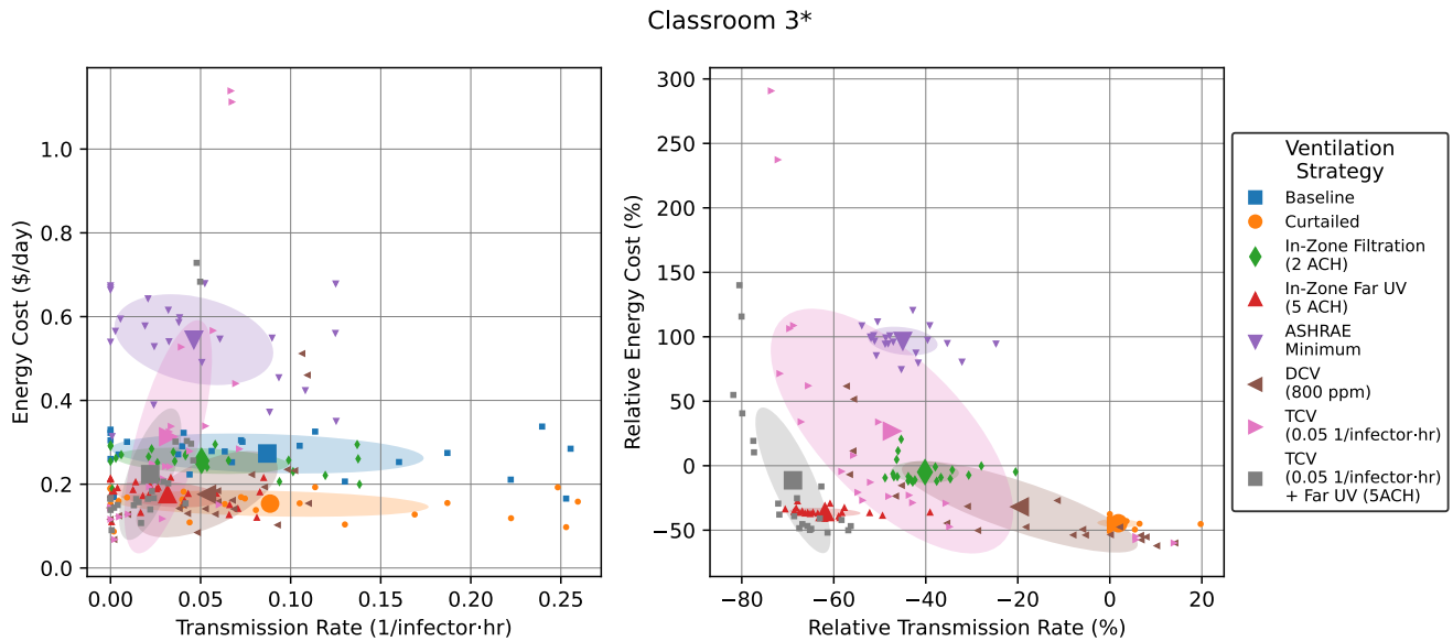
Figure 8: Energy versus transmission rate tradeoffs for hypothetical ventilation scenarios in Classroom 3*. Small points show individual daily values, while large points with error bars show mean \pm standard deviation. Right plot is relative to “Baseline” for each day.
