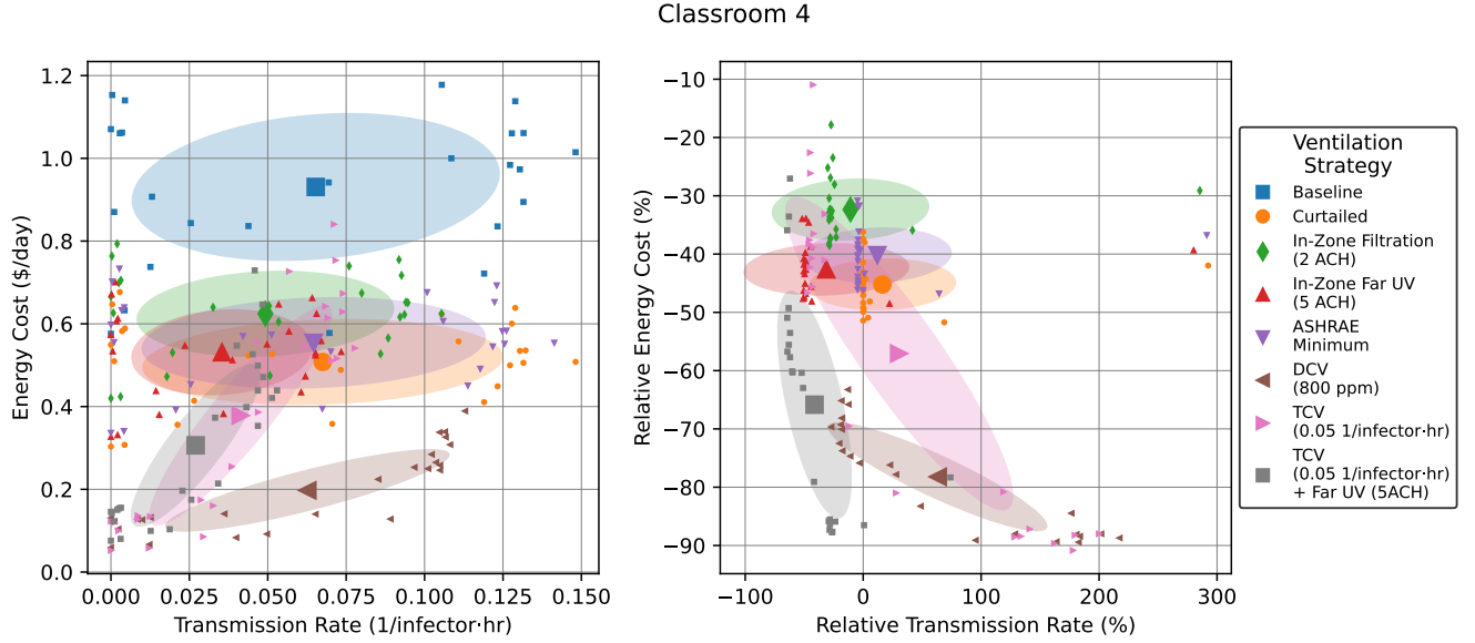
Figure 10: Energy versus transmission rate tradeoffs for hypothetical ventilation scenarios in Classroom 4. Small points show individual daily values, while large points with error bars show mean \pm standard deviation. Right plot is relative to “Baseline” for each day.
