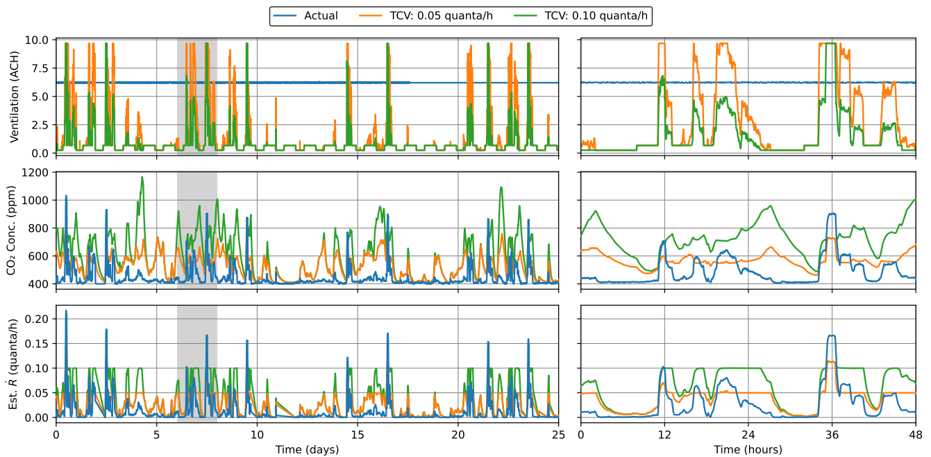
Figure 25: Simulated transmission-controlled ventilation in comparison with actual operation for Classroom 1. The second column shows a zoomed-in view of the gray shaded region in the first column.
