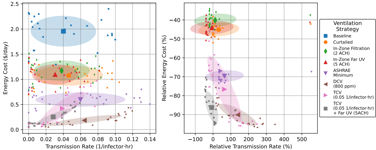
Figure 2: Energy versus transmission rate tradeoffs for hypothetical ventilation scenarios in Classroom 1. Small points show individual daily values, while large points with error bars show mean \pm standard deviation. Right plot is relative to “Baseline” for each day.
