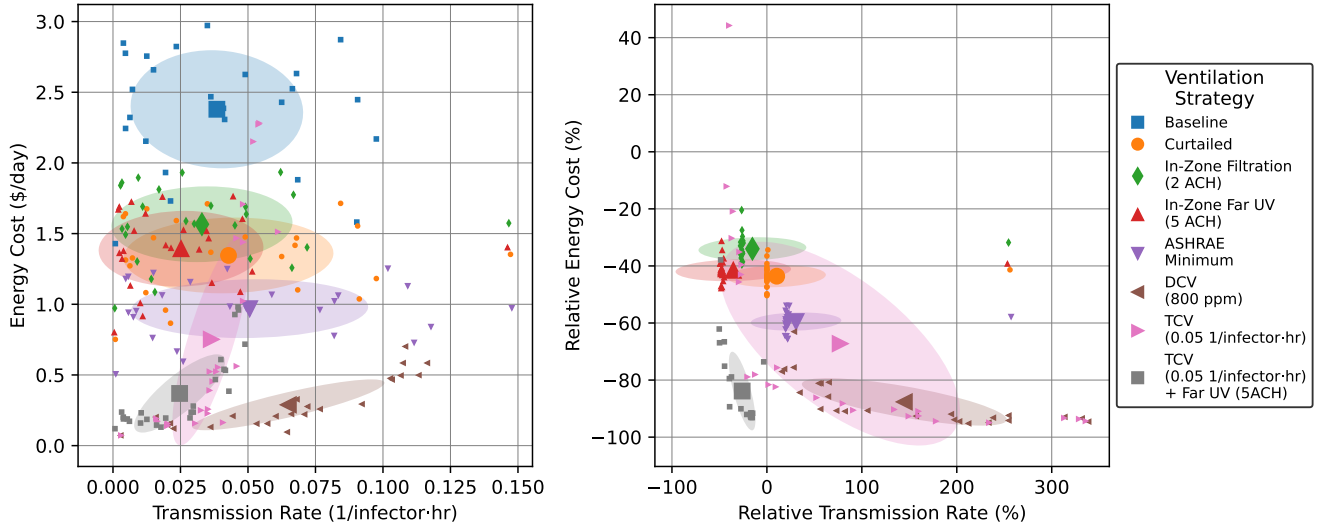
Figure 14: Energy versus transmission rate tradeoffs for hypothetical ventilation scenarios in Lecture Hall 1. Small points show individual daily values, while large points with error bars show mean \pm standard deviation. Right plot is relative to “Baseline” for each day.
