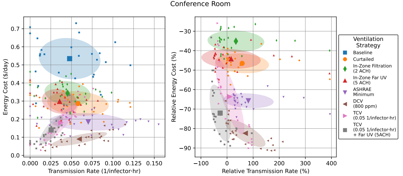
Figure 12: Energy versus transmission rate tradeoffs for hypothetical ventilation scenarios in Conference Room. Small points show individual daily values, while large points with error bars show mean \pm standard deviation. Right plot is relative to “Baseline” for each day.
