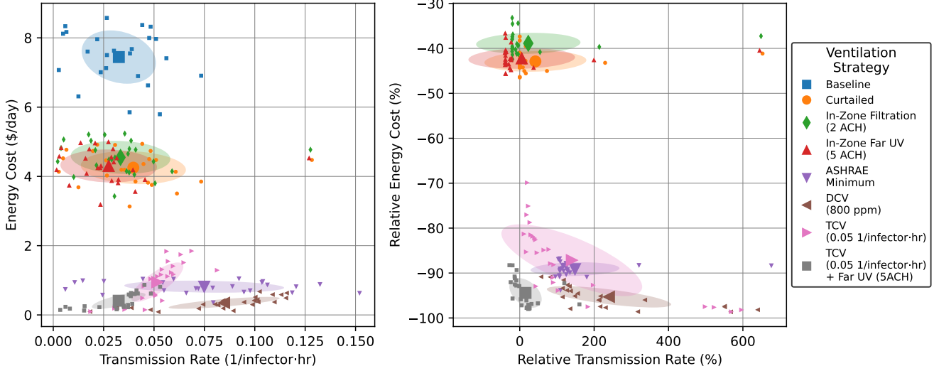
Figure 16: Energy versus transmission rate tradeoffs for hypothetical ventilation scenarios in Lecture Hall 2. Small points show individual daily values, while large points with error bars show mean \pm standard deviation. Right plot is relative to “Baseline” for each day.
