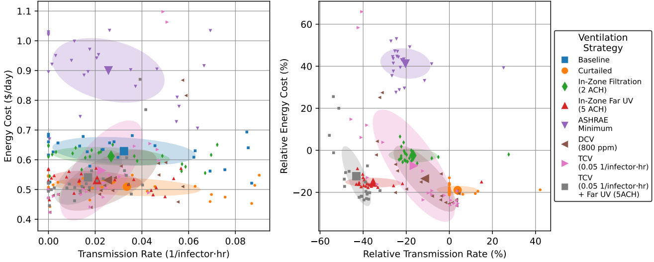
Figure 6: Energy versus transmission rate tradeoffs for hypothetical ventilation scenarios in Classroom 3. Small points show individual daily values, while large points with error bars show mean \pm standard deviation. Right plot is relative to “Baseline” for each day.
