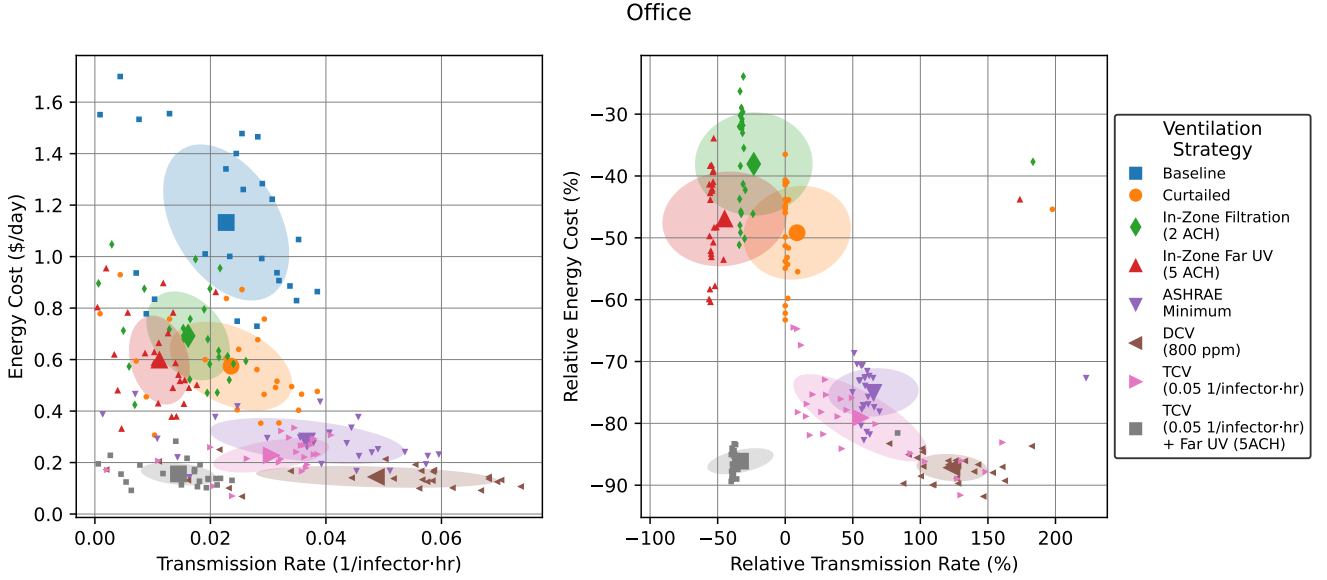
Figure 18: Energy versus transmission rate tradeoffs for hypothetical ventilation scenarios in Office. Small points show individual daily values, while large points with error bars show mean \pm standard deviation. Right plot is relative to “Baseline” for each day.
