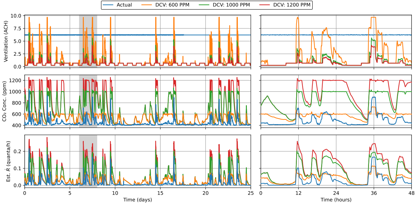
Figure 24: Simulated demand-controlled ventilation in comparison with actual operation for Classroom 1. The second column shows a zoomed-in view of the gray shaded region in the first column.
