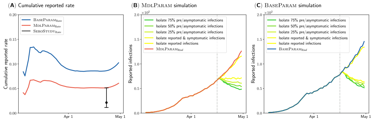
Figure 5: (A) MDLINFER estimates cumulative reported rate more accurately than BASEINFER: The blue and red curve represent the cumulative reported rate estimated by BASEINFER, BASEPARAM Rate , and by MDLINFER, MDLPARAM Rate , respectively. The black point estimate and its confidence interval represent the cumulative reported rate SEROSTUDY Rate estimated by serological studies [2, 26]. Note that both approaches try to fit the SEROSTUDY Rate without being informed with them. The results reveal that a large majority of COVID-19 infections were unreported. (B) MDLINFER reveals that non-pharmaceutical interventions (NPI) on asymptomatic and presymptomatic infections are essential to control the COVID-19 epidemic. Here, the red curve and other five curves represent the MDLINFER’s estimation of reported infections for no NPI scenario and 5 different NPI scenarios described in the Results section. The vertical grey dash line divides the observed period (left) and forecast period (right). (C) Inaccurate estimation by BASEINFER may lead to wrong non-pharmaceutical intervention conclusions. The blue curve and other five curves represent the BASEINFER’s estimation of reported infections for no NPI scenario and the same 5 scenarios in (B).
