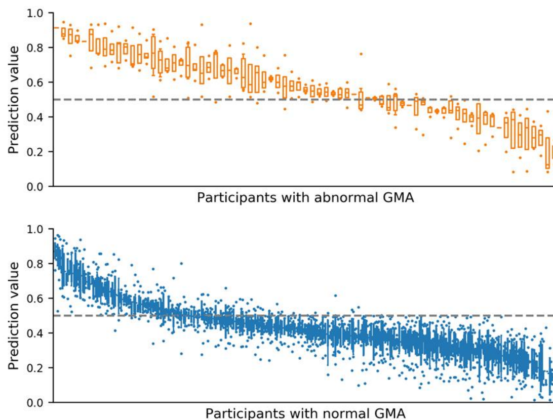
Figure 3: Variation in classifier prediction values. Classifier prediction values from 25-fold cross validation. Prediction values reported when infant movement included in held out test set, ordered by median prediction value. Top (orange) infant videos scored as abnormal/absent general movement assessment (GMA) by expert rater, n=73 infant videos. Bottom (blue) infant videos scored as normal GMA by expert rater, n=396 infant videos. Boxes with horizontal line represent interquartile range and median respectively, error bars represent 95% confidence interval and dots represent outliers. Dashed line at 0.5 represents cut-off value for classifier between abnormal/absent GMA prediction and normal GMA prediction.
