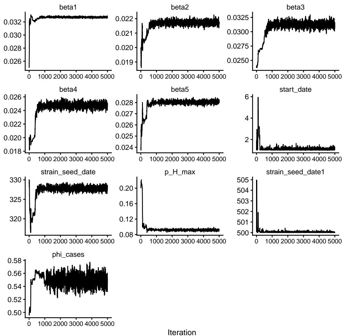
Figure S1: Trace plots for fitted parameters from MCMC. Plots show samples from full chain (50,000 iterations), including the burn-in, thinned by a factor of 10.
