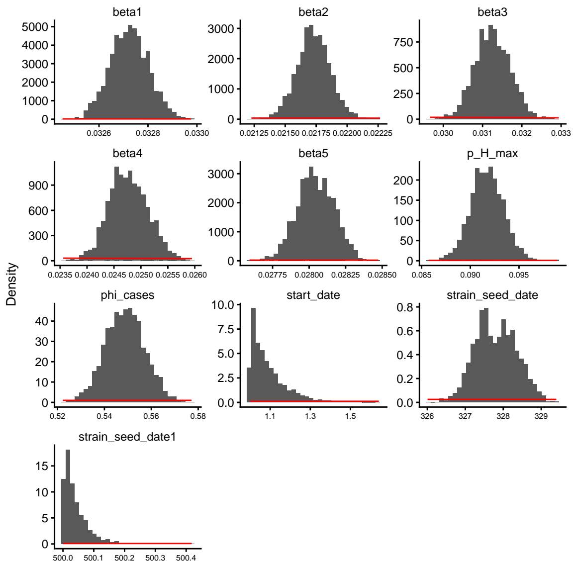
Figure S2: Prior (red lines) and posterior (histograms) distributions of fitted parameters
