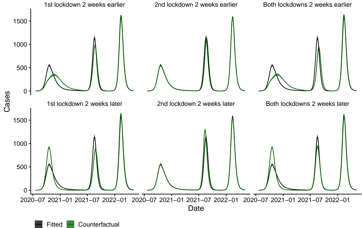
Figure S7: Impact of alternative lockdown scenarios on numbers of COVID-19 symptomatic cases.
