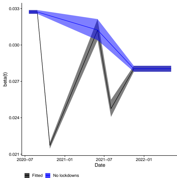
Figure S9: Estimated transmission rate over time, \beta(t) . Black line shows median estimate, shaded region the 95% CI for the fitted model. Blue line and shaded region show the same for the “no lockdowns” counterfactual scenario.
