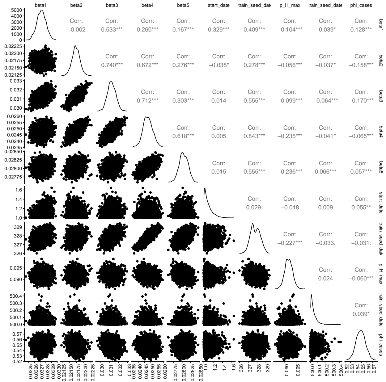
Figure S3: Posterior distributions and pairwise correlations of the fitted parameters. Parameter posterior distributions are shown on the diagonal, pairwise scatter plots in the lower triangle, and pairwise correlation coefficients in the upper triangle.
