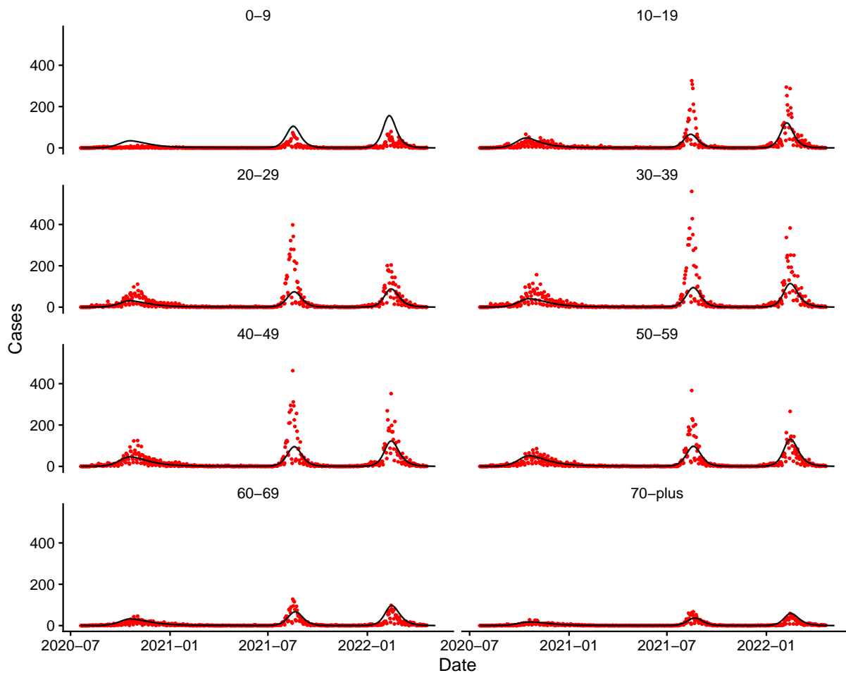
Figure S5: Fit of the model to age-stratified confirmed case data for French Polynesia from July 2020 to May 2022. Red points show data, black line and grey shaded area show median and 95% CI of simulations of the fitted model, i.e. the uncertainty in the expected number of cases in the model. Note that this does not include uncertainty in the reporting process and that there is a strong day-of-the-week effect in the reporting.
