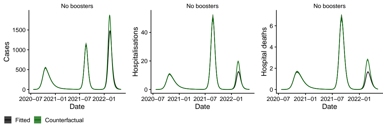
Figure S8: Impact of booster programme on numbers of COVID-19 symptomatic cases, hospitalisations and hospital deaths relative to no boosters for lower booster waning rate from [2]. See blue lines in Figure 2 in main text for comparison with higher booster waning rate from [1].
