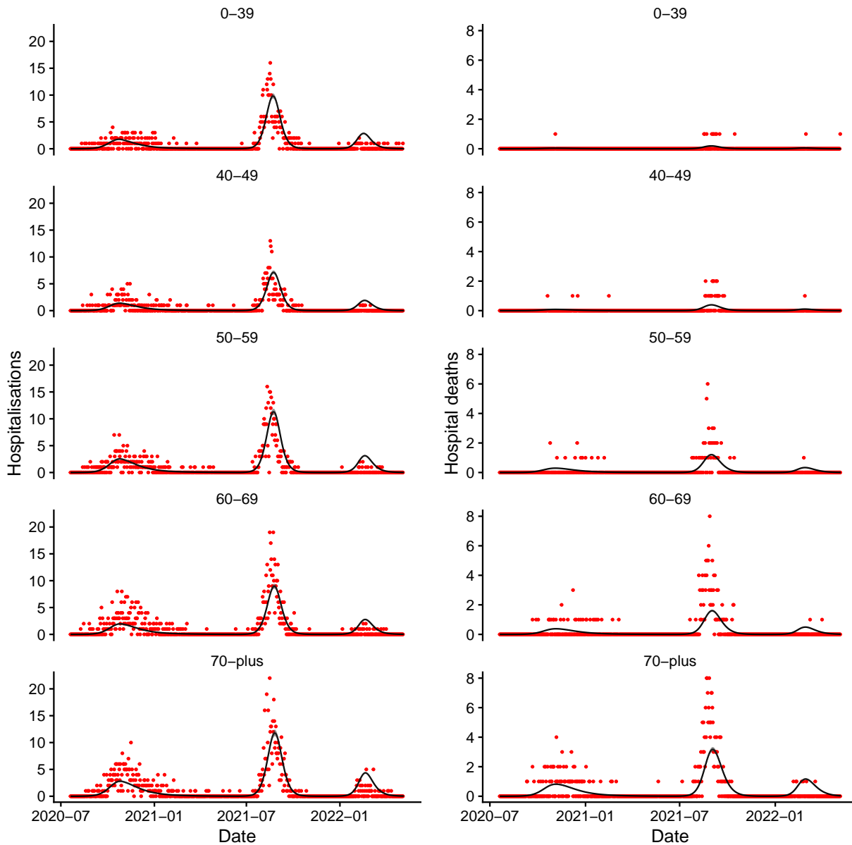
Figure S4: Fit of the model to age-stratified hospitalisation (left) and hospital death (right) data for French Polynesia from July 2020 to May 2022. Red points show data, black line and grey shaded area show median and 95% credible intervals of simulations of the fitted model, i.e. the uncertainty in the expected number of hospitalisations and deaths in the model. Note that this does not include uncertainty in the reporting process. Note different scales on vertical axes.
