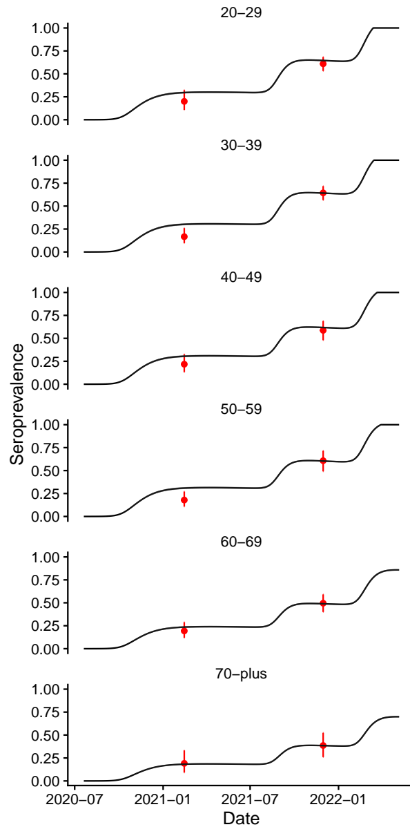
Figure S6: Fit of the model to age-stratified seroprevalence data from the two seroprevalence surveys conducted on Tahiti and Moorea by the Cellule Epi-surveillance COVID and the Health Department of French Polynesia in February 2021, and on Tahiti by Institut Louis Malardé in November-December 2021. Red dots and bars show seroprevalence estimates and exact binomial 95% confidence intervals for the two sero-surveys, and black line and grey shaded region show median and 95% CI of seroprevalence from simulations of the model.
