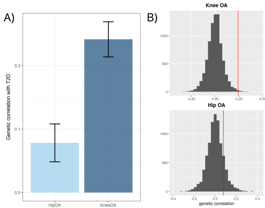
96 97 Figure 1: Stronger evidence for a genetic correlation between type 2 diabetes and knee osteoarthritis compared to hip 98 osteoarthritis. A) Genetic correlation results between type 2 diabetes (T2D) and knee or hip osteoarthritis (OA). B) 99 Permutation-based testing results for knee OA and hip OA, respectively. The red line is the true correlation.
