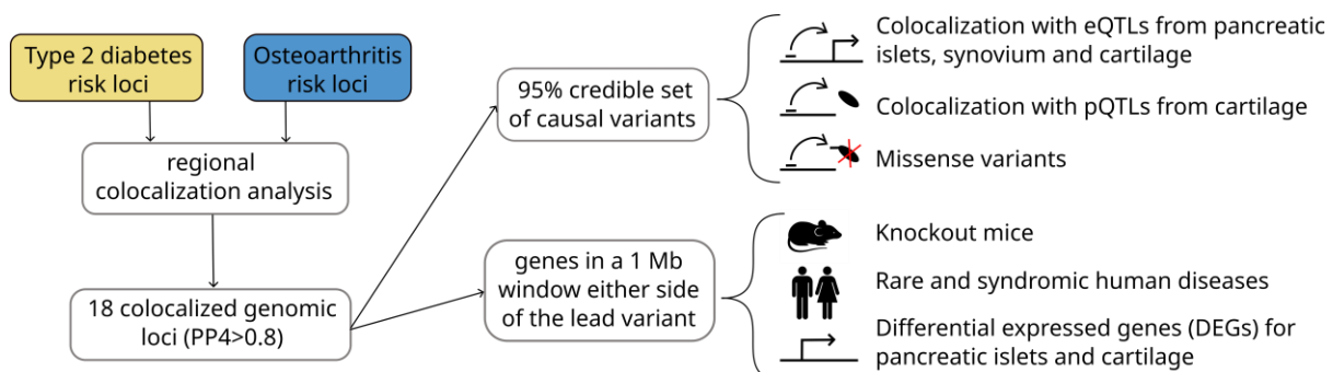
124 Figure 3: Study design. In each of the 18 genomic loci that colocalized with a posterior probability of a single shared causal 125 variant ( PP4 \geq 0.8 ), we explored all genes in a 1Mb window on either side of the lead variants of the 95% credible set for the 126 causal variant of the colocalization analysis. For each gene, we searched databases for knockout mice, and rare and syndromic 127 human diseases for pre-defined type 2 diabetes- and musculoskeletal-related phenotypes. We also examined differentially 128 expressed genes (DEGs) in pancreatic islets of healthy versus diabetes patients, and of degraded versus intact osteoarthritis 129 cartilage. We examined the variants in the 95% credible set for the causal variant of each colocalization locus for missense 130 variants. We performed regional multi-trait colocalization analyses between type 2 diabetes, each osteoarthritis phenotype, 131 and molecular QTL (gene expression and protein QTL) from disease-relevant tissues. We also examined previously curated 132 high-confidence effector genes for type 2 diabetes or osteoarthritis (Methods).
