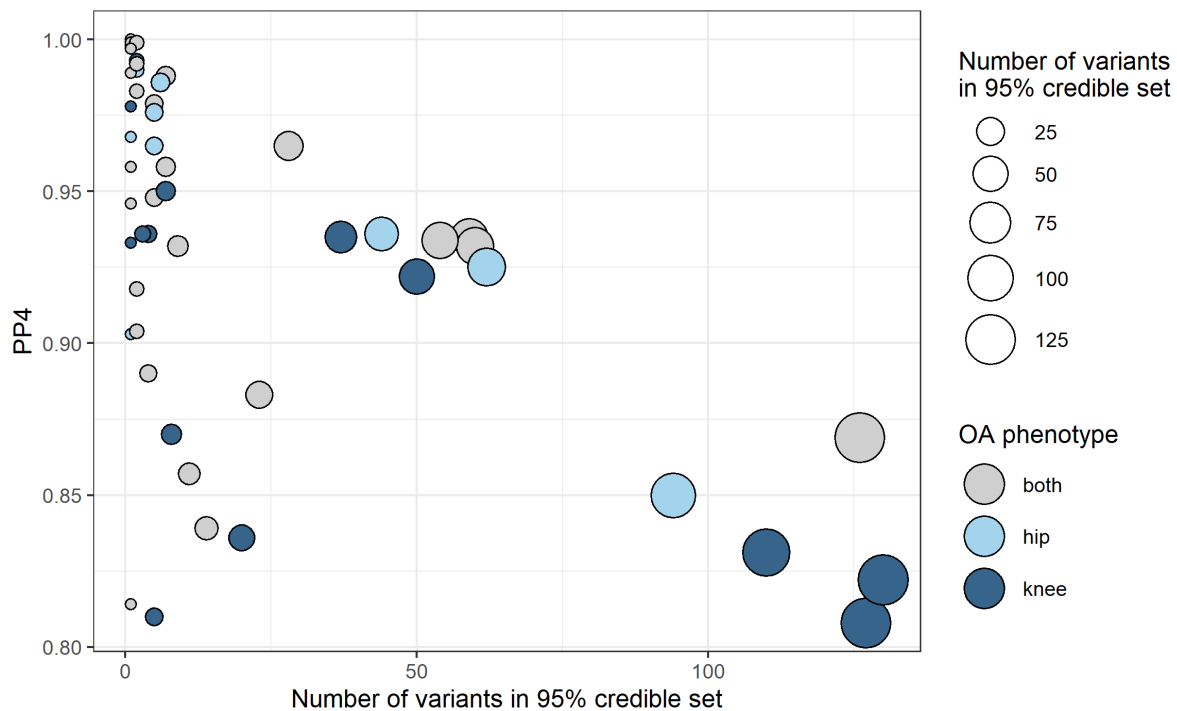
109 Figure 2: Overview of colocalizing regions. The y-axis depicts the posterior probability of a shared causal variant (PP4) and 110 the x-axis the number of variants in the 95% credible set for the causal variant. Each point represents a colocalized signal 111 between type 2 diabetes and one osteoarthritis (OA) phenotype. Point size is proportional to the number of variants in the 112 colocalization analysis 95% credible set. We find strong statistical evidence for colocalization ( PP4 > 0.8 ) at 18 unique genomic 113 loci. Some of those loci colocalize between type 2 diabetes and more than one osteoarthritis phenotype, thus we have 51 114 points.
