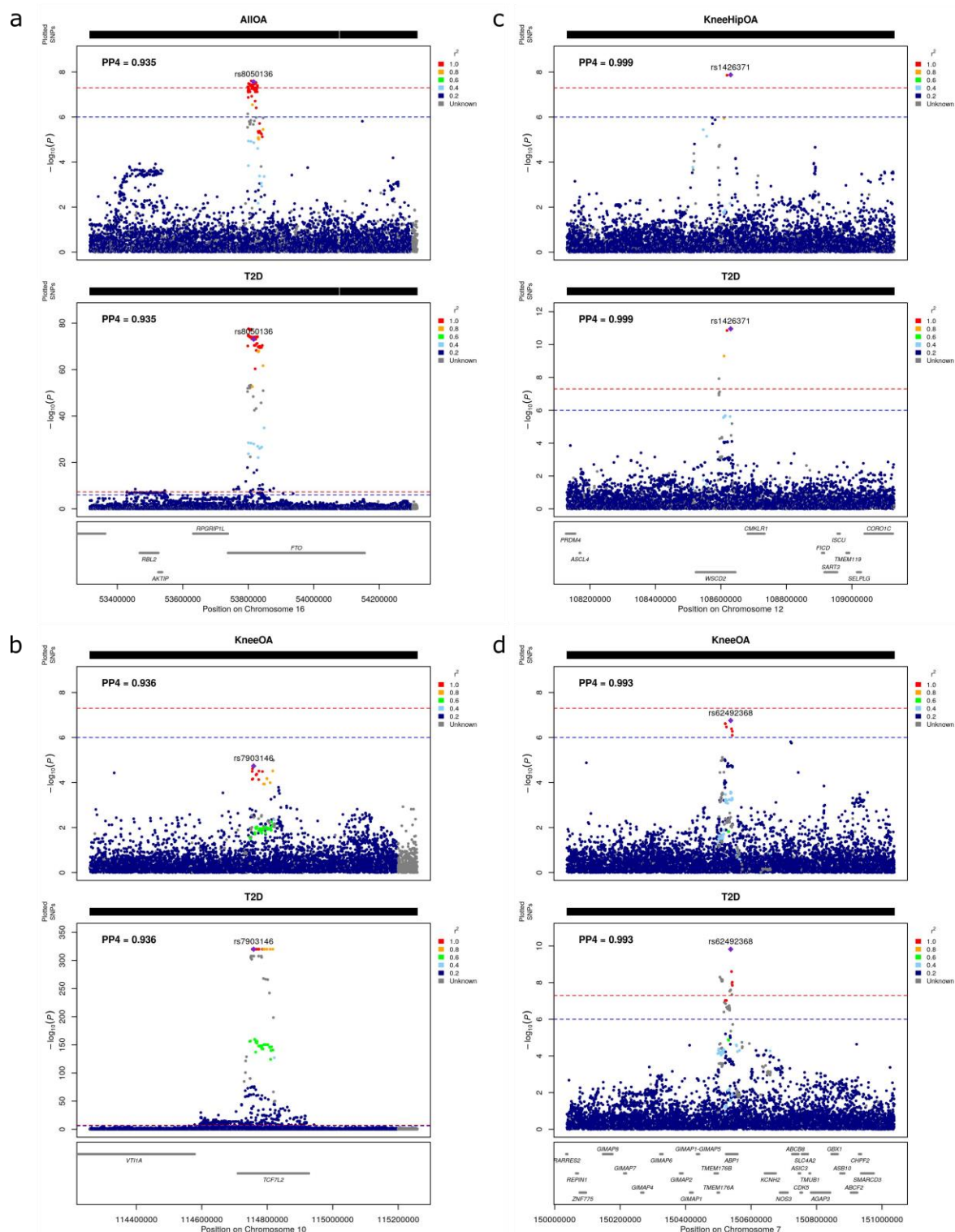
322 323 Figure 5: Regional association plots of the highlighted colocalizing regions between type 2 diabetes and osteoarthritis. a) 324 FTO and IRX3 region; b) TCF7L2 region; c) WSCD2 and TMEM119 region; d) TMEM176A region. The plots are colored based 325 on linkage disequilibrium between the lead causal variant and all other variants. (PP4 = posterior probability of a single 326 shared causal variant; OA = osteoarthritis; T2D = type 2 diabetes; All OA = osteoarthritis at any site)
