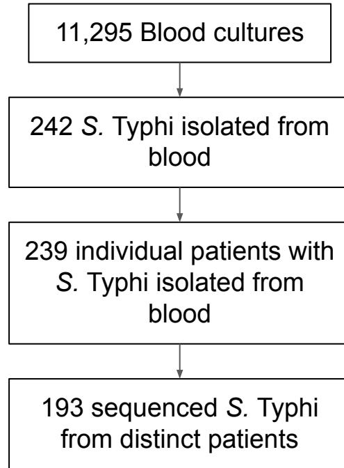
Supplementary Figure 2: STROBE diagram of blood cultures done, S. Typhi isolated and S. Typhi sequenced as part of the STRATAA and TyVAC studies
