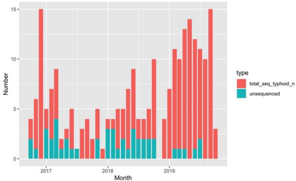
Supplementary Figure 3: The number of patients with sequenced and unsequenced S. Typhi isolates across the recruitment period
