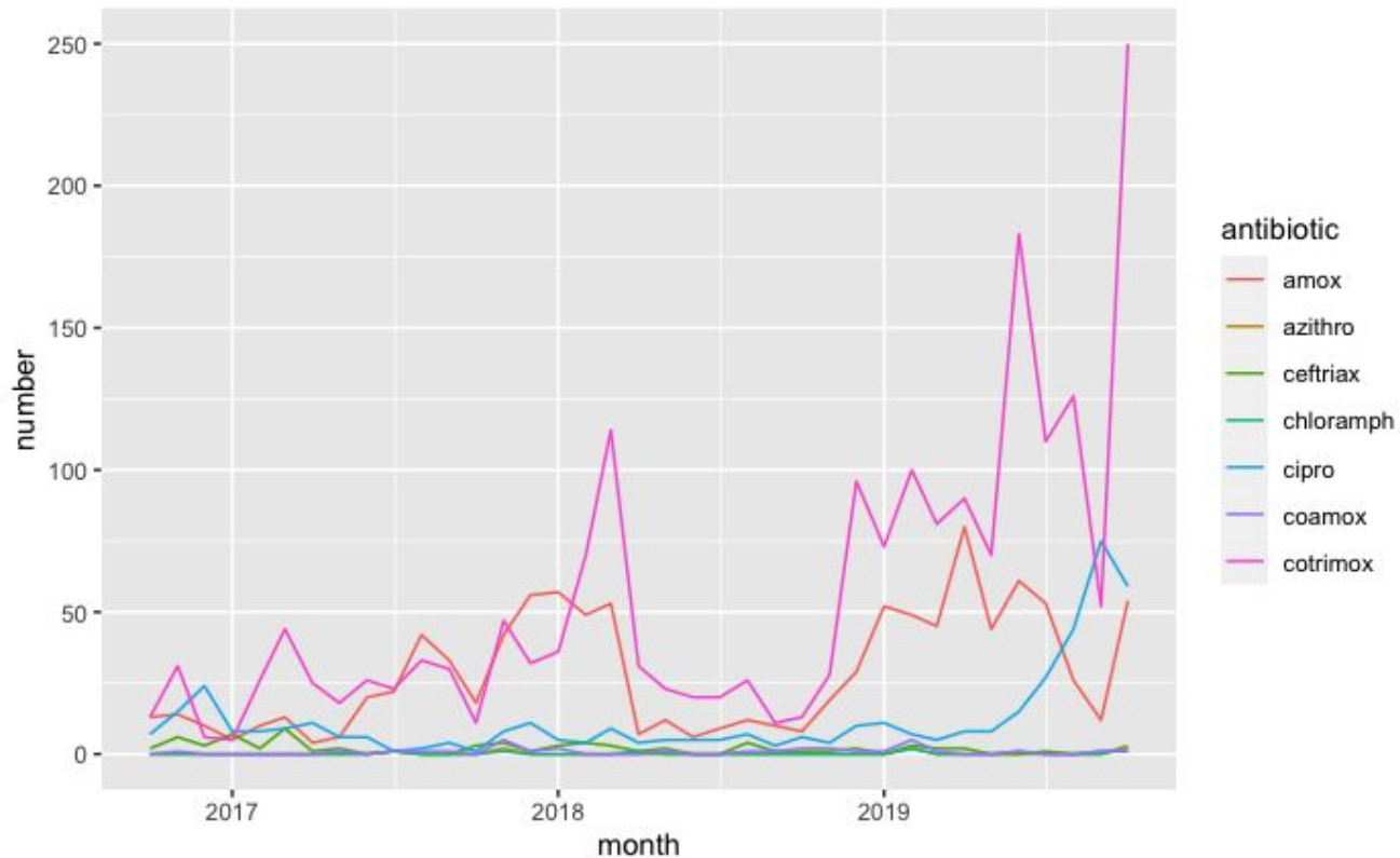
Supplementary Figure 4: Monthly prescriptions of 7 antibiotics to STRATAA participants
