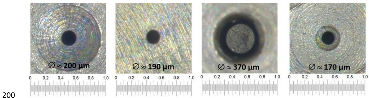
201 Figure 2: Light microscopic images of the outlet orifices with determined orifice diameters of the 202 examined nozzles; scaling in mm.
