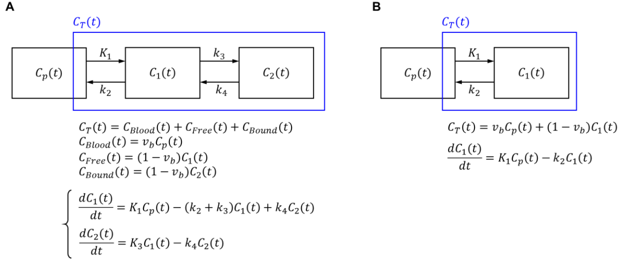
Fig. S21. Definition of conventional one-tissue and two-tissue compartmental models used in PET kinetic modeling. (A) Two-tissue compartmental model with five fitting microparameters (2T5P) of (v_b, K_1, k_2, k_3, k_4) and (B) one-tissue compartmental model with three fitting microparameters (1T3P) of (v_b, K_1, k_2) , in which C_p corresponds to the activity concentration of the tracer in blood plasma (which is approximated by image-derived whole-blood activity concentration in this study), C_T corresponds to the activity concentration of the tracer in tissue, v_b represents the fractional blood volume in tissue, and K_1, k_2, k_3, and k_4 are the rate constants between the model compartments. Two-tissue compartmental model with four fitting microparameters (2T4P) can be defined as a special case of 2T5P model, in which k_4 is zero. K_1 is expressed in mL/min/mL tissue , while k_2, k_3, and k_4 are all expressed in 1/min. The differential equations defining each model are shown below each model. K_1 and k_2 are affected by the blood flow and the permeability of the tracer across the blood capillaries. In a simplified case, the first compartment represents concentrations of the free tracer in tissue and the second compartment represents concentrations of the tracer bound to cell receptors in the tissue. In the case of 1T3P model, the free and bound compartments are not distinguishable from each other. In the specific case of ^{89}\text{Zr} -Df-Creftmirlimab targeting the CD8 receptors, all rate constants include effects from cell trafficking and the concentrations in each compartment also include concentrations of labeled cells trafficking in and out of the tissue.
