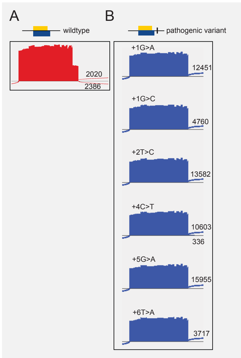
Supplemental Figure 1 Sashimi plot from IGV showing read pileup and splice junction read counts from deep sequencing of RT-PCR products from individual minigene assays of (A) wildtype WT1 exon 9 and flanking introns and (B) six mutant constructs
