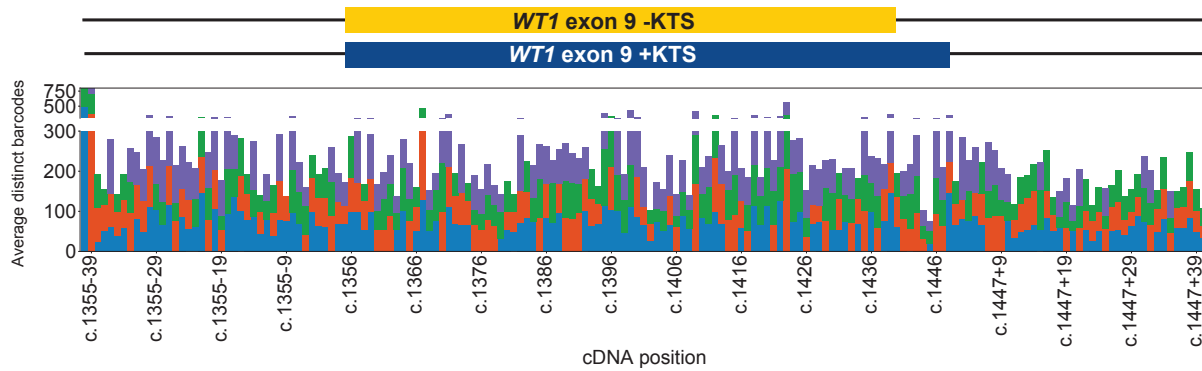
Supplemental Figure 2. Distinct barcode counts for each mutation (mean across replicates) are shown by position. Each shows the three different nucleotide substitutions per position.
