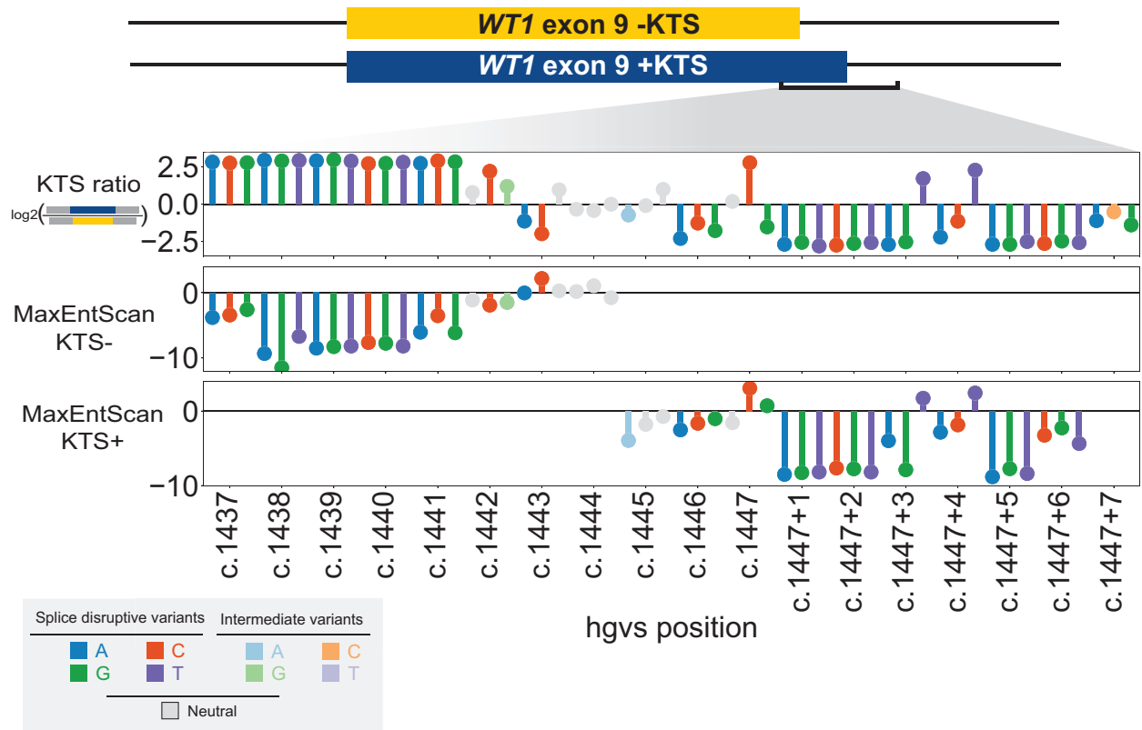
Supplemental Figure 4. MaxEntScan predictions of splice site strength. Measured splicing scores for variants surrounding the two KTS donors (top) and MaxEntScan predictions of splice site strength for the KTS- (middle) and KTS+ donors. Each lollipop represents a single variant plotted by its cDNA position (x-axis), with dark shading for variants altering the KTS ratio, light shading for intermediate ones, and gray for variants with no effect upon the KTS donors. Variants outside of the MaxEntScan scoring range have no associated lollipop.
