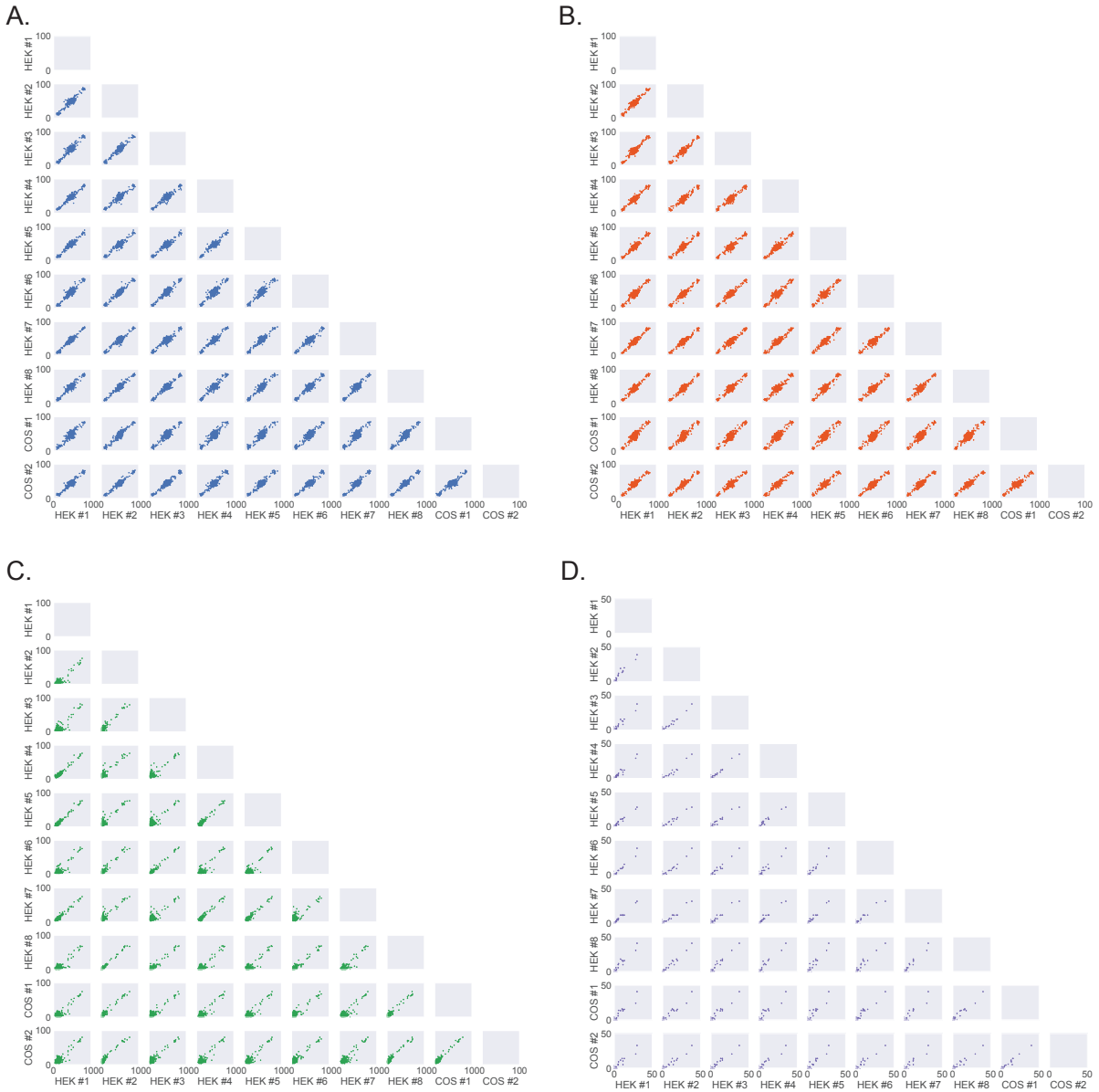
Supplemental Figure 3. Inter-replicate correlations of measured isoform use. A. KTS+ isoform usage for each replicate - different cell-types are indicated. Here, each point represents an individual variant. B. KTS- isoform usage for each replicate. C. SKIP isoform usage for each replicate. D. OTHER isoform usage for each replicate.
