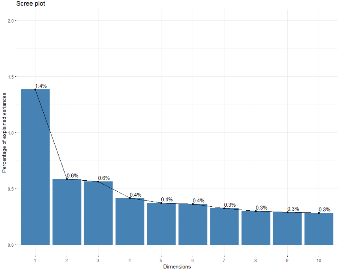
Supplementary figure 3. Scree plot of number of dimensions and percentage of explained variance.
