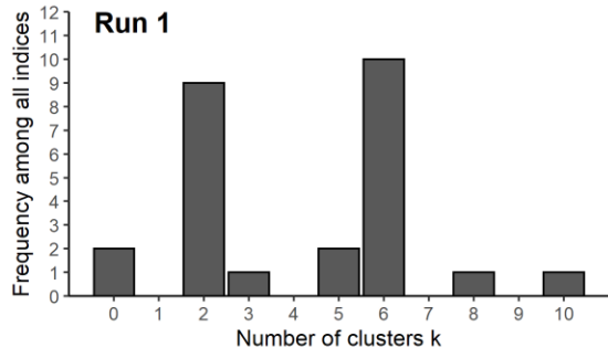
Supplementary figure 4. NBClust package output of five runs. All indices were run except GAP, Gamma, Gplus and Tau.
