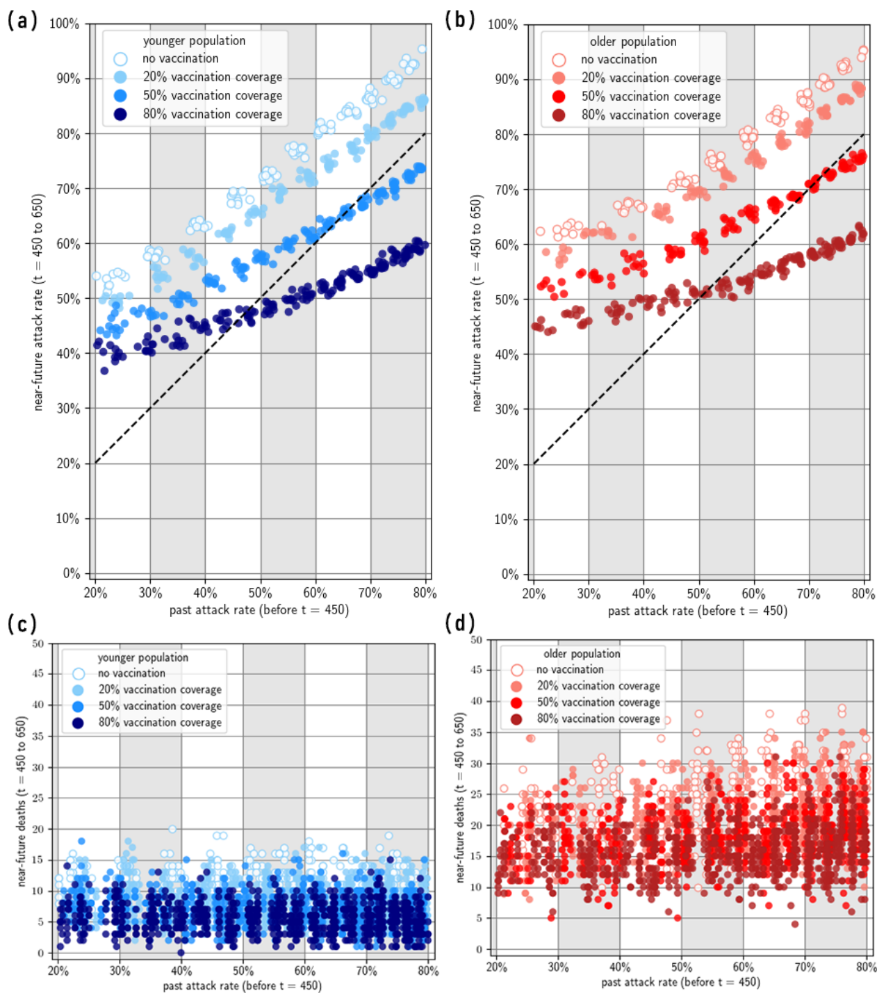
Figure 5: Near-future attack rate and deaths given past immunity, for a second wave due to a BA.4/BA.5-like immune escape variant. The diagonal line represents where past and near-future attack rates are equal. Note that we have only included simulation results in which the past attack rate is between 20% and 80%.
