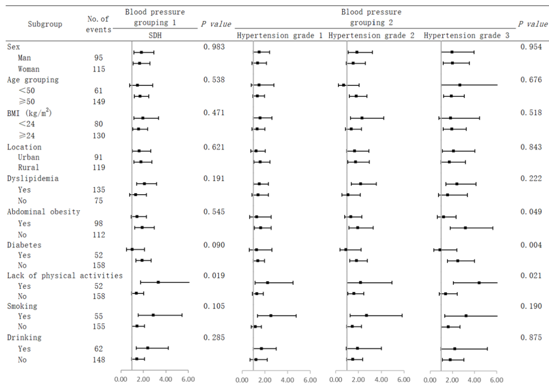
Figure 1 Subgroup analysis of the association between blood pressure and the risk of AMI
