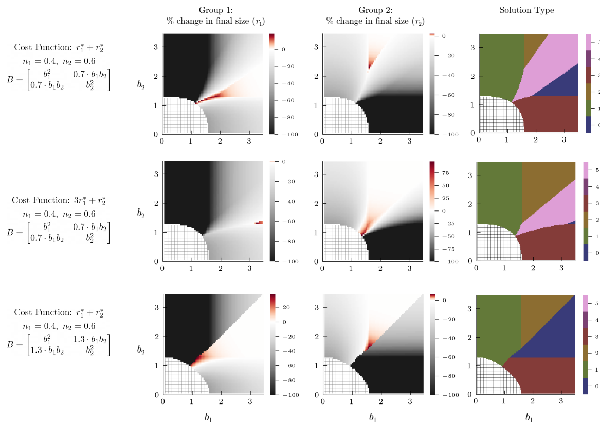
FIG. 4. A section of the parameter and optimal outcome space: The first column of each row shows the cost function, group sizes and the structure of the transmission matrix B . The next two columns are heatmaps which show the percentage change in the attack rate of Group 1 and 2 if the optimal intervention is implemented. The last column shows the type of solution obtained from the optimisation problem – the mathematical expression and description for the solutions can be looked up in TABLE I. The red coloring in the heat-map show regions of the parameter space where the optimal intervention would cause a worse outcome in one of the groups while minimising the cost function for the overall population. The model is identical for the first two rows, but the cost function is different. In the first row the cost function is the attack rate, while in the second row it is a weighted function of the two attack rates. The group sizes are 0.4 and 0.6 for all the rows.
