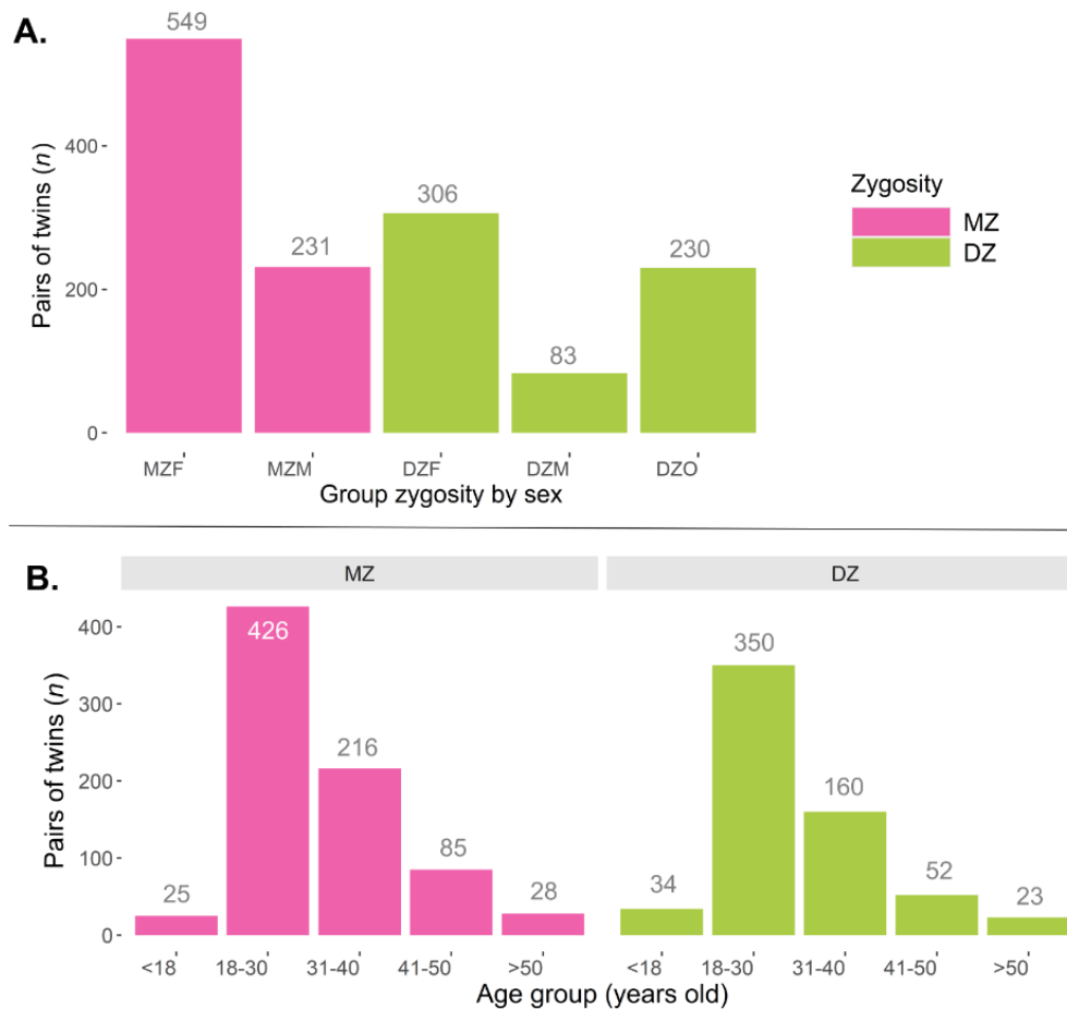
Figure 2.A. Distribution of pairs segregated by zygosity and sex. Sample size by group no differences by group were observed ( p=0.18 ). B. Distribution of pairs segregated by zygosity and age group. No differences between DZ and MZ pairs were observed ( p=0.13 ).
