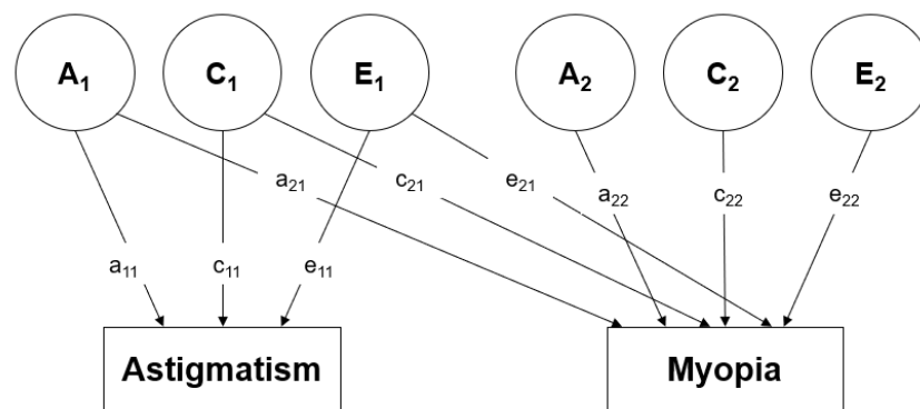
Figure 1. Bivariate path modelling for astigmatism and myopia. Cholesky decomposition in latent variables: A (genetic contribution), C (shared environment influence), and E (residual or non-shared environmental influences). A1 represents the latent variable ( i.e. the set of genes) that contributes to astigmatism (path a_{11} ) and myopia (path a_{21} ). A2 is the second latent variable ( i.e. a second set of genes) affecting myopia. As well as the respective variables for shared and nonshared environmental contributions (C and E).
