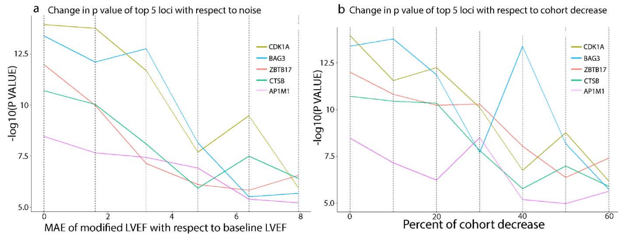
Figure 4 a , Slope chart shows the change in the P value of the top 5 loci with respect to mean absolute error; b , Slope chart shows the change in a P value of top 5 loci with respect to the cohort decrease; each locus is named after the closest gene
