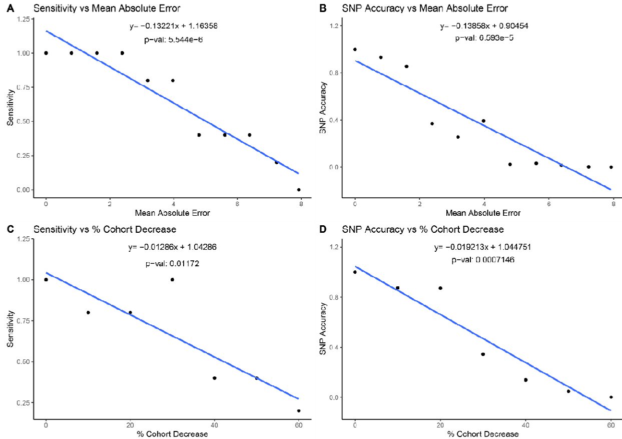
Figure 3 Impact of cohort decrease and noise generation on GWAS power.
