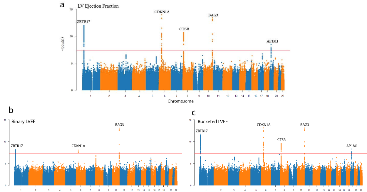
Figure 1 Manhattan plots for genome-wide association studies on UK Biobank reported left ventricular ejection fraction
