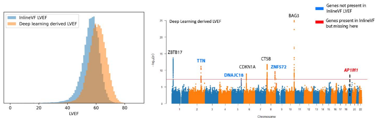
Figure 5 Differences in distribution and GWAS summary statistics between two methods of obtaining LVEF from MRI
