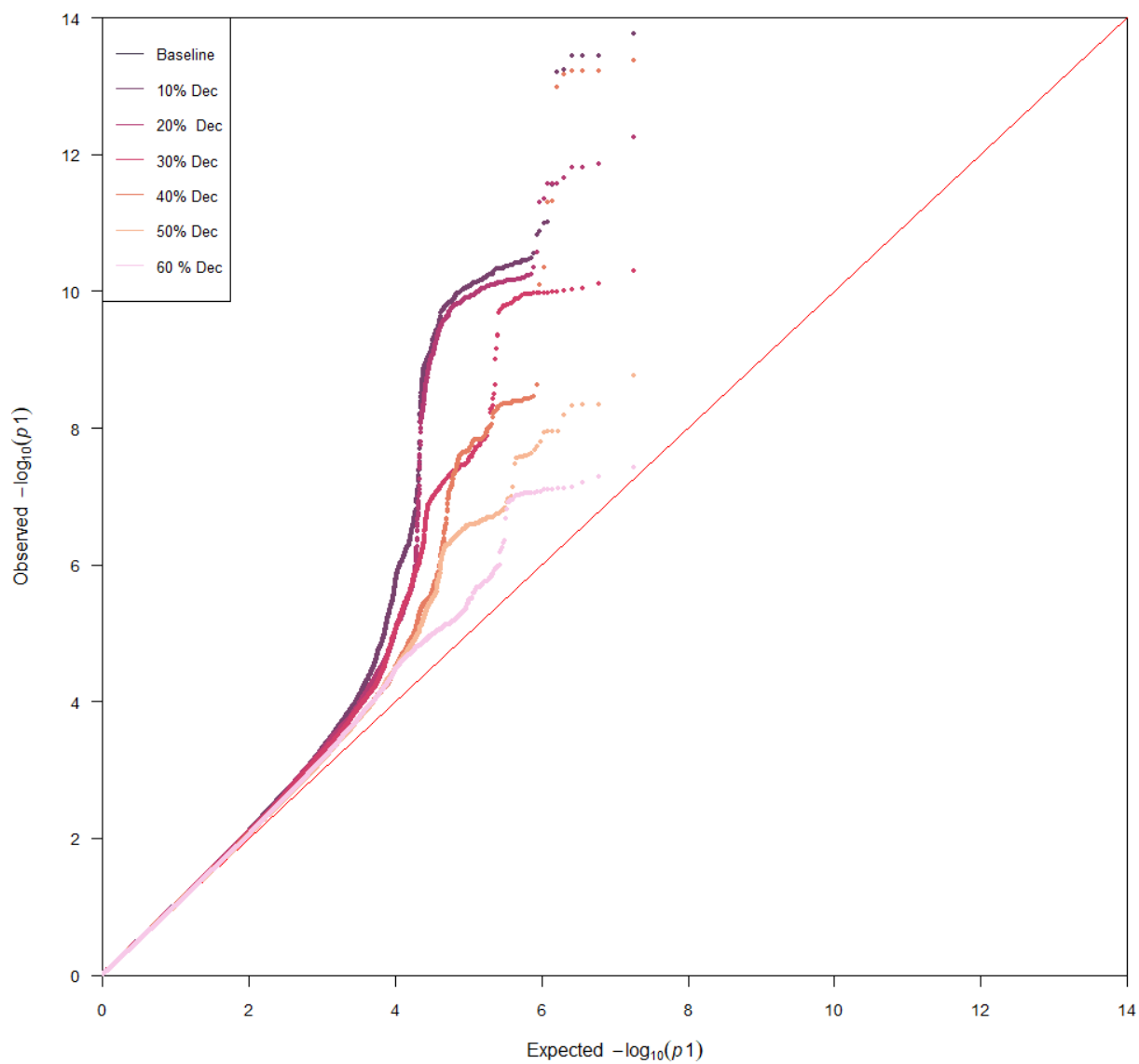
Supplementary Figure 2. Q-Q plots of P values from GWAS summary statistics for different percentages of cohort decrease
