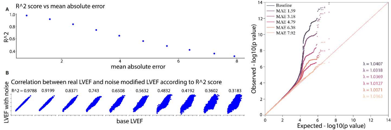
Figure 2 Impact of noise in LVEF on GWAS
