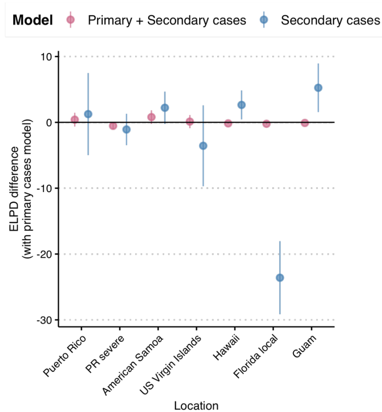
465 Figure 3. Leave-one-out cross validation model comparison using the 466 estimated difference in ELPD (expected log pointwise predictive probabilities).
