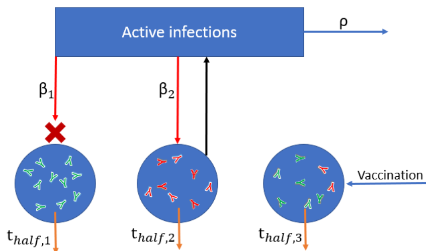
Figure 1: Schematic of simplified agent-based model used to simulate probabilities of infection and adverse outcomes based on nAb titers. The model simulates exposures (red arrows) according to individual contact rates ( \beta_1 , \beta_2 ) and the force of infection (active infections multiplied by R_0 ). Exposure succeeds or fails to induce infection probabilistically according to the level of protection afforded by an individual's combined infection and vaccine nAb titer. nAbs decay over time according to each individual's half-life ( t_{half} ), and nAb boosting occurs through vaccination (green antibodies) and infection (red antibodies). The number of active infections is tracked, increasing by one for each successful infection and decaying according to the recovery rate ( \rho ).
