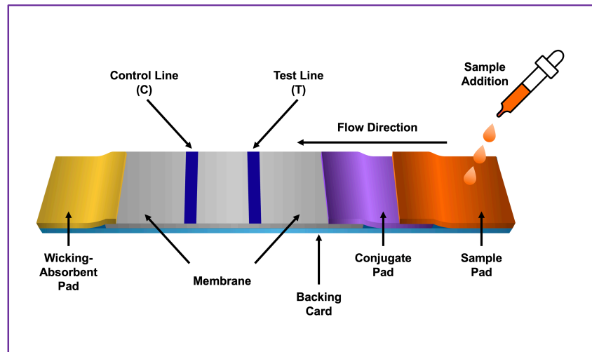
Figure 1. Schematic representation of a typical configuration of a lateral flow immunoassay test platform or strip. There are five key design components forming the platform: sample pad, conjugate pad, membrane with immobilized antibodies, and an absorbent pad. The components of the strip are usually fixed to an inert material backing card, housing, and protecting the test strip.
