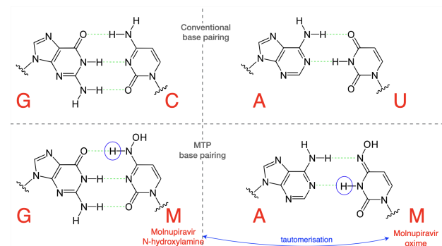
Figure 1. Molnupiravir triphosphate can assume multiple tautomeric forms. The N-hydroxylamine form resembles cytosine, while the oxime form more closely resembles uracil. They therefore pair with guanine and adenine respectively. (Figure adapted in part from Malone and Campbell (2021).)
