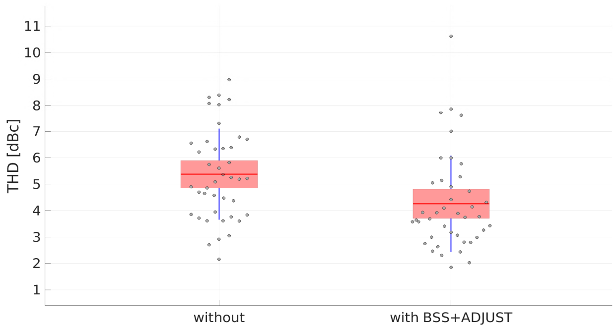
Fig S 10: Total-Harmonic Distortion (THD) analysis reporting the values in y-axis as the THD trial-values in dBc and in the x-axis we described the measures of the THD after filtering (1) without using Artifact Subspace Reconstruction (ASR) and ADJUST, and (2) using the Blind-Source Separation (BSS) method ASR and ADJUST for artifact-removal. THD difference between modalities is significant - F(1,445)=13.35 , p=0.0278 . The points in grey show the outlier values on each modality. For calculating the THD values in dBs we used the method described in [4].
