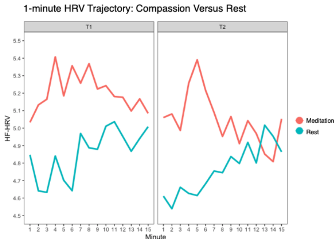
Figure 5. Average HRV signal-change across 1-minute bins, ordered for T1 and T2, at CFT Meditation and Rest. Note the overall between Meditation and Rest at both timepoints, whereas the average HRV recording at 1-minute intervals were greater for the compassion condition (Red Lines) versus the baseline Resting state (Blue Lines). Note that at T2 (right panel), the HRV recording during CFT was shown to decrease during the threat component of the exercise.
