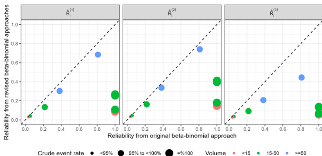
Figure 2: Reliability estimates from the original and revised beta-binomial approaches (line of identity dashed).
