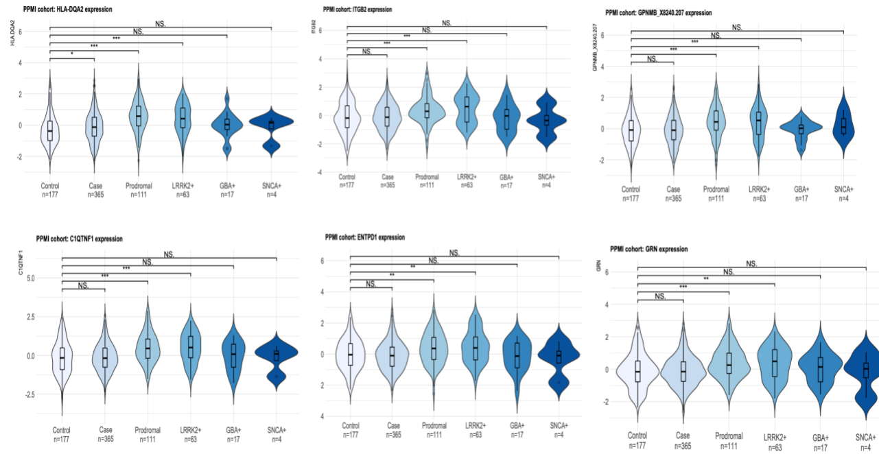
Supplementary Figure 3: PPMI significant PWAS Violin plots. Plot of HLA-DQA2 , C1QTNF1 , ITGB2 , ENTPD1 , GPNMB , & GRN gene expression. Control Vs. PD case and mutation carriers ( LRRK2 + , GBA + , and SNCA + ) (light to dark blue). The significance level as stars with p-value equal to or less than 0.001 (***), 0.01 (**), and 0.05 (*).
