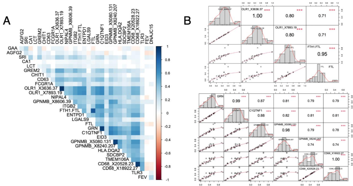
Supplementary Figure 2: Protein-protein correlation. (A) Pearson correlation coefficient matrix of the 26 proteins. (B) Chart correlation of the significant regions of OLR1 and FTL analytes above and GRN below. The distribution of each protein is shown on the diagonal with the bottom displaying the bivariate scatterplots with a fitted line. The top of the diagonal shows the correlation value and the significance level as stars with p-value equal to or less than 0.001 (***), 0.01 (**), and 0.05 (*).
