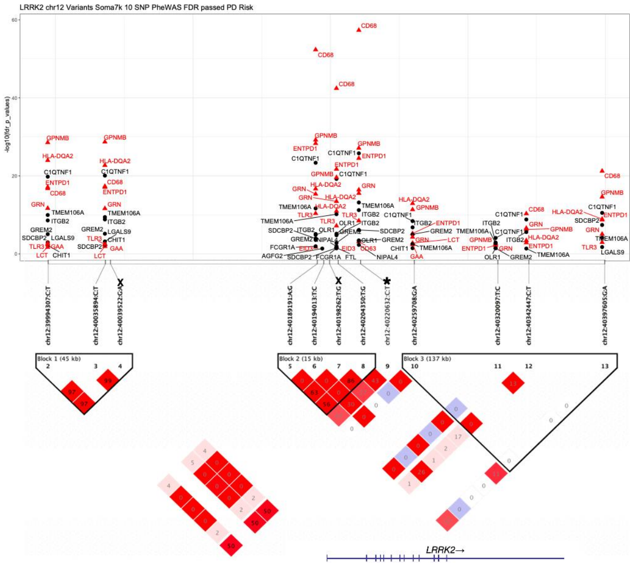
Supplementary Figure 1: PheWAS and LD matrix of LRRK2 variants. PheWAS plot of 10 SNPs in chr12 LRRK2 . FDR corrected -\log_{10}(\text{p-value}) y-axis. 26 unique CSF proteins pass FDR with 11 having known PD risk association (red triangles). LD plot of 12 independently associated Chr12 SNPS, 10 are present with chr12:40220632:C:T (*) and r^2 > 0.85 per LD block removed (X). The 5 independently associated SNPs within the LRRK2 region (Chr12:40,196,744-40,369,285) is below the LD plot with a blue line.
