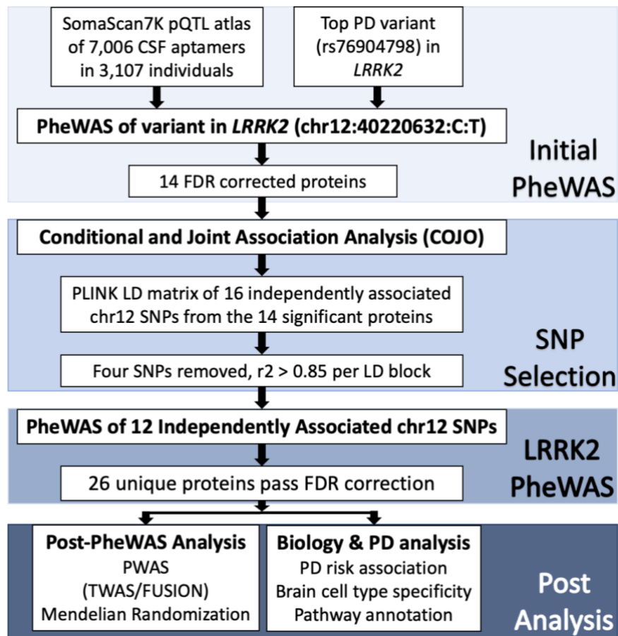
Figure 1 Workflow and study design. The workflow of the LRRK2 loci associated protein analysis with initial PheWAS, SNP selection, LRRK2 PheWAS, fine mapping of significant aptamers, and analysis of proteins in terms of biological and PD significance.
