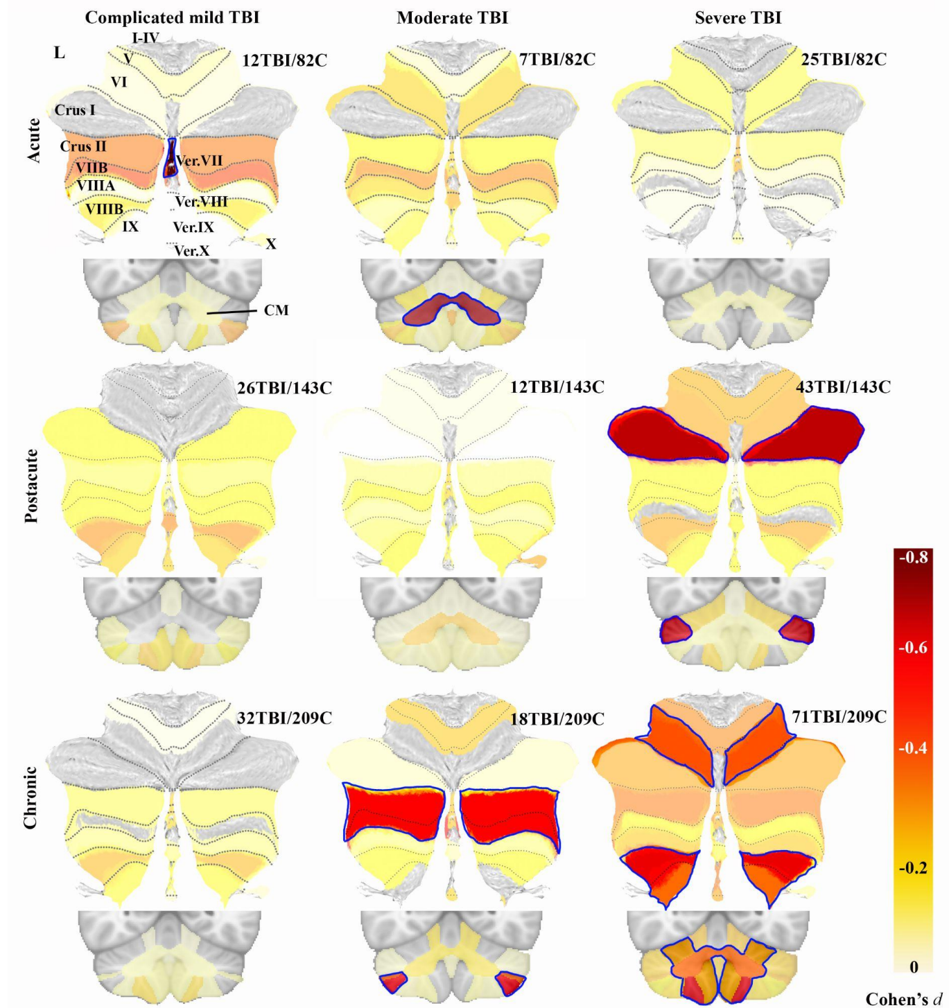
Figure 3. Severity and chronicity analyses. Atlas-based effect size (Cohen's d ) maps and MNI-based coronal slices are shown for group comparisons separated by severity (columns) and chronicity (rows). Lobules and vermal regions (Ver.VII-X) are labeled in the top left on the SUIT flatmap. The corpus medullare (CM) is shown in the coronal slices. The color corresponds to the effect size, according to the colorbar, with dark red for the largest effect sizes. Non-significant effect sizes are shown at 50% opacity, while significant ones are not opaque and outlined in blue. The number of mTBI and non-TBI participants (C) are shown for each comparison. No participant was included twice in any of the nine sub-analyses, but non-TBI participants were included across multiple comparisons. Only negative effect sizes are shown, positive effect sizes were not significant and are not included.
