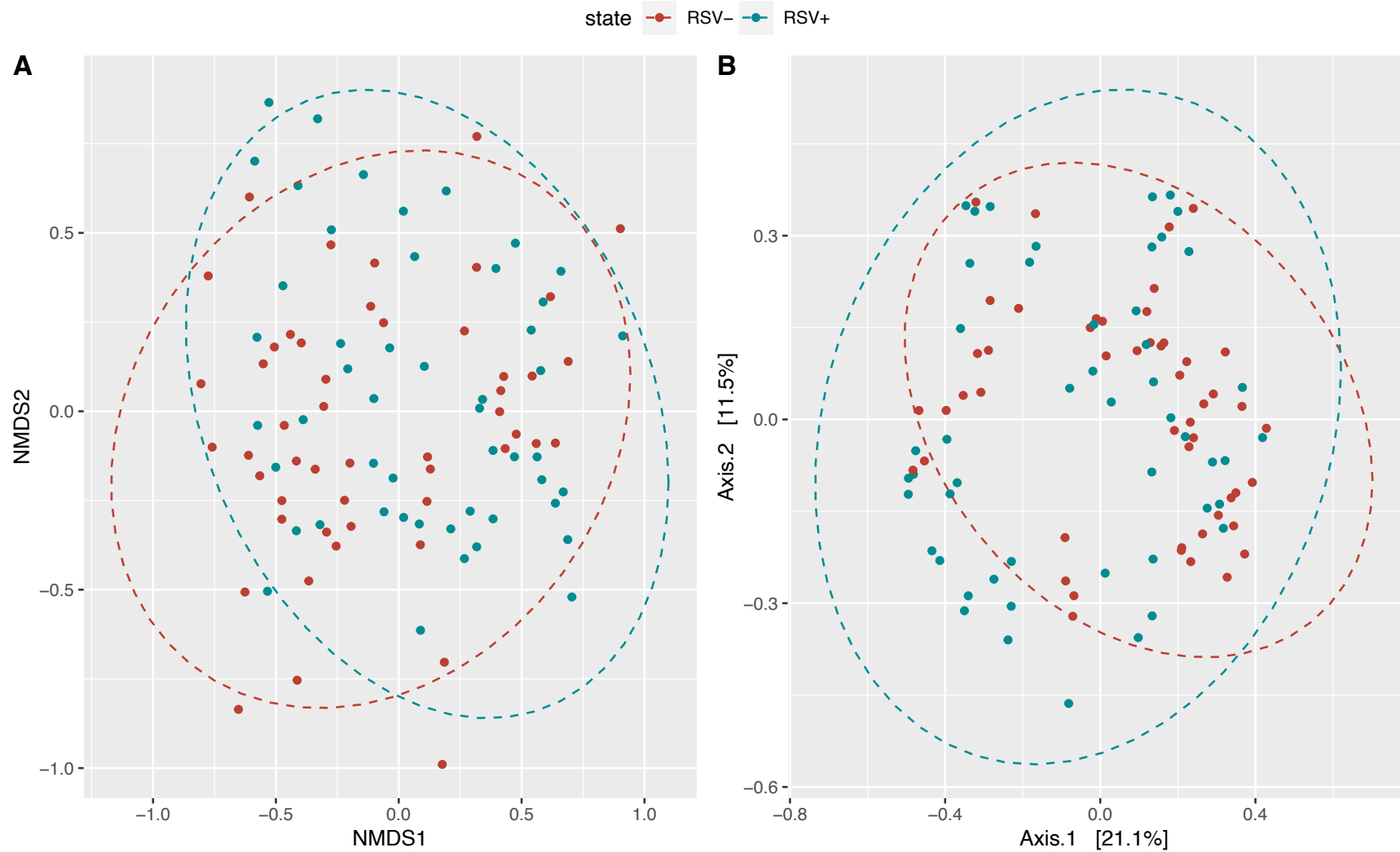
Figure, Supplemental Digital Content 3 Species analyses displaying the Bray Curtis dissimilarity index between RSV+ and RSV- infants. A) NMDS overlap between RSV+ and RSV- samples with a stress value of 0.262 showing very little distinct clustering. B) PCoA indicating some unique clustering of RSV+ in bottom left-hand corner.
